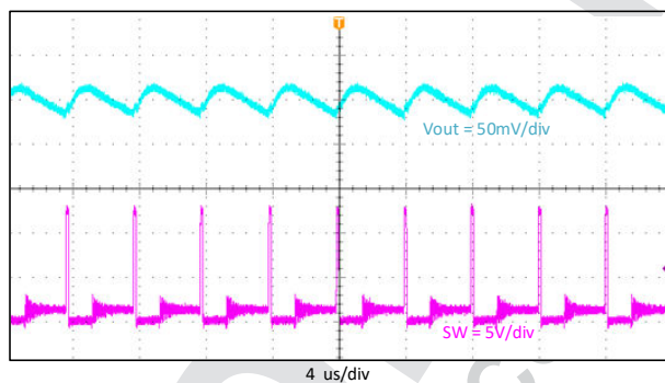
☒ 9-6. Output Voltage Ripple, I_{out} = 0.3\text{ A}
