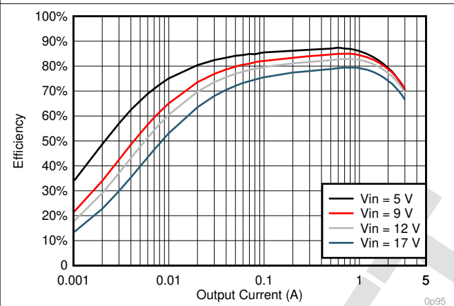
7-9. V_{OUT} = 0.95\text{ V} Efficiency, L = 1.2\ \mu\text{H}
