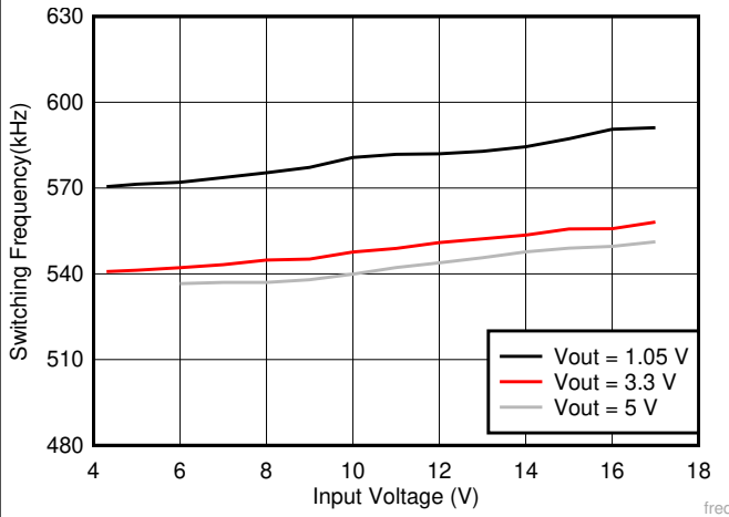
7-7. Switching Frequency vs Input Voltage
