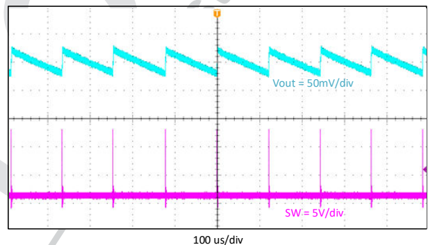
☒ 9-5. Output Voltage Ripple, 10 mA
