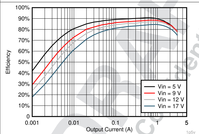
7-11. V_{OUT} = 1.5\text{ V} Efficiency, L = 1.5\ \mu\text{H}
