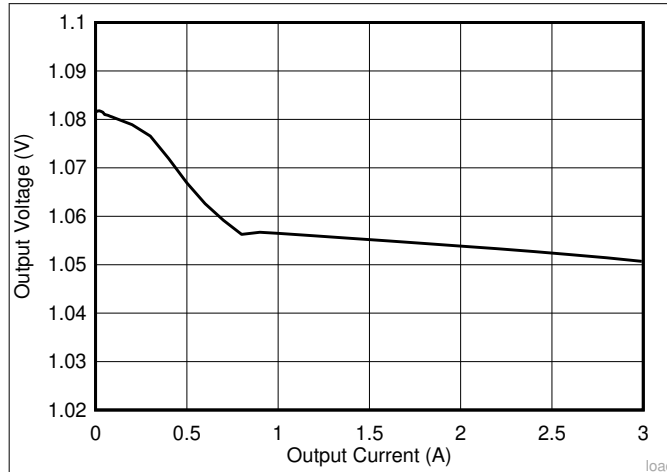
☒ 9-2. Load Regulation with Different Loading
