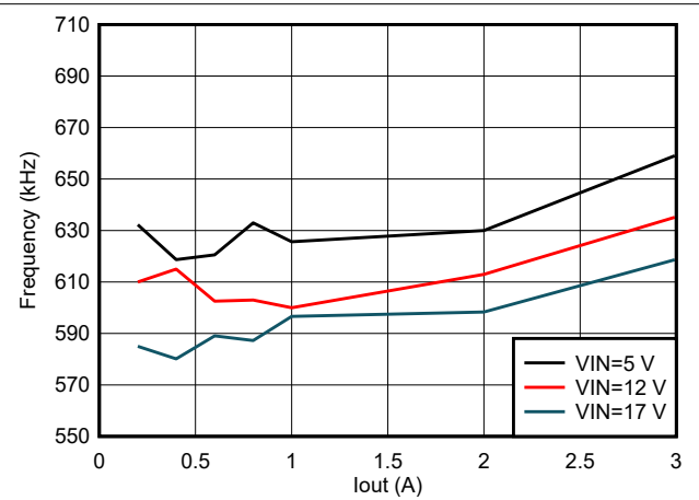
7-3. TPS563206 Frequency vs Loading
