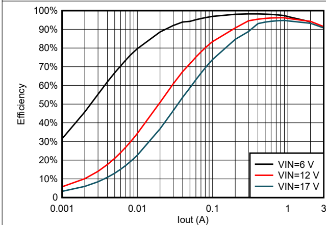
5-17. TPS563206 Efficiency at 5 Vout With 4.7uH Inductor
