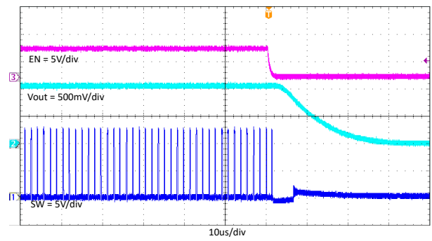
7-13. TPS563203 Enable off With 3A Loading
