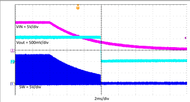
7-17. TPS563203 Power off With 3A Loading
