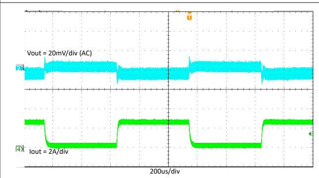
7-21. TPS563206 Load Transient With 0.3A to 2.7A
