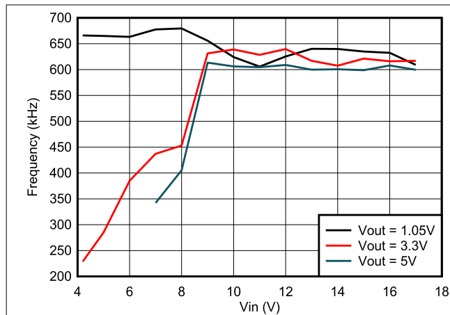
5-7. Frequency vs Input Voltage at 3A Loading
