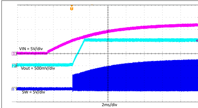
7-16. TPS563203 Power on With 3A Loading
