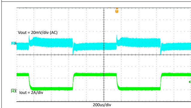
7-20. TPS563203 Load Transient With 0.3A to 2.7A
