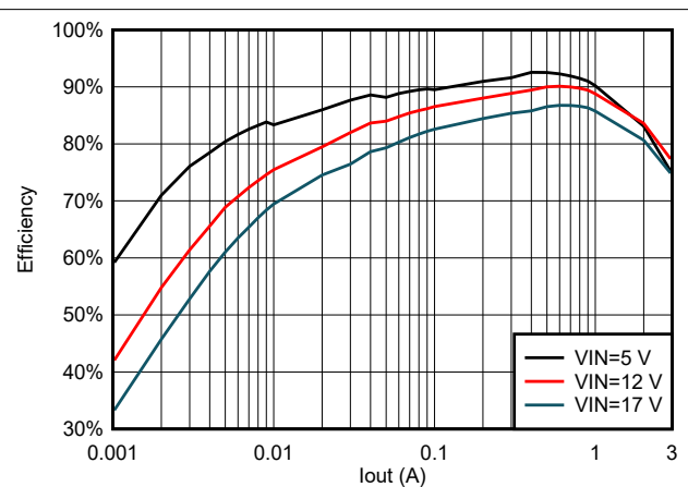
5-12. TPS563203 Efficiency at 1.05 Vout With 2.2uH Inductor
