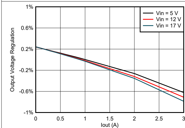
7-4. TPS563203 Load Regulation vs Loading
