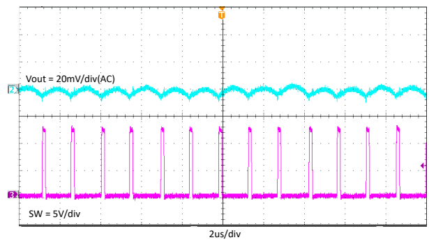
7-11. TPS563206 Output Voltage Ripple With 3A Loading
