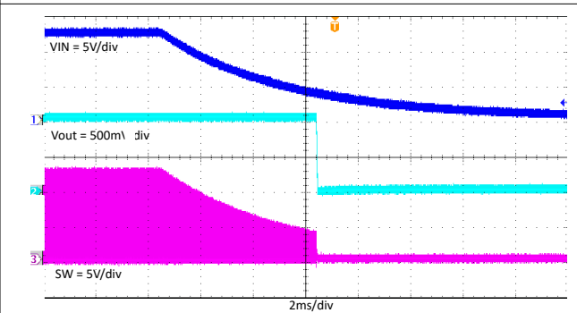
7-19. TPS563206 Power off With 3A Loading
