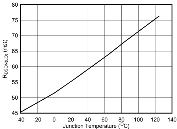
图 5-5. Low-Side R_{dson}
