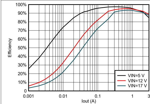
5-15. TPS563206 Efficiency at 3.3 Vout With 4.7uH Inductor
