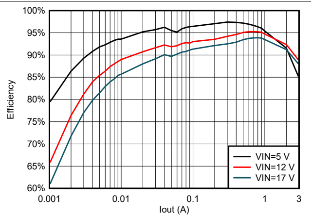
5-14. TPS563203 Efficiency at 3.3 Vout With 4.7uH Inductor
