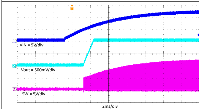
7-18. TPS563206 Power on With 3A Loading
