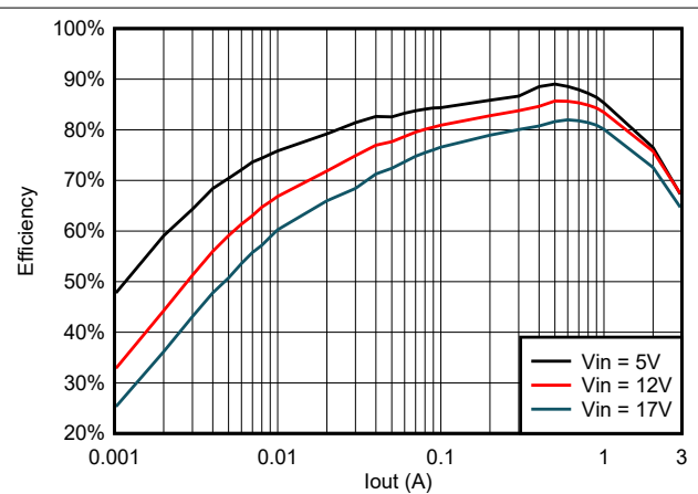
5-10. TPS563203 Efficiency at 0.6 Vout With 1.5uH Inductor
