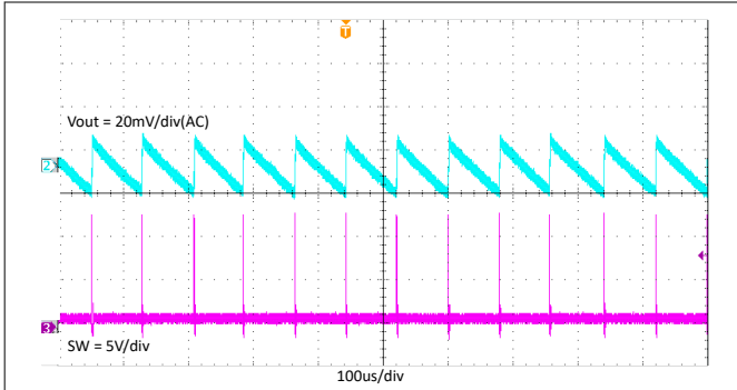
7-8. TPS563203 Output Voltage Ripple With 0.1A Loading
