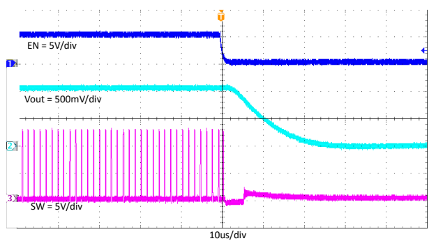
7-15. TPS563206 Enable off With 3A Loading
