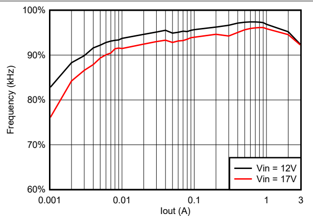
5-18. TPS563203 Efficiency at 7 Vout With 6.8uH Inductor
