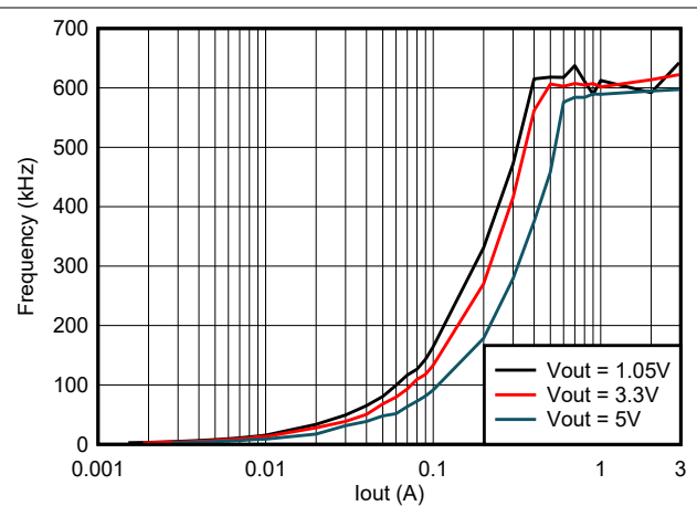
5-8. TPS563203 Frequency vs Loading
