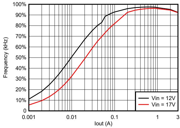
图 5-19. TPS563206 Efficiency at 7 Vout With 6.8uH Inductor
