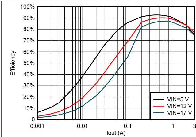
5-13. TPS563206 Efficiency at 1.05 Vout With 2.2uH Inductor
