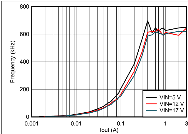
7-2. TPS563203 Frequency vs Loading
