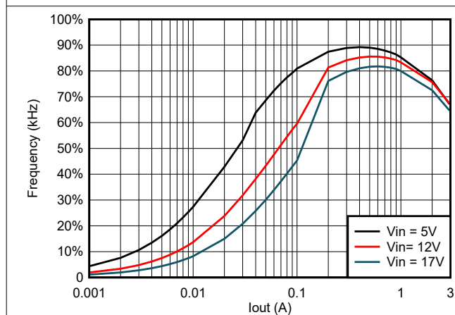
5-11. TPS563206 Efficiency at 0.6 Vout With 1.5uH Inductor
