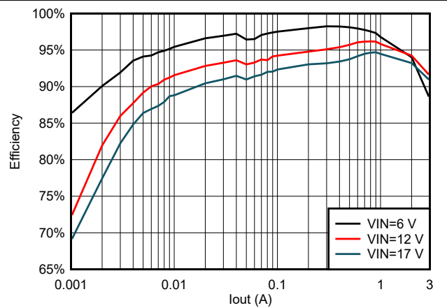
5-16. TPS563203 Efficiency at 5 Vout With 4.7uH Inductor
