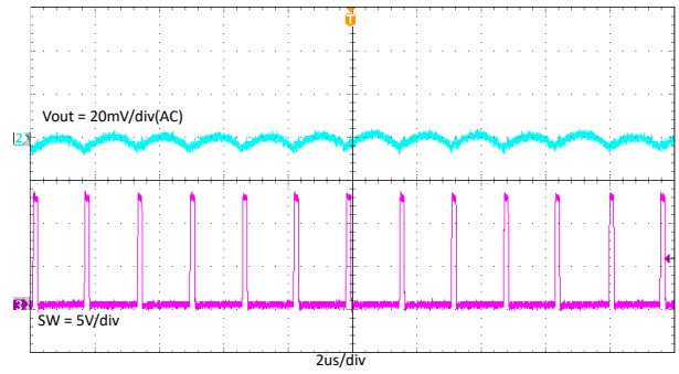
7-9. TPS563206 Output Voltage Ripple With 0.1A Loading
