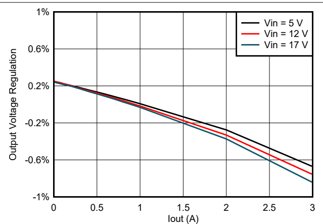
7-5. TPS563206 Load Regulation vs Loading
