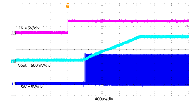
7-12. TPS563203 Enable on With 3A Loading
