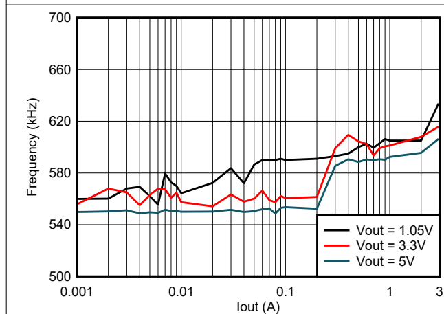
5-9. TPS563206 Frequency vs Loading
