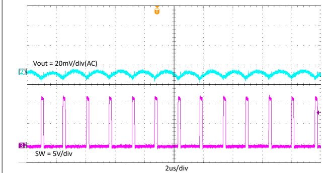
7-10. TPS563203 Output Voltage Ripple With 3A Loading
