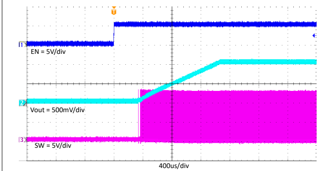
7-14. TPS563206 Enable on With 3A Loading
