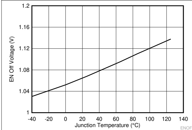
7-3. EN Pin EN Off Voltage vs Junction Temperature
