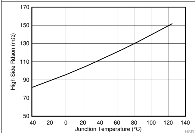
7-5. High-Side R_{ds-On} vs Junction Temperature
