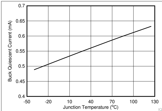
7-1. Supply Current vs Junction Temperature
