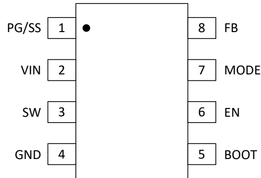
图 5-1. 8-Pin SOT583 DRL Package (Top View)
