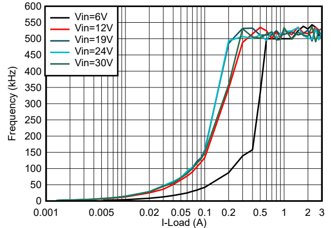
8-5. Switching Frequency vs Load Current
