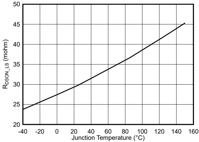
6-3. Low-Side R_{DS(on)} vs Junction Temperature
