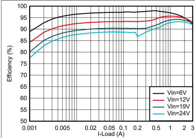
8-2. Efficiency
