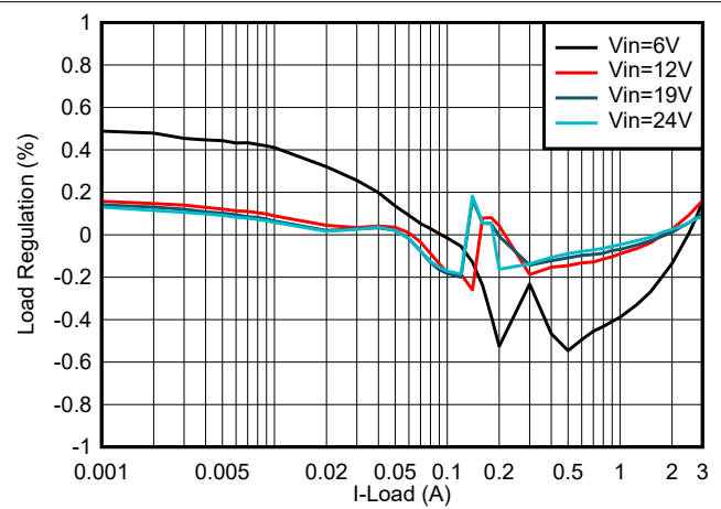
8-3. Load Regulation
