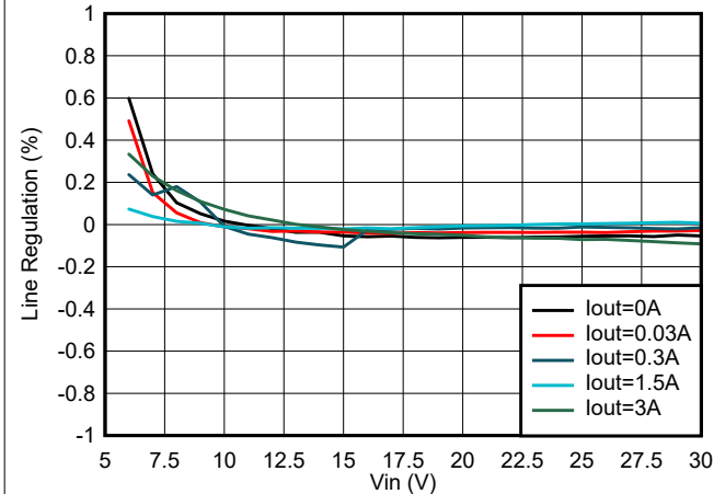
8-4. Line Regulation
