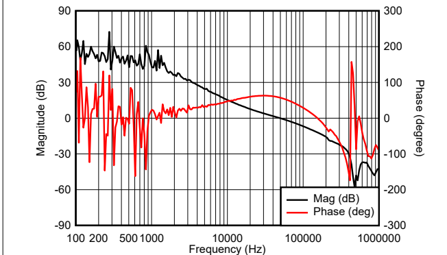
8-6. Loop Frequency Response, I_{OUT} = 3\text{ A} , BW = 49.4 kHz, PM = 57°, GM = -12 dB
