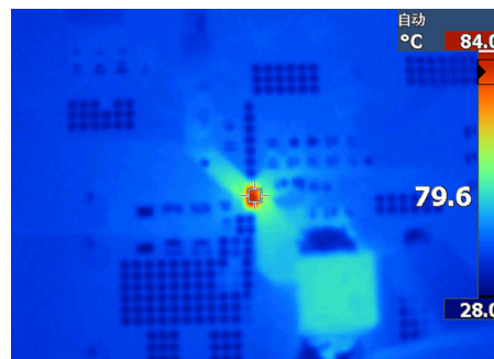
8-7. Case Temperature, V_{IN} = 24\text{ V} , I_{OUT} = 3\text{ A} , f_{sw} = 500\text{ kHz}
