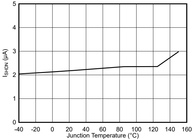
6-1. Shutdown Current vs Junction Temperature
