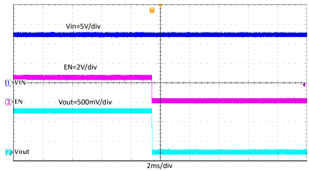
8-19. Shutdown Through EN, I OUT = 4 A
