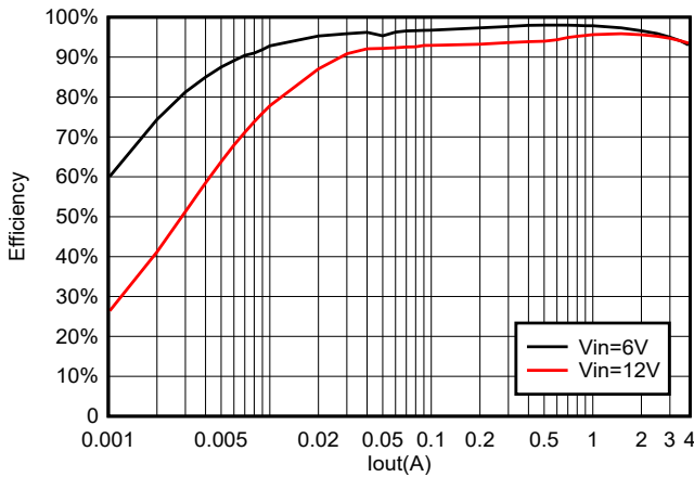
6-21. TPS564255 Efficiency at 5 V_{OUT} with a 4.7- \mu\text{H} Inductor
