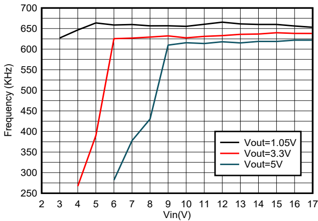
6-9. Frequency vs Input Voltage, I_{OUT} = 4\text{ A}
