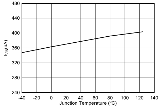
6-2. TPS564257 Quiescent Current
