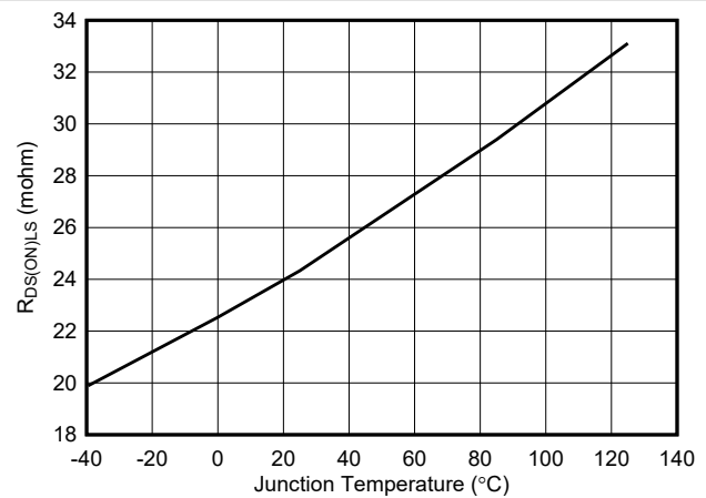
6-6. Low-Side R_{DS(ON)}
