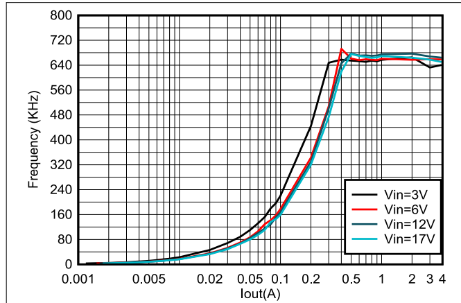
8-2. TPS564252 Frequency vs Loading
