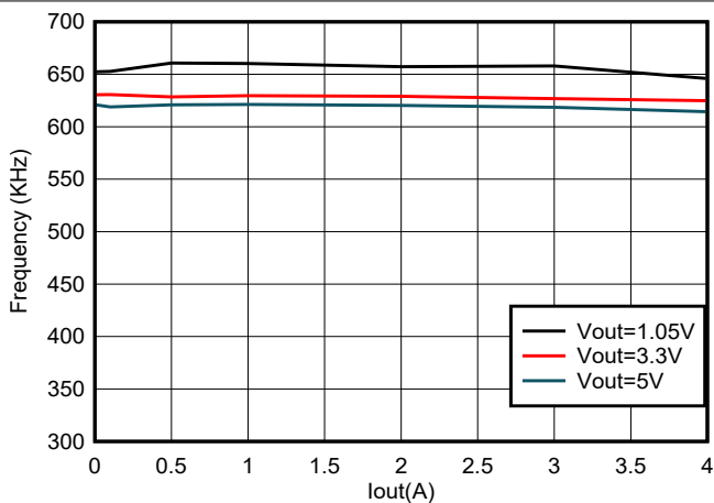
6-11. TPS564257 Frequency vs Loading, V_{IN} = 12\text{ V}
