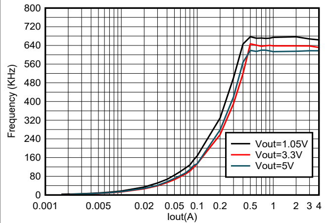
6-10. TPS564252 Frequency vs Loading, V_{IN} = 12\text{ V}
