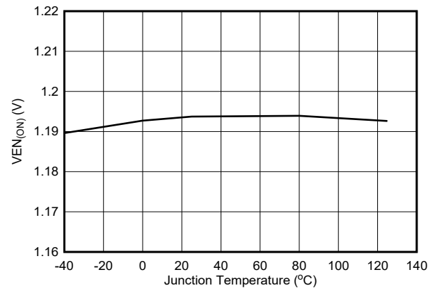
6-4. Enable On Threshold Voltage
