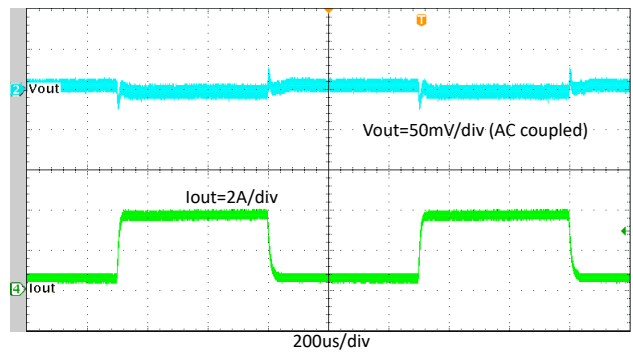
8-17. TPS564255 Transient Response with 0.4 A to 3.6 A
