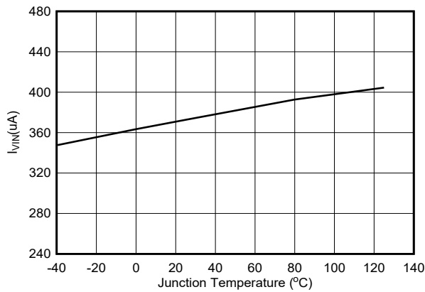
6-3. TPS564255 Quiescent Current
