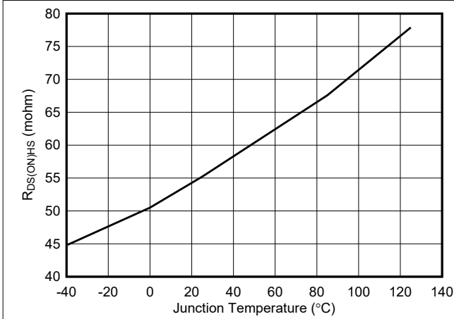
6-7. High-Side R_{DS(on)}
