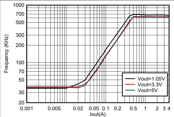
6-12. TPS564255 Frequency vs Loading, V_{IN} = 12\text{ V}
