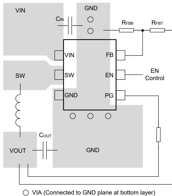
8-26. Suggested Layout
