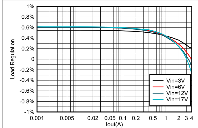
8-6. TPS564257 Load Regulation vs Loading
