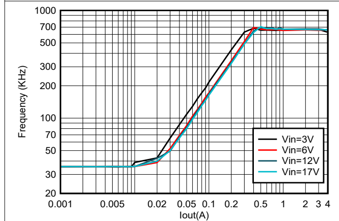
8-4. TPS564255 Frequency vs Loading
