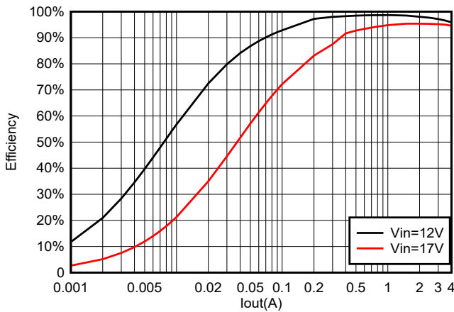
6-23. TPS564257 Efficiency at 10 V_{OUT} with a 6.8- \mu\text{H} Inductor
