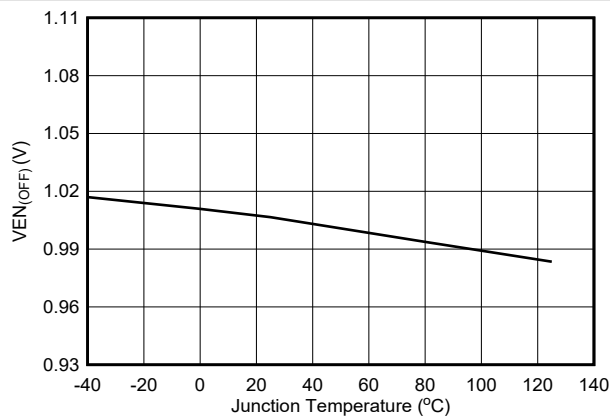
6-5. Enable Off Threshold Voltage
