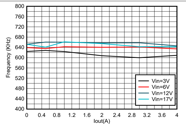
8-3. TPS564257 Frequency vs Loading
