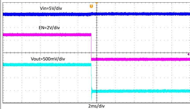
8-12. Shutdown Through EN, I_{OUT} = 6\text{ A}
