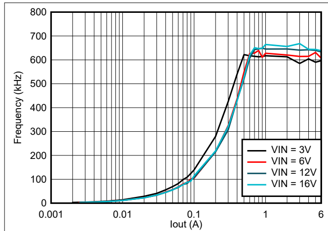
8-2. TPS566242 Frequency vs Loading
