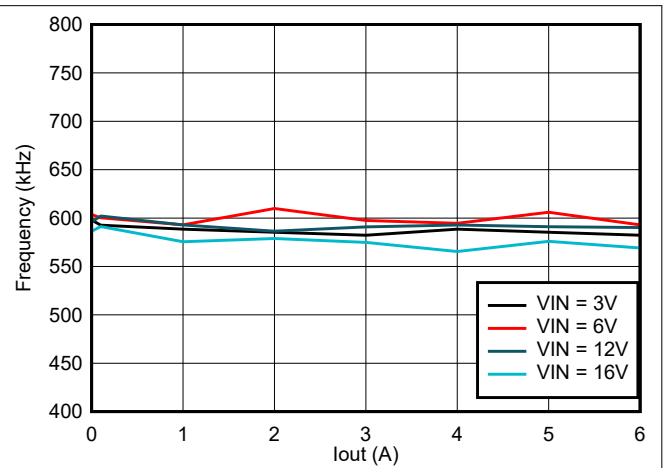
8-3. TPS566247 Frequency vs Loading
