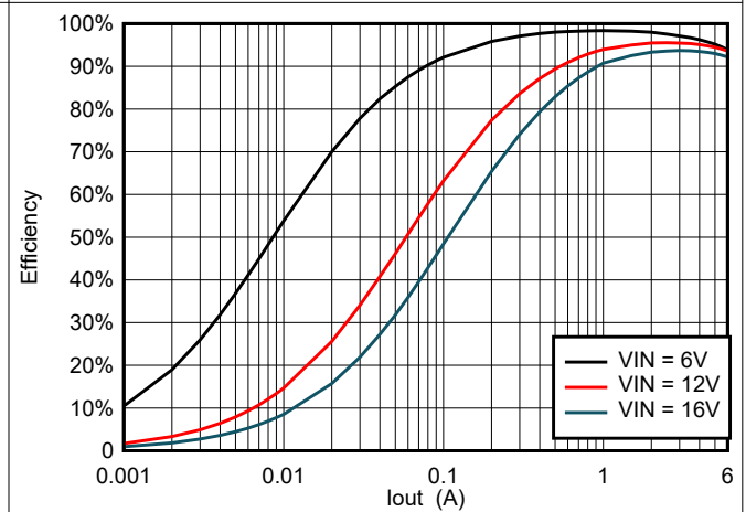
6-18. TPS566247 Efficiency at 5 V_{OUT} with a 2.2- \mu\text{H} Inductor
