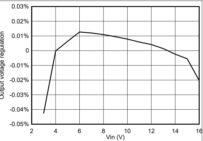
8-7. TPS566247 Line Regulation vs Loading with 6-A Loading
