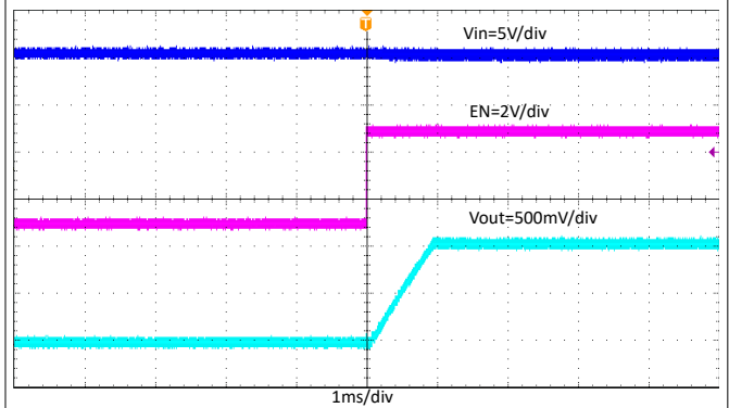
8-11. Start-Up Through EN, I_{OUT} = 6\text{ A}
