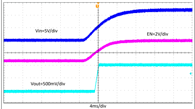
8-13. Start-Up with V_{IN} Rising, I_{OUT} = 6\text{ A}
