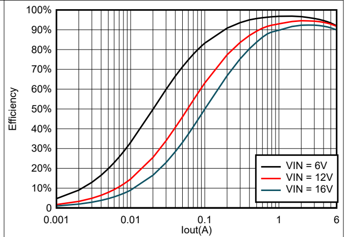
6-16. TPS566247 Efficiency at 3.3 V_{OUT} with a 2.2- \mu\text{H} Inductor
