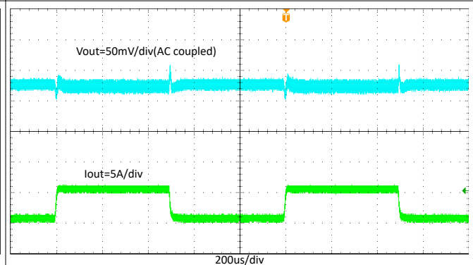
8-17. TPS566247 Transient Response with 0.6 A to 5.4 A by 2.5-A/ \mu\text{s} Load Step
