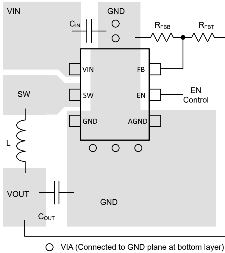
10-1. Suggested Layout
