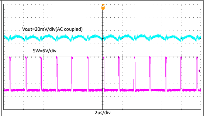
8-9. TPS566247 Output Voltage Ripple with 0.01-A Loading
