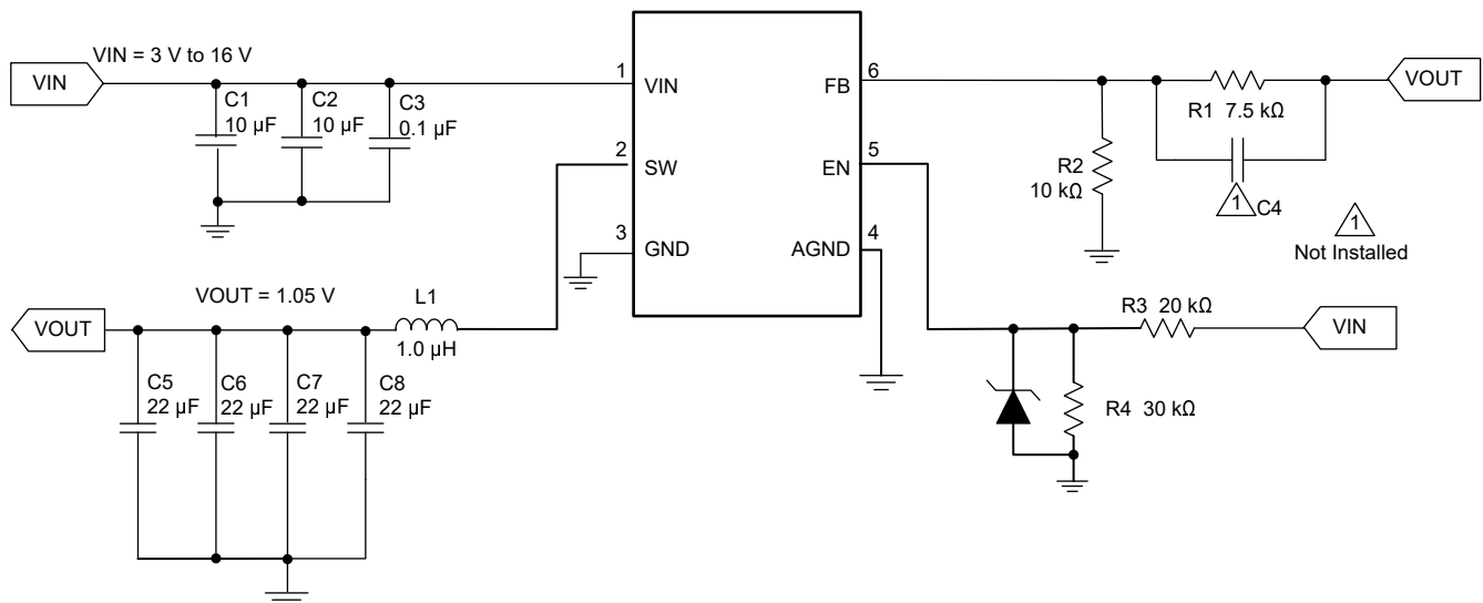
Figure 8-1. Schematic
