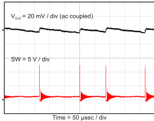
8-11. Output Voltage Ripple, I_{OUT} = 10\text{ mA}
