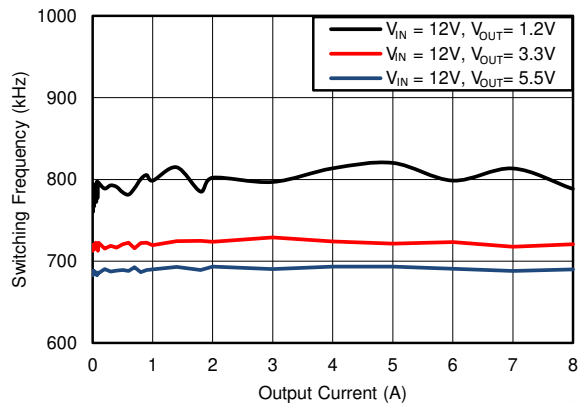
6-18. F_{SW} Load Regulation, Mode = FCCM, F_{SW} = 800\text{kHz}
