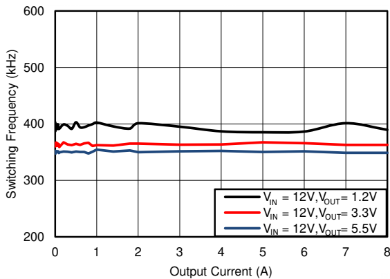
6-17. F_{SW} Load Regulation, Mode = FCCM, F_{SW} = 400\text{kHz}
