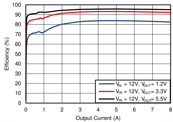
6-14. Efficiency, Mode = DCM, F_{SW} = 1200\text{kHz}
