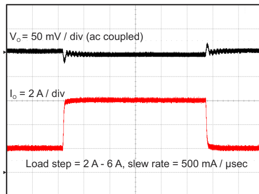
8-18. Transient Response
