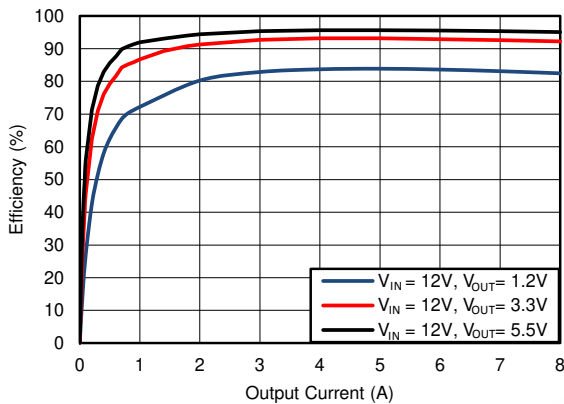
6-15. Efficiency, Mode = FCCM, F_{SW} = 1200\text{kHz}
