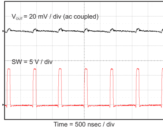
8-13. Output Voltage Ripple, I_{OUT} = 8\text{ A}
