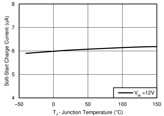
6-6. Soft-Start Charge Current vs Temperature
