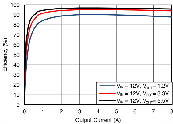
6-13. Efficiency, Mode = FCCM, F_{SW} = 400\text{kHz}
