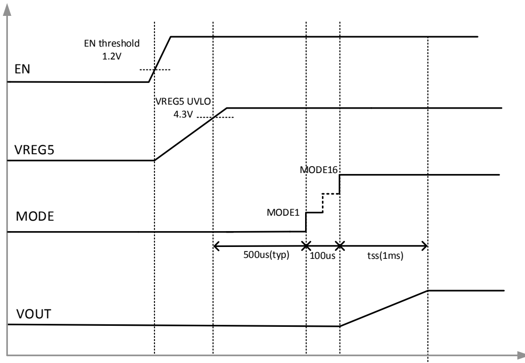
☒ 7-1. Power-Up Sequence
