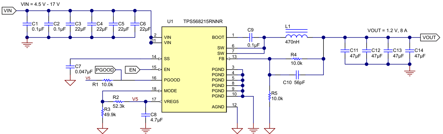
図 8-1. Application Schematic
