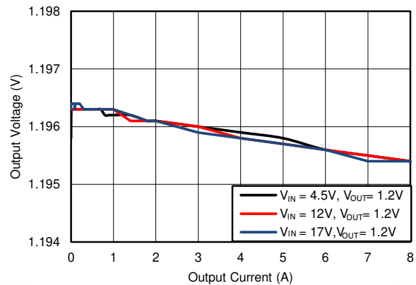
6-16. Load Regulation, F_{SW} = 400\text{kHz}
