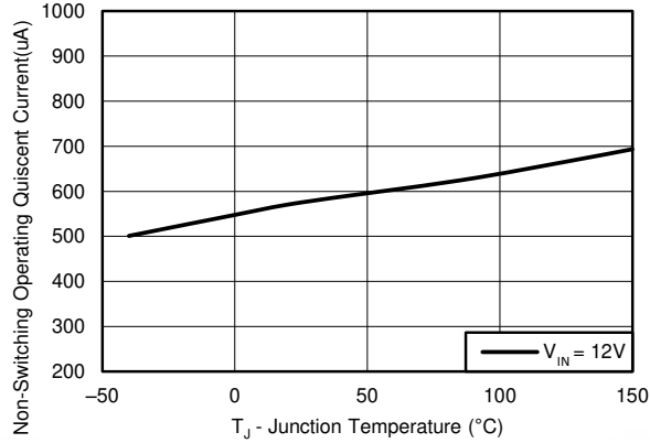
6-1. Quiescent Current vs Temperature
