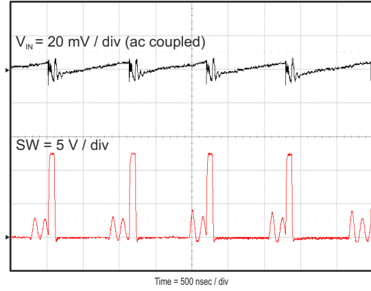
8-9. Input Voltage Ripple, I_{OUT} = 700\text{ mA}
