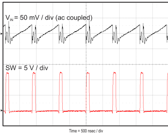
8-10. Input Voltage Ripple, I_{OUT} = 8\text{ A}
