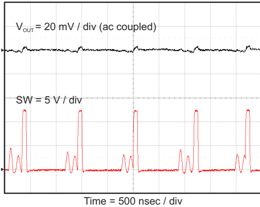
8-12. Output Voltage Ripple, I_{OUT} = 700\text{ mA}
