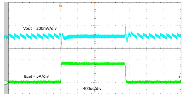
7-11. Transient Response 0A to 8A
