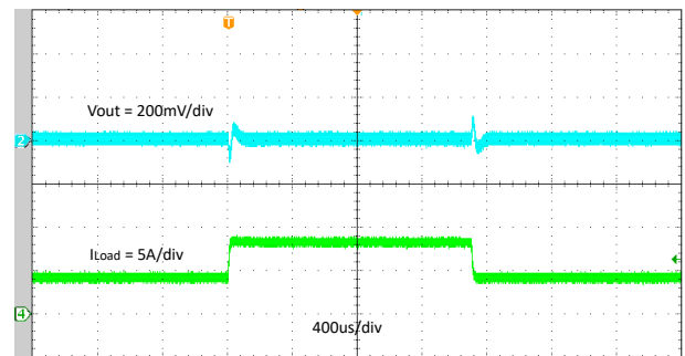
7-13. Transient Response 4A to 8A
