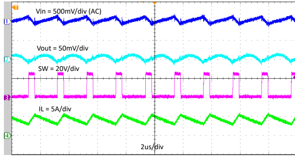
7-8. Steady State Waveforms, I_{OUT} = 4A
