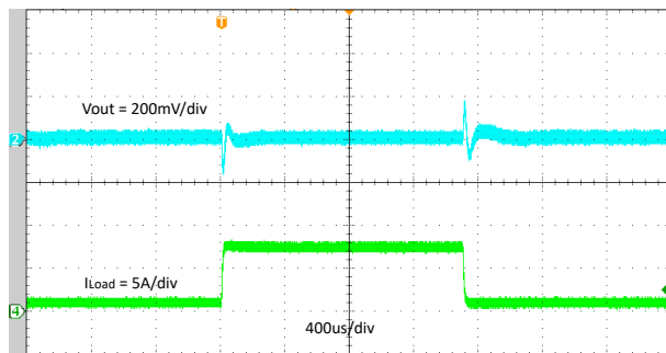
7-12. Transient Response 0.8A to 7.2A
