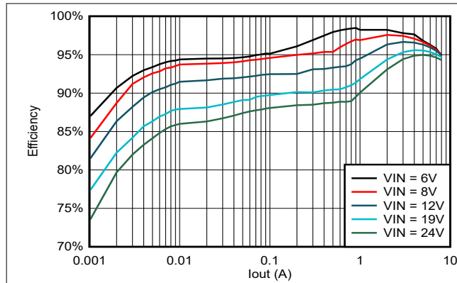
图 5-17. TPS56837 Efficiency, Vout = 5V, Fsw = 500kHz
