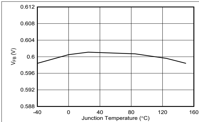
5-5. Feedback Voltage vs Temperature
