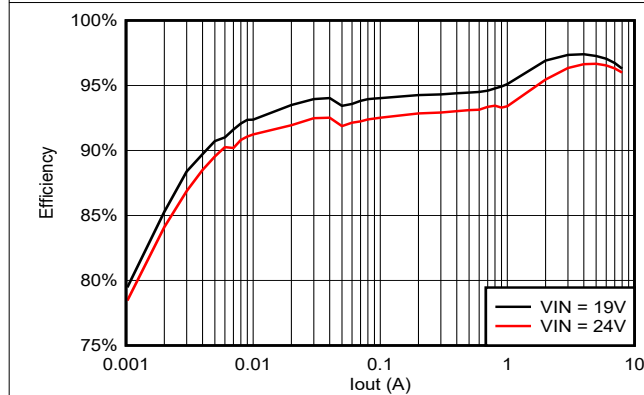
图 5-21. TPS56837 Efficiency, Vout = 12V, Fsw = 800kHz
