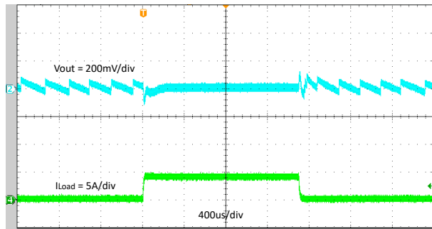
7-10. Transient Response 0A to 4A
