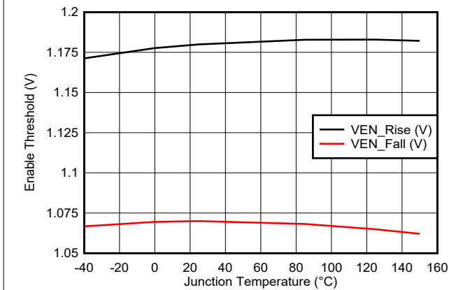
5-7. EN Threshold vs Temperature
