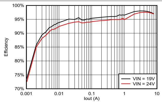
图 5-20. TPS56837 Efficiency, Vout = 12V, Fsw = 500kHz
