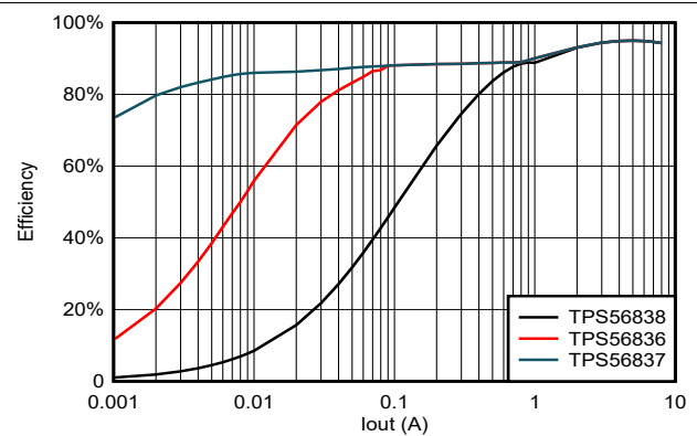
图 5-22. TPS56837, TPS56838 and TPS56836 Efficiency, Vin = 24V, Vout = 5V, Fsw = 500kHz
