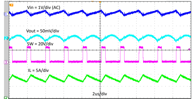
7-9. Steady State Waveforms, I_{OUT} = 8A
