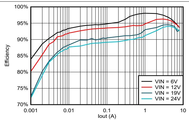
图 5-18. TPS56837 Efficiency, Vout = 5V, Fsw = 800kHz
