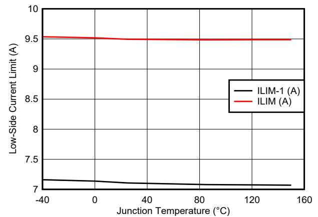
5-8. Low-Side Valley Current Limit vs Temperature
