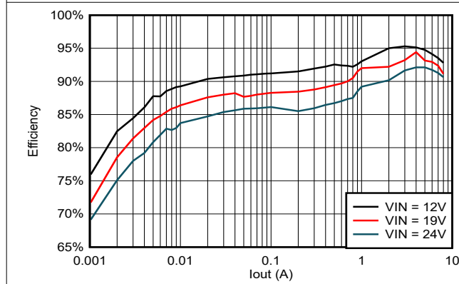
图 5-19. TPS56837 Efficiency, Vout = 5V, Fsw = 1200kHz
