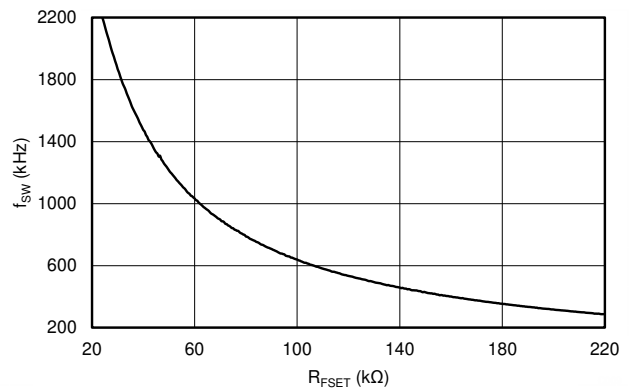
6-6. Boost Switching Frequency f_{SW} vs R_{FSET}
