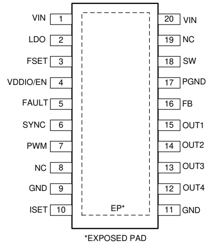
图 5-1. PWP Package 20-Pin HTSSOP With Exposed Thermal Pad Top View
