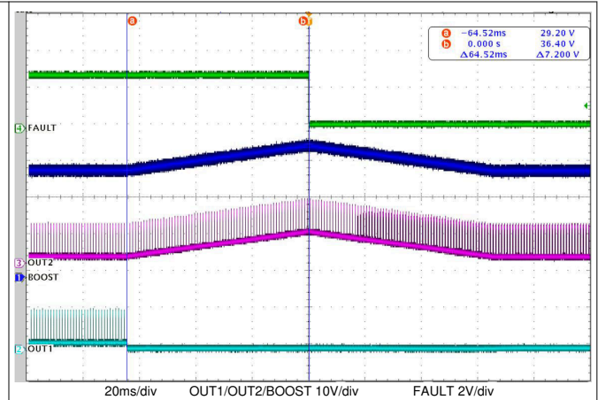
8-5. Open LED Fault
