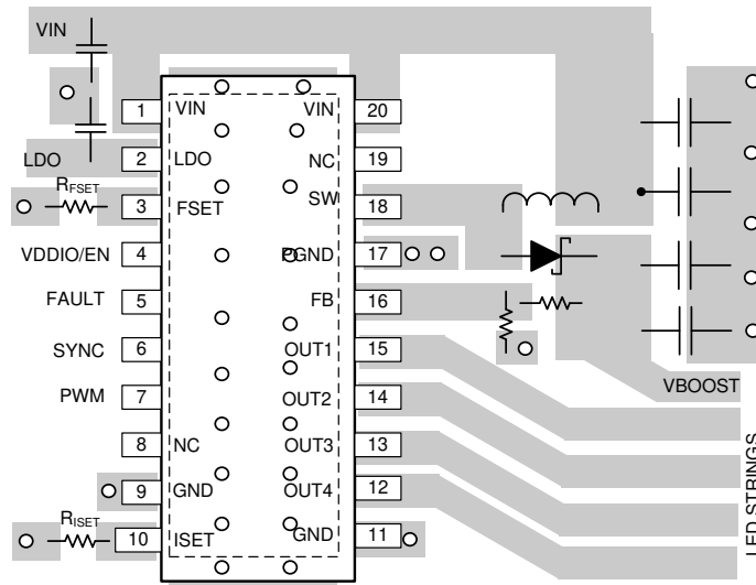
10-1. TPS61194 Boost Layout
