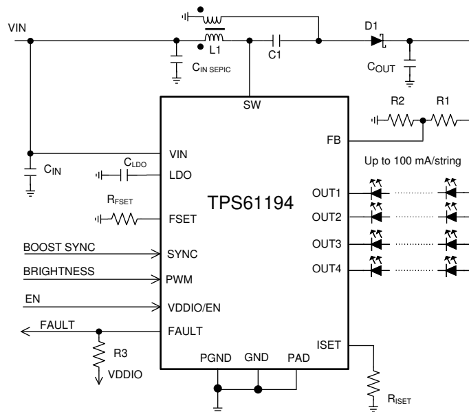
8-6. SEPIC Mode, 4 Strings, 100 mA per String Configuration
