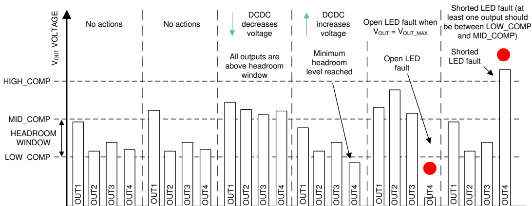
7-4. Protection and DC-DC Voltage Adaptation Algorithms
