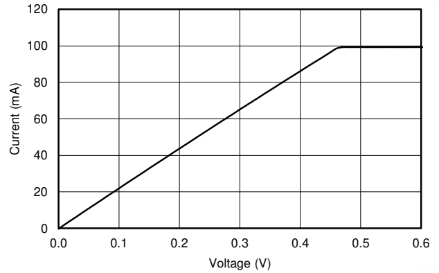
6-8. LED Current Sink Saturation Voltage
