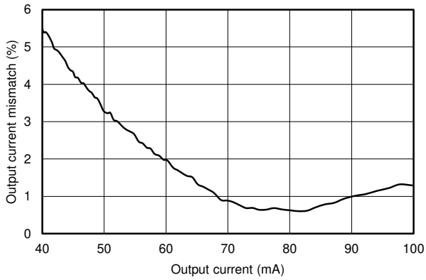
6-7. LED Current Sink Matching
