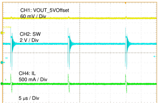
9-2. Steady 10 mA
