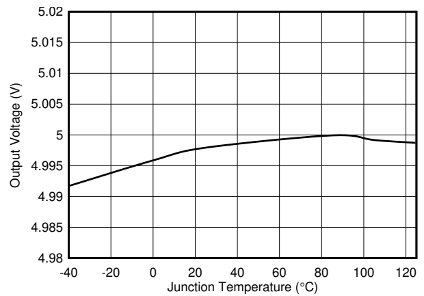
7-6. V_{OUT} vs Temperature
