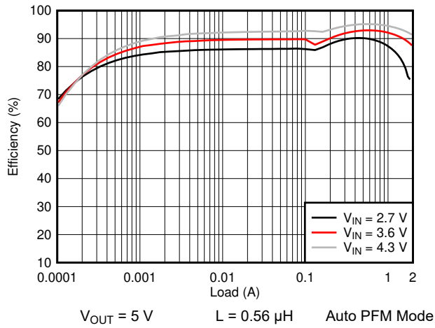
7-1. Efficiency vs Load
