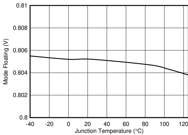
7-15. Mode Floating vs Temperature
