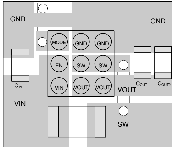
10-1. Recommended Layout
