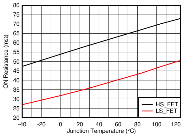
7-5. R_{DS(ON)} vs Temperature
