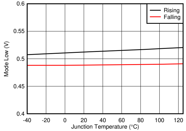
7-14. Mode Low Rising / Falling vs Temperature
