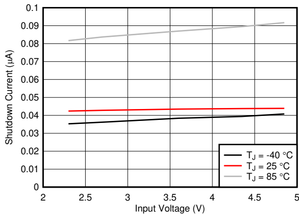
7-9. Shutdown Current vs Input Voltage
