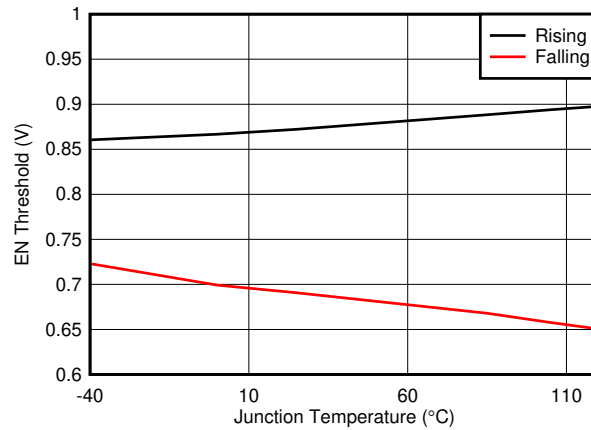
7-17. EN Threshold vs Temperature
