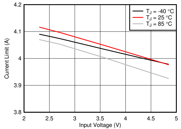
7-10. Current Limit (Auto PFM) vs Input Voltage
