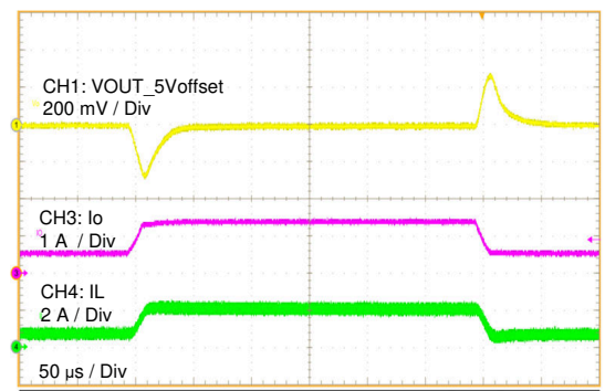
9-5. Load Sweep
