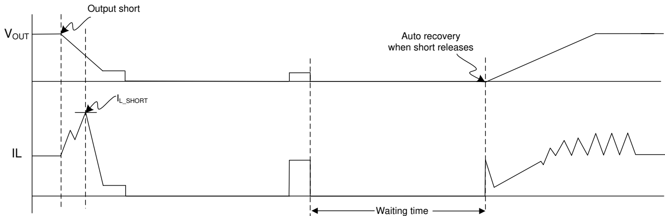
8-2. Hiccup Mode Short Protection
