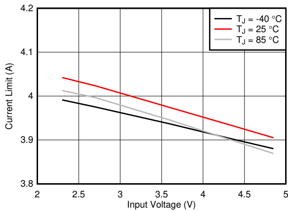
7-11. Current Limit (Forced PWM) vs Input Voltage
