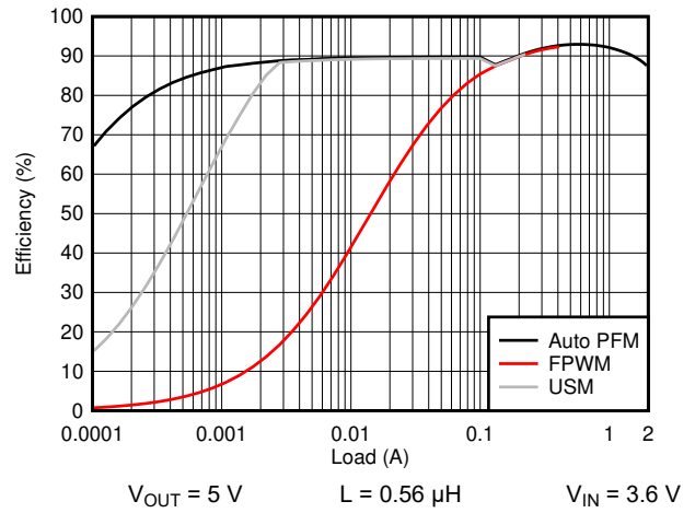
7-2. Efficiency vs Load
