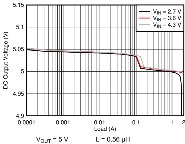
7-3. DC Output Voltage vs Load
