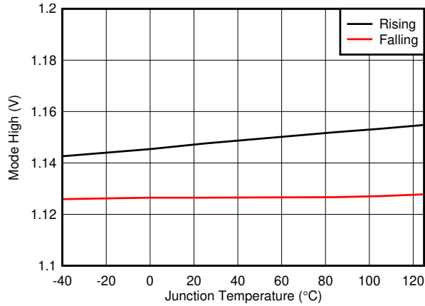
7-13. Mode High Rising / Falling vs Temperature
