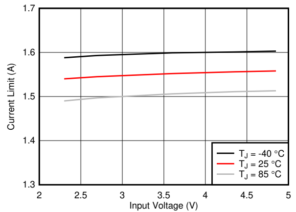
7-12. DC Startup Current Limit vs Input Voltage
