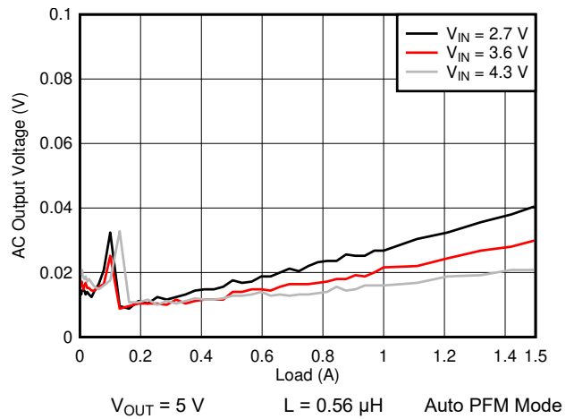
7-4. AC Output Voltage vs Load
