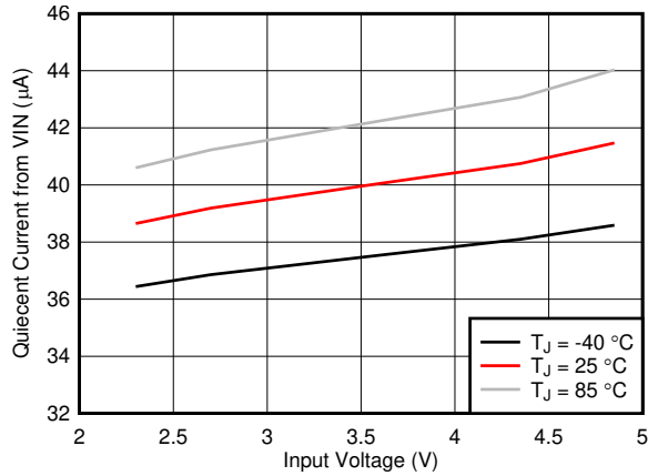
7-7. Quiescent Current (from VIN) vs Input Voltage
