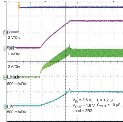
Figure 9-15. Startup Into Load – V_{OUT} = 1.8 \text{ V}
