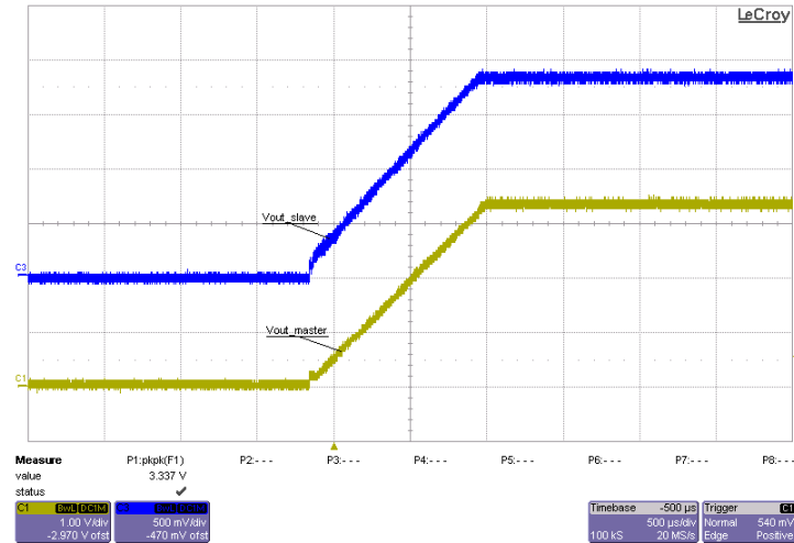
10-58. Scope Plot for Output Voltage Tracking
