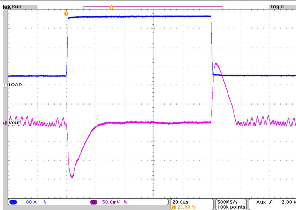
10-22. Load Transient Response V_{OUT} = 3.3\text{ V} PFM T_A = 25^\circ\text{C} V_{IN} = 5.0\text{ V} I_{OUT} = 0.4\text{ A to } 3.6\text{ A to } 0.4\text{ A}
