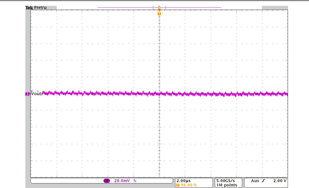
10-47. Output Voltage Ripple
