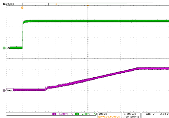
10-53. Start-Up Timing
