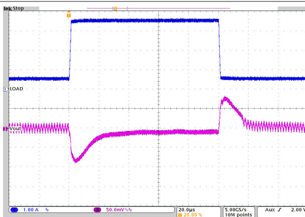
10-24. Load Transient Response V_{OUT} = 1.8\text{ V} PFM T_A = 25^\circ\text{C} V_{IN} = 5.0\text{ V} I_{OUT} = 0.4\text{ A to } 3.6\text{ A to } 0.4\text{ A}
