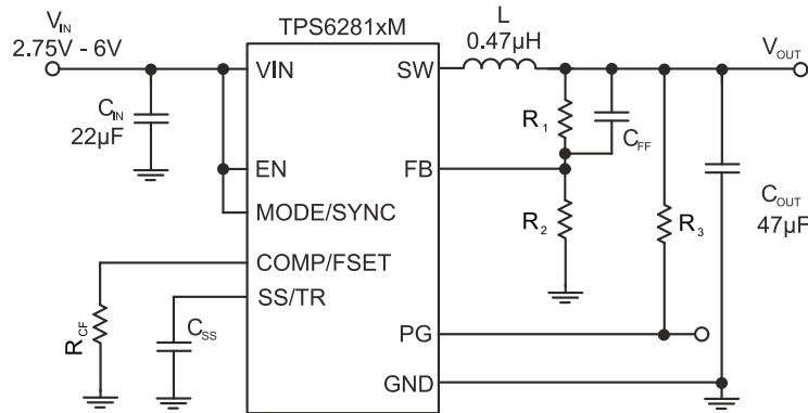
10-1. Typical Application
