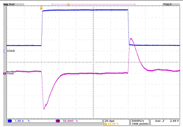
10-23. Load Transient Response V_{OUT} = 3.3\text{ V} PWM T_A = 25^\circ\text{C} V_{IN} = 5.0\text{ V} I_{OUT} = 0.4\text{ A to } 3.6\text{ A to } 0.4\text{ A}
