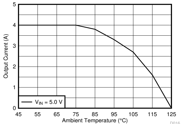
8-30. Thermal Derating
