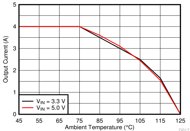
8-29. Thermal Derating
