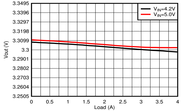
8-22. Load Regulation
