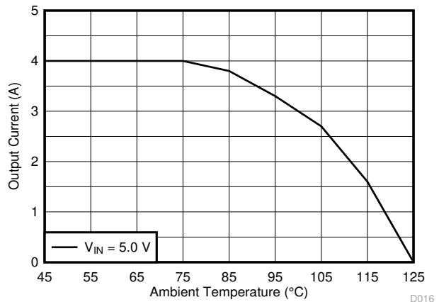
V_{OUT} = 3.3V \theta_{JA} = 71.4^\circ C/W
