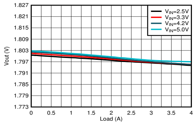
8-14. Load Regulation
