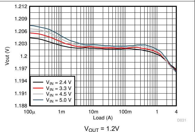
図 8-8. Load Regulation
