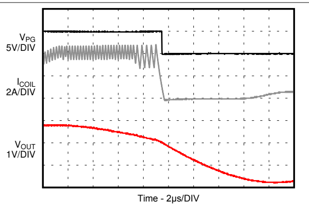
I_{OUT} = 1A TPS6282x
