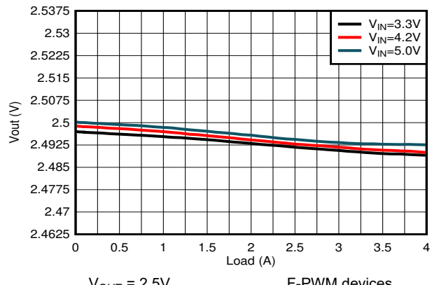
8-18. Load Regulation
