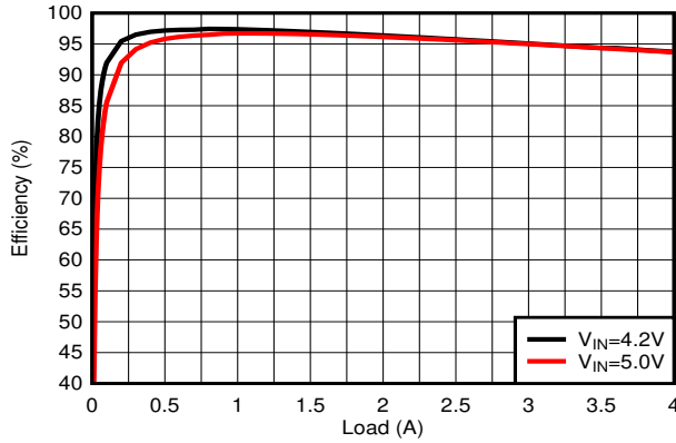
8-21. PWM Efficiency
