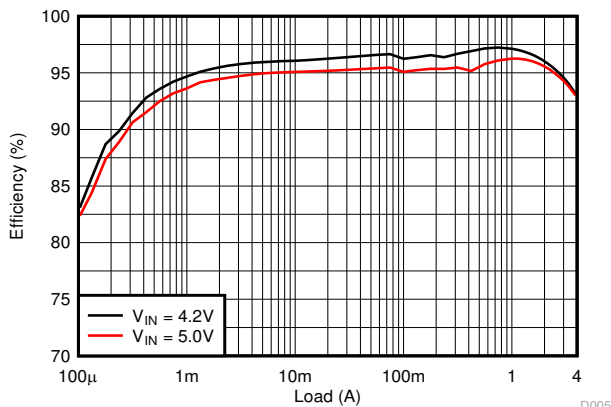
8-17. PWM Efficiency
