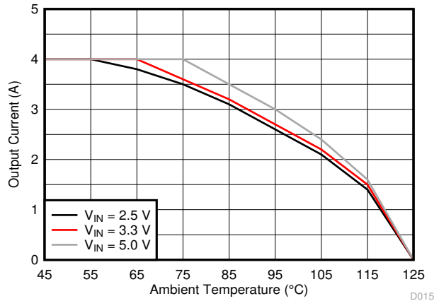
V_{OUT} = 1.8V \theta_{JA} = 71.4^\circ C/W
