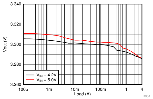
8-20. Load Regulation
