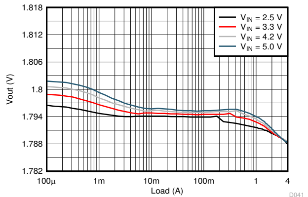
8-10. Load Regulation
