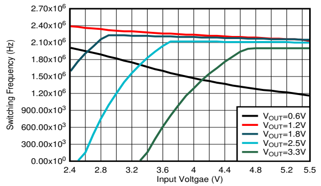
8-24. Switching Frequency
