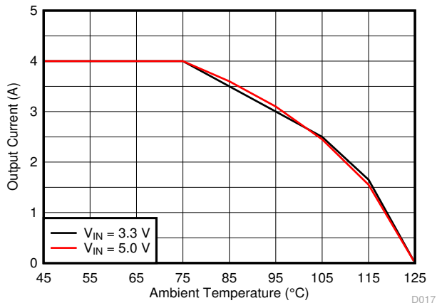
V_{OUT} = 2.5V \theta_{JA} = 71.4^\circ C/W
