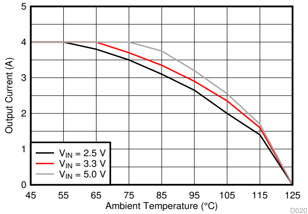
V_{OUT} = 1.2V \theta_{JA} = 71.4^\circ C/W
