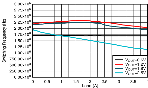
8-23. Switching Frequency
