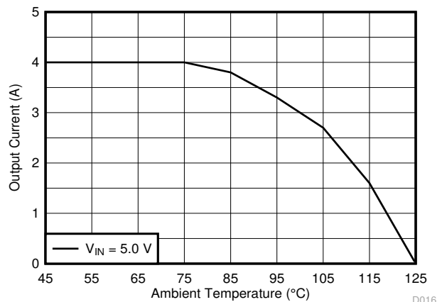
8-30. Thermal Derating
