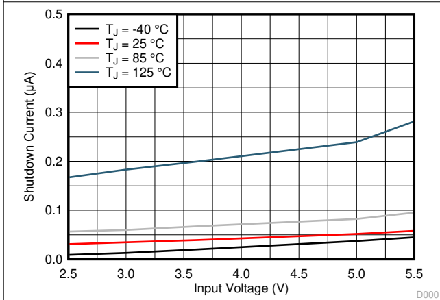
图 6-3. Shutdown Current
