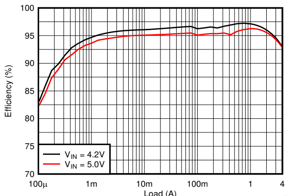
8-17. PWM Efficiency
