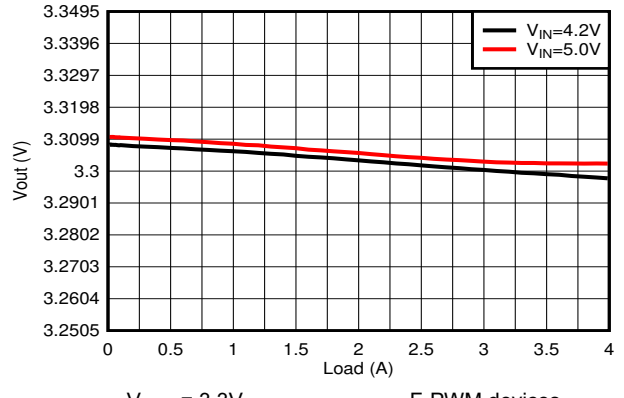
8-22. Load Regulation
