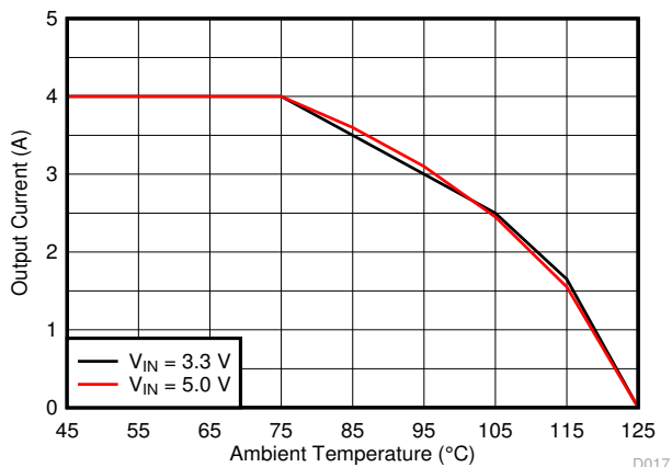
8-29. Thermal Derating
