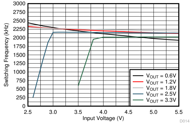
8-28. Switching Frequency
