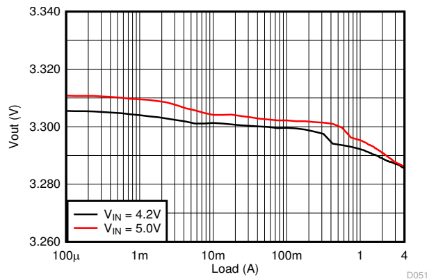
8-20. Load Regulation
