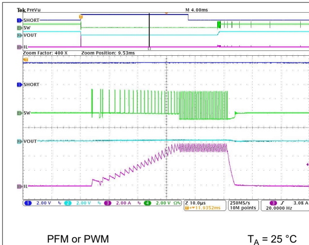
8-45. HICCUP Short-Circuit Protection (Zoom In - Second Hiccup)
