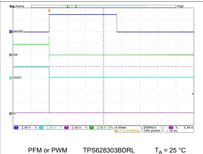
8-46. Latch-off Short-Circuit Protection
