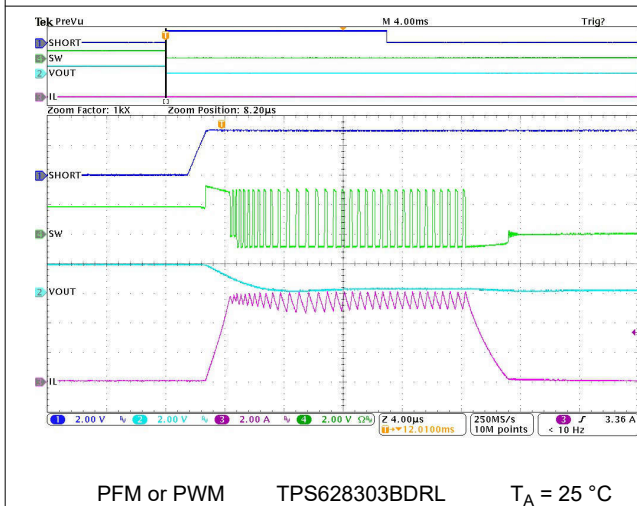
8-47. Latch-off Short-Circuit Protection (Zoom In)
