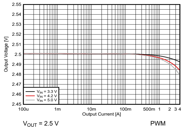
8-24. Output Voltage versus Output Current
