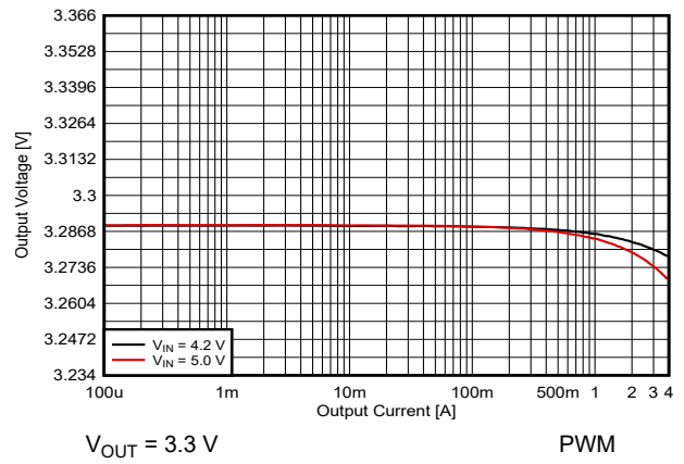
8-26. Output Voltage versus Output Current
