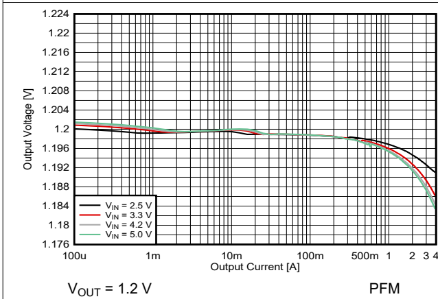
8-19. Output Voltage versus Output Current
