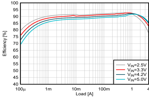
8-9. Efficiency versus Output Current
