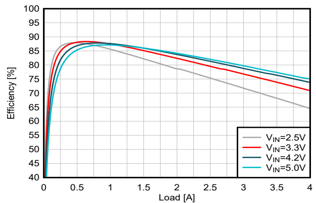
8-12. Efficiency versus Output Current
