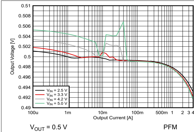
8-15. Output Voltage versus Output Current
