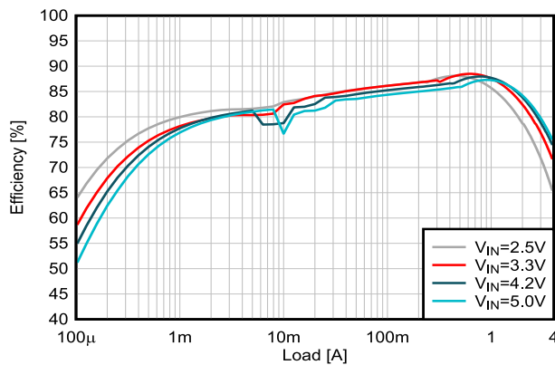
8-11. Efficiency versus Output Current
