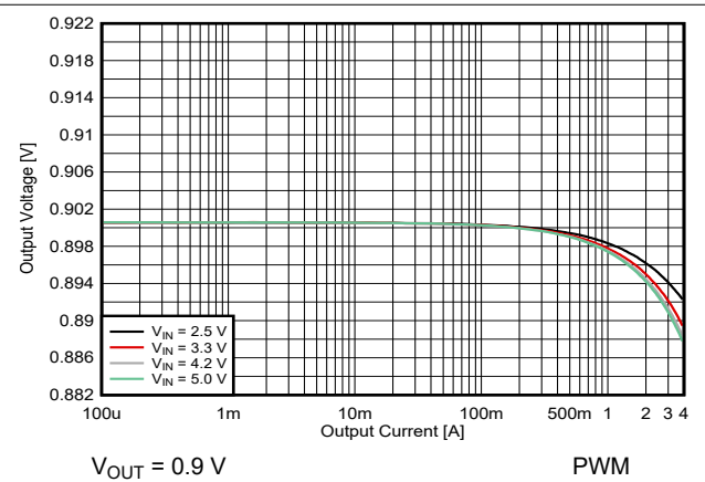
8-18. Output Voltage versus Output Current
