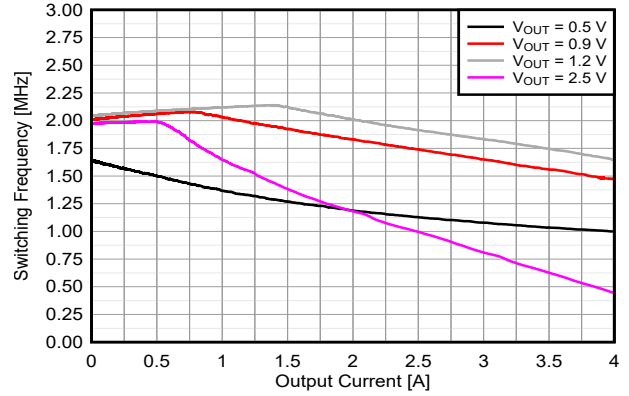
8-28. Switching Frequency versus Output Current
