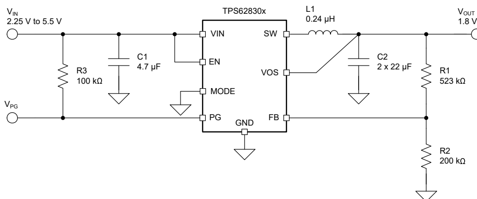
図 8-2. Typical Application of TPS62830x (Optimized for Transient Response)
