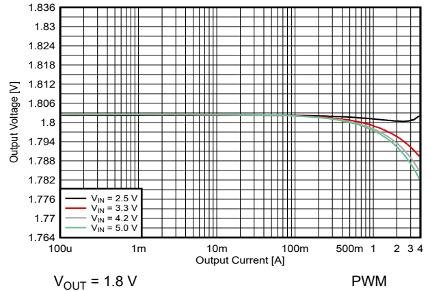
8-22. Output Voltage versus Output Current
