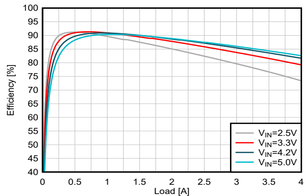
8-10. Efficiency versus Output Current
