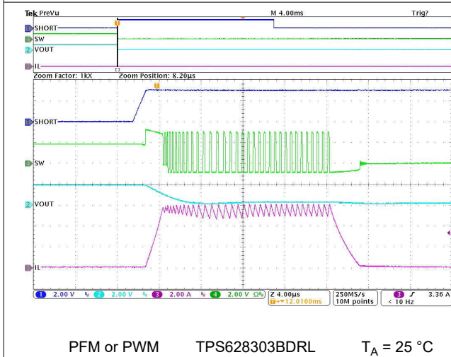
PFM or PWM T_A = 25\text{ }^\circ\text{C} 8-45. HICCUP Short-Circuit Protection (Zoom In - Second Hiccup)
