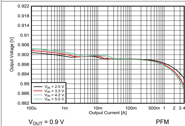
8-17. Output Voltage versus Output Current
