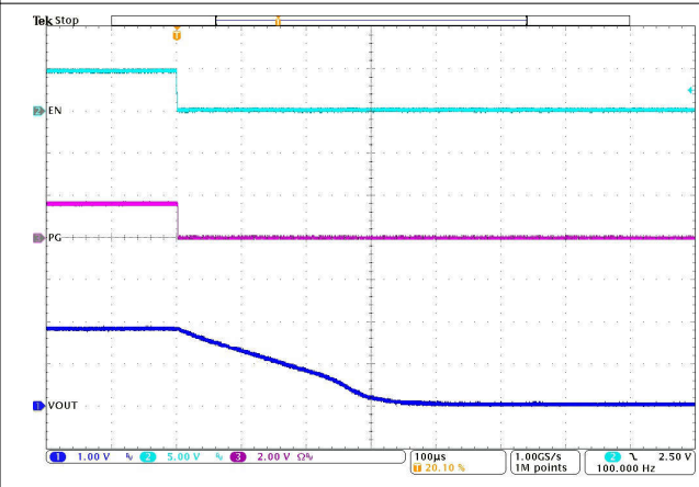
I_{OUT} = 0\text{ mA} PFM T_A = 25\text{ }^\circ\text{C}
