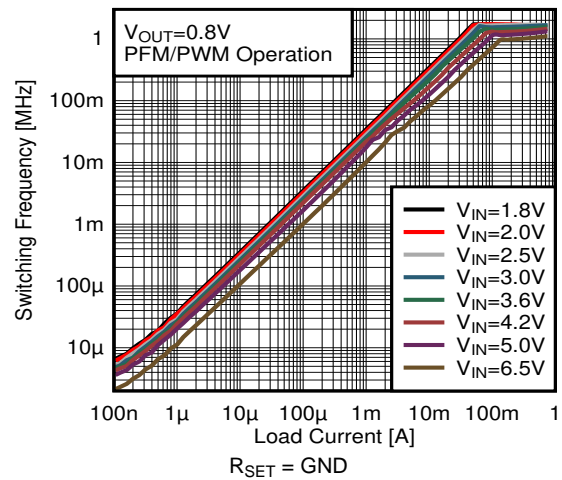
35. Switching Frequency versus Load Current V_{OUT} = 0.8\text{ V}
