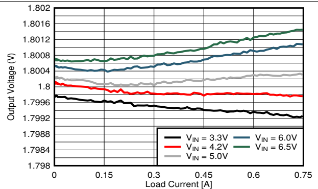
EN = VIN MODE = HIGH 43. Output Voltage Accuracy (Load Regulation)
