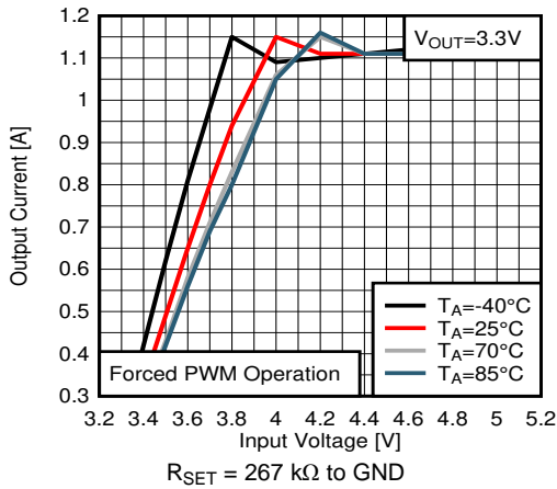
34. Maximum Output Current versus Input Voltage V_{OUT} = 3.3\text{ V}
