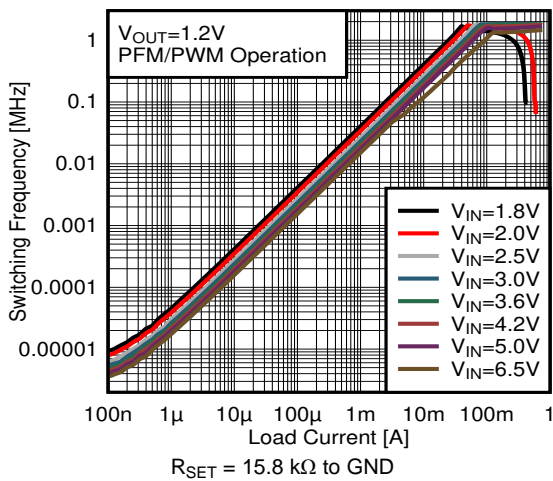
36. Switching Frequency versus Load Current V_{OUT} = 1.2\text{ V}
