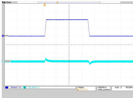
10-38. Line Transient Response
