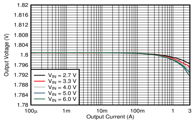
10-11. Output Voltage Versus Output Current
