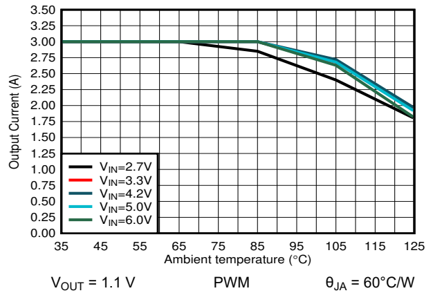
10-19. Output Current Versus Ambient Temperature
