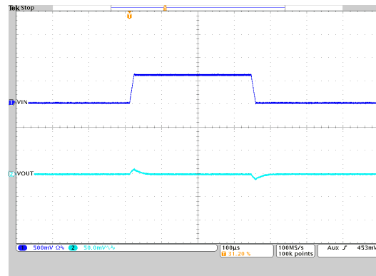
10-39. Line Transient Response
