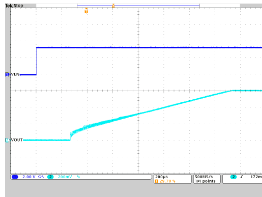
10-56. Start-Up Timing
