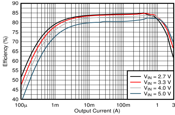
10-8. Efficiency Versus Output Current
