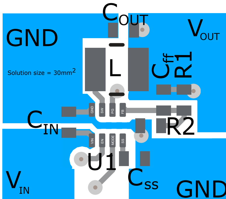
Figure 12-1. Example Layout
