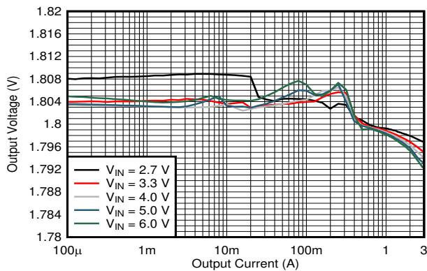
10-10. Output Voltage Versus Output Current
