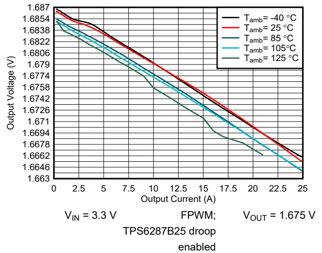
9-19. Output Voltage Versus Output Current
