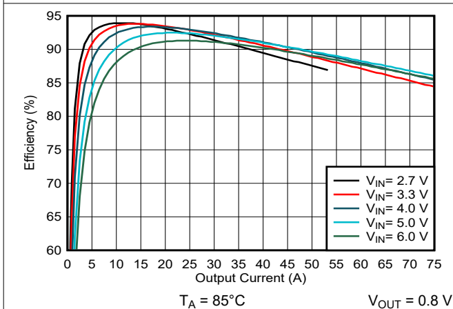
9-38. Efficiency Versus Output Current
