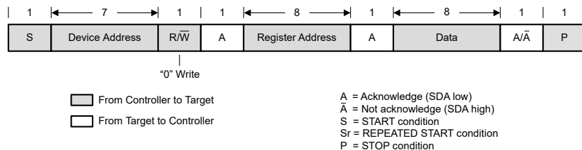
☒ 8-20. : "Write" Data Transfer Format in Standard-, Fast, Fast-Plus Modes
