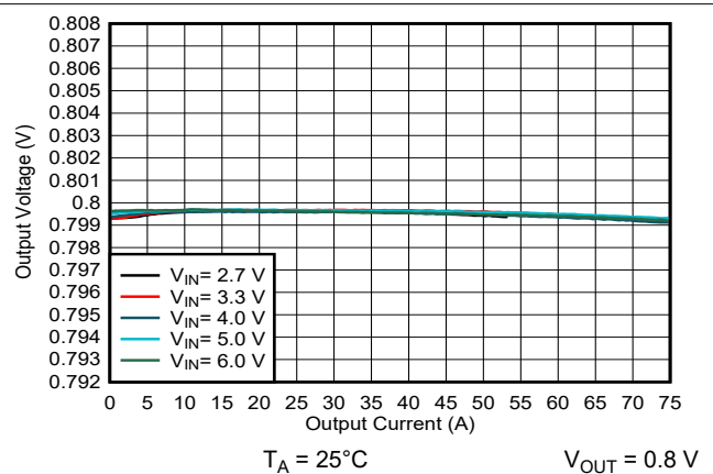
9-37. Output Voltage Versus Output Current
