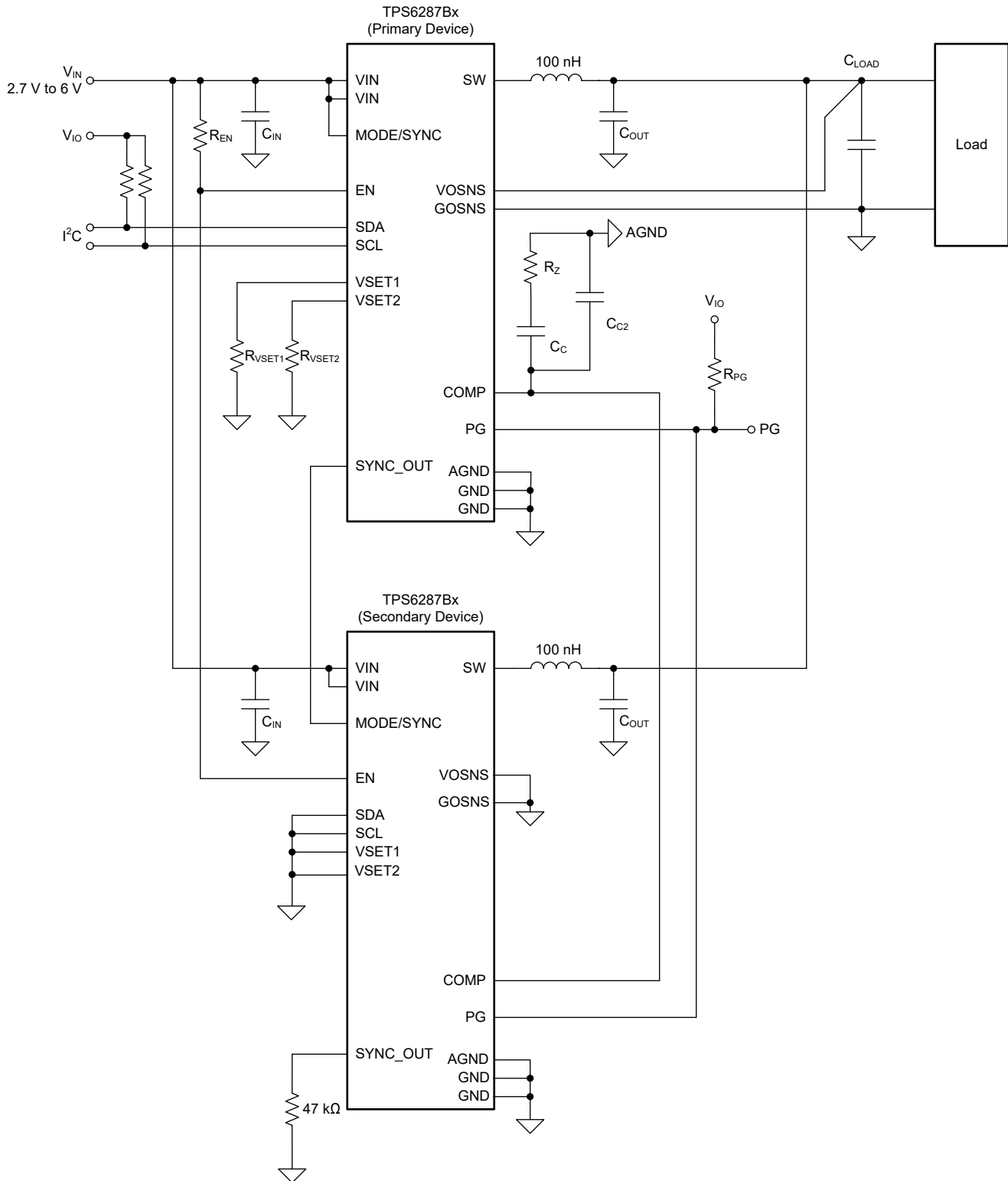
図 9-26. Stacking Two Devices for up to 50 A
