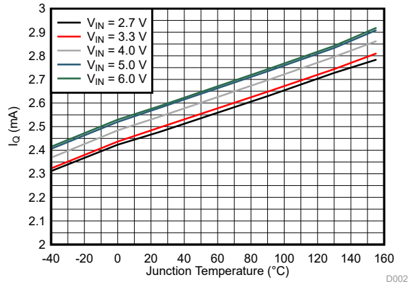
図 6-4. Quiescent Current vs Temperature
