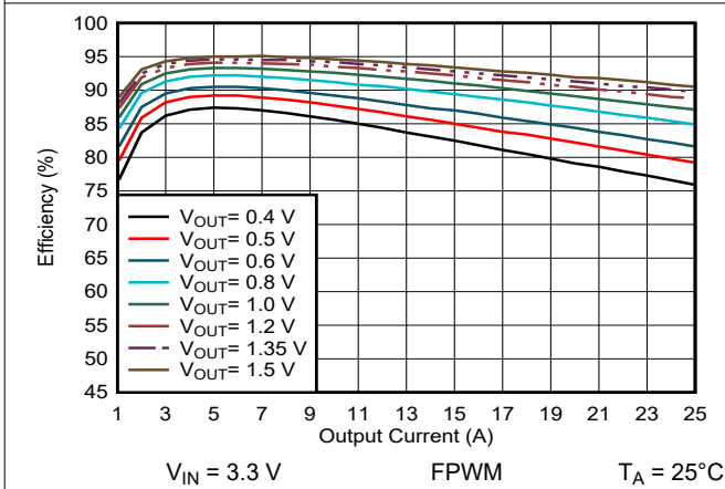
9-4. Efficiency Versus Output Current
