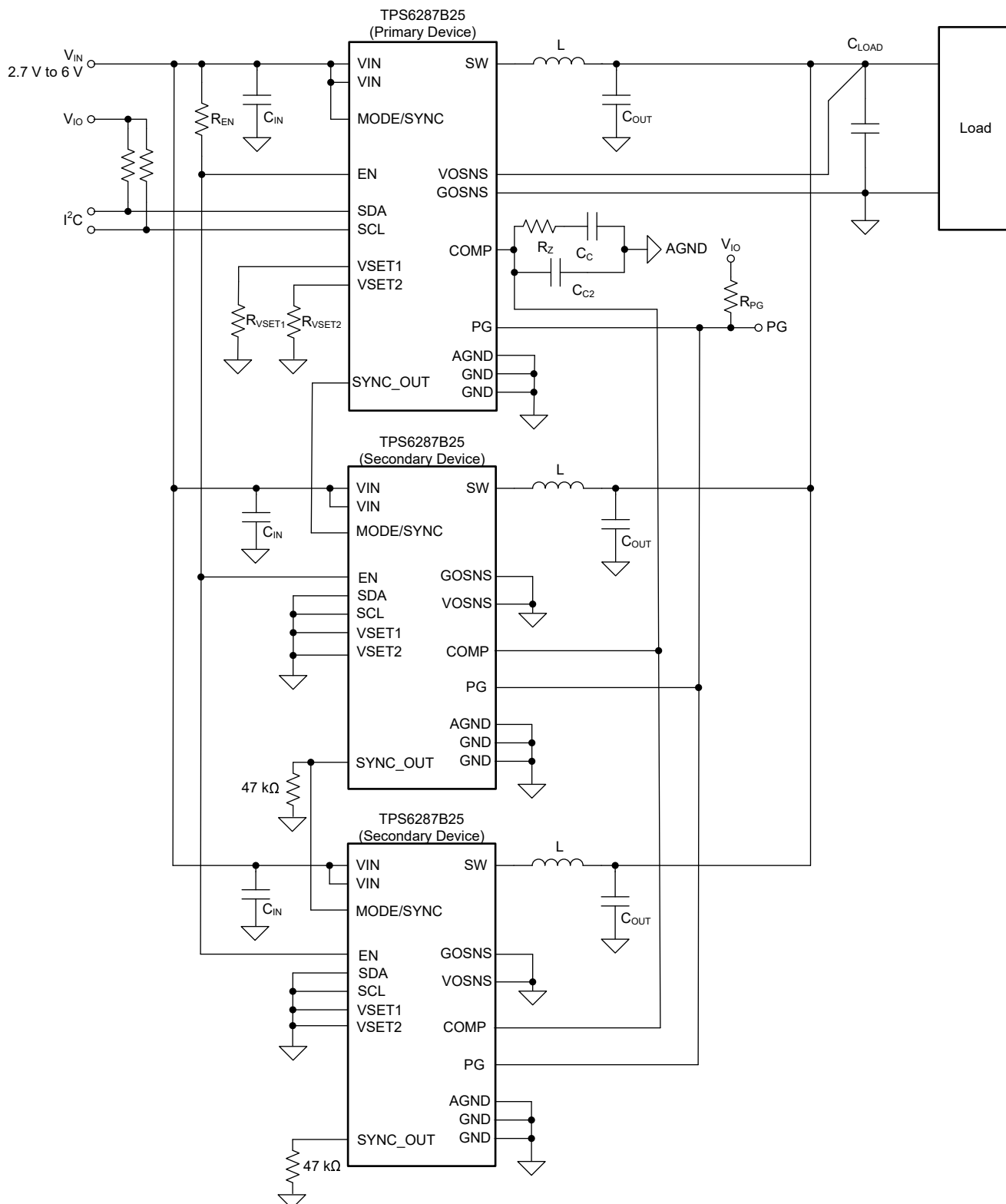
図 9-35. Stacking Three Devices
