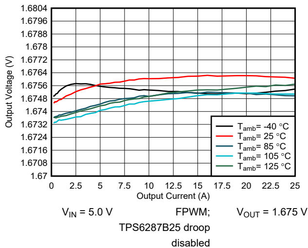
9-12. Output Voltage Versus Output Current
