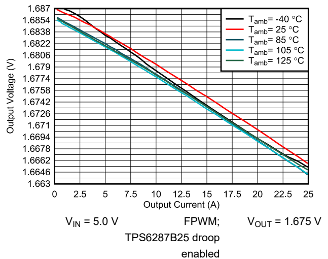
9-13. Output Voltage Versus Output Current
