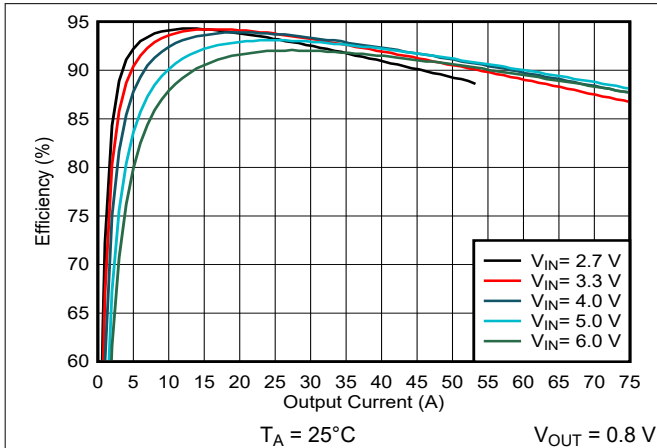
9-36. Efficiency Versus Output Current
