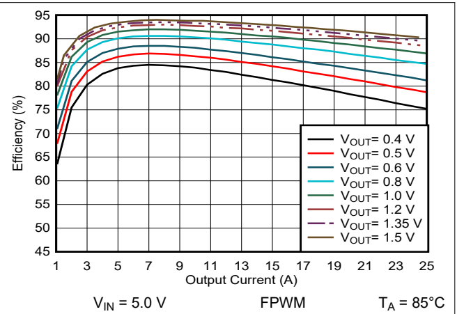
9-3. Efficiency Versus Output Current
