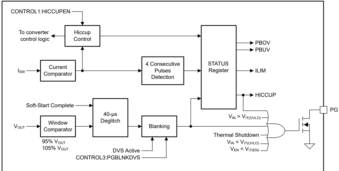
図 8-13. Power-Good Functional Block Diagram (Standalone / Primary Device)
