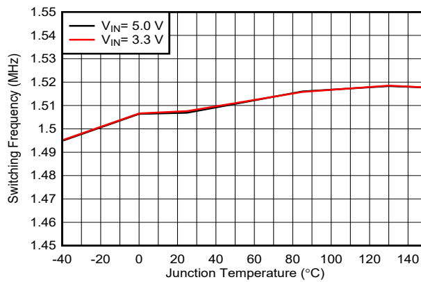
図 6-5. Switching Frequency vs Temperature
