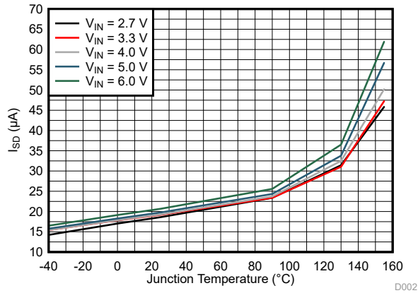
図 6-3. Shutdown Current vs Temperature
