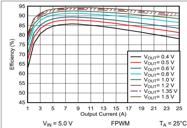
9-2. Efficiency Versus Output Current
