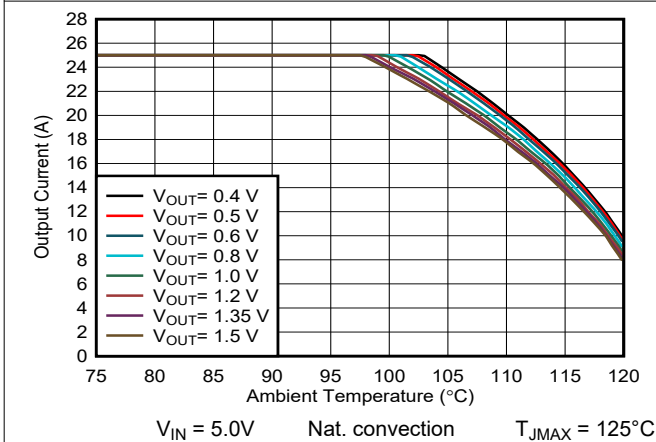
9-6. Safe Operating Area
