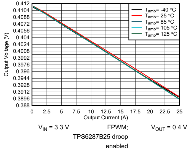
9-15. Output Voltage Versus Output Current
