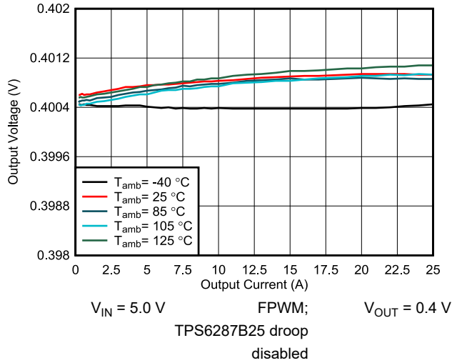
9-8. Output Voltage Versus Output Current
