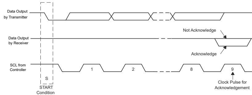
☒ 8-18. Acknowledge on the I 2 C Bus
