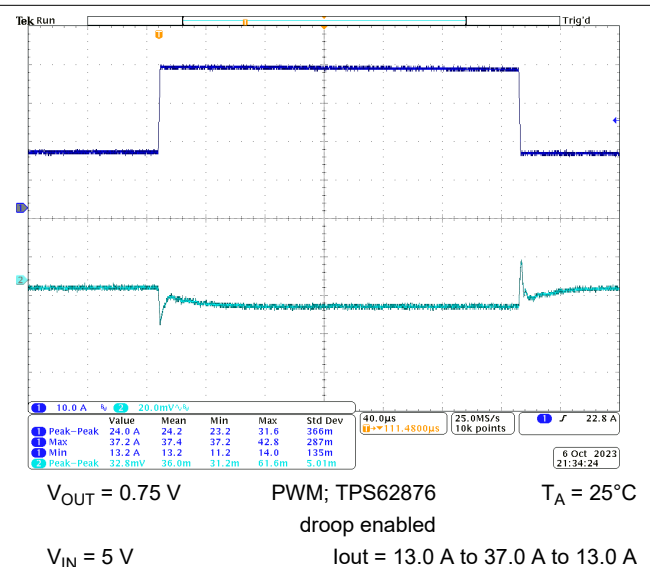
图 9-32. Load Transient Response
