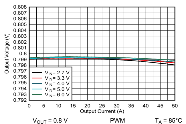
图 9-30. Output Voltage Versus Output Current
