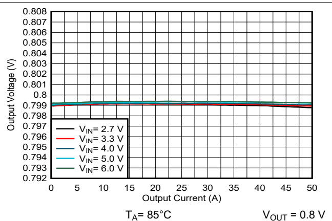
9-39. Output Voltage Versus Output Current
