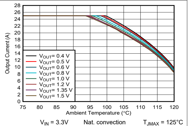
9-7. Safe Operating Area
