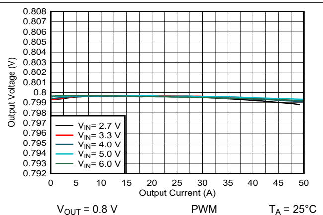
图 9-28. Output Voltage Versus Output Current
