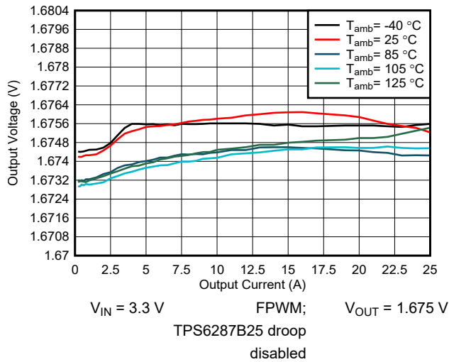
9-18. Output Voltage Versus Output Current
