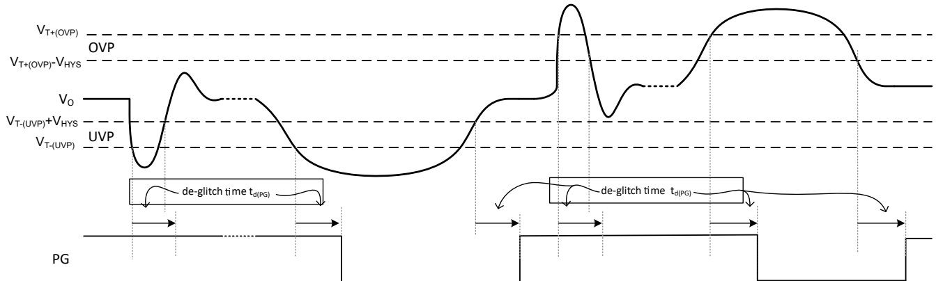
図 8-12. PG Timing
