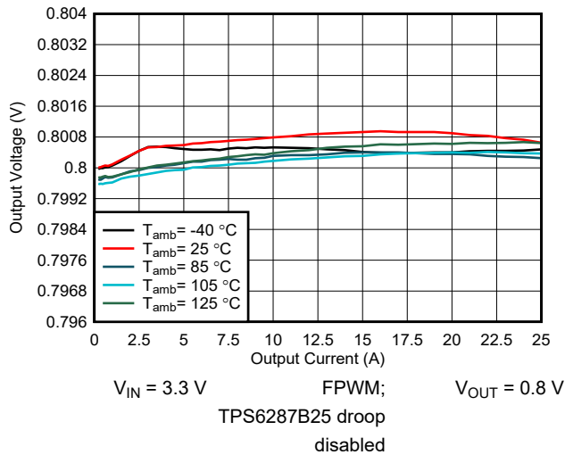
9-16. Output Voltage Versus Output Current
