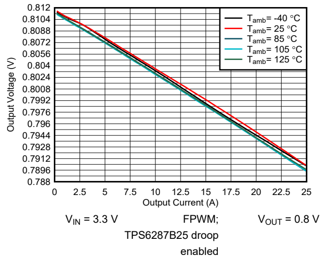
9-17. Output Voltage Versus Output Current
