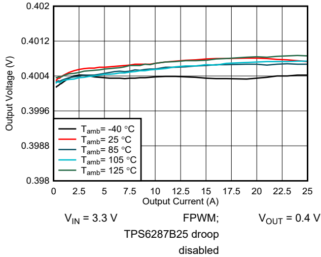
9-14. Output Voltage Versus Output Current
