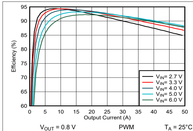
图 9-27. Efficiency Versus Output Current
