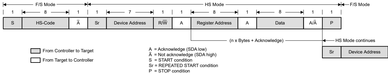
8-22. Data Transfer Format in HS-Mode
