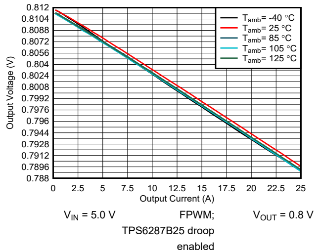
9-11. Output Voltage Versus Output Current
