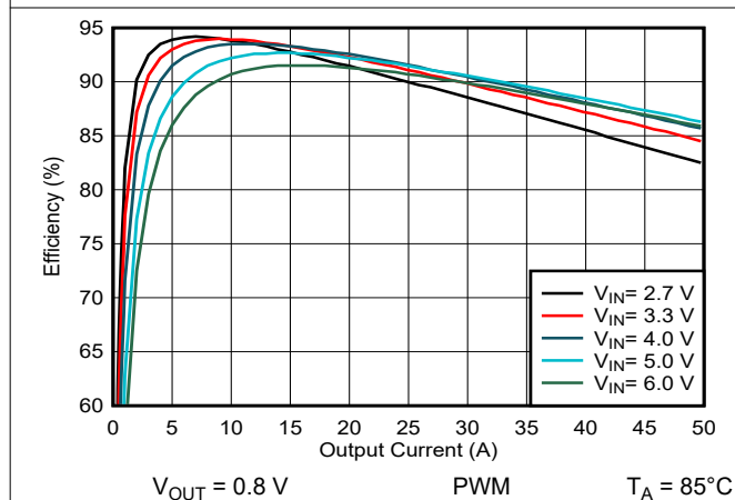
图 9-29. Efficiency Versus Output Current
