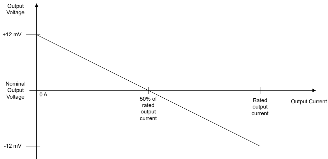
図 8-10. Voltage Scaling with Output Current
