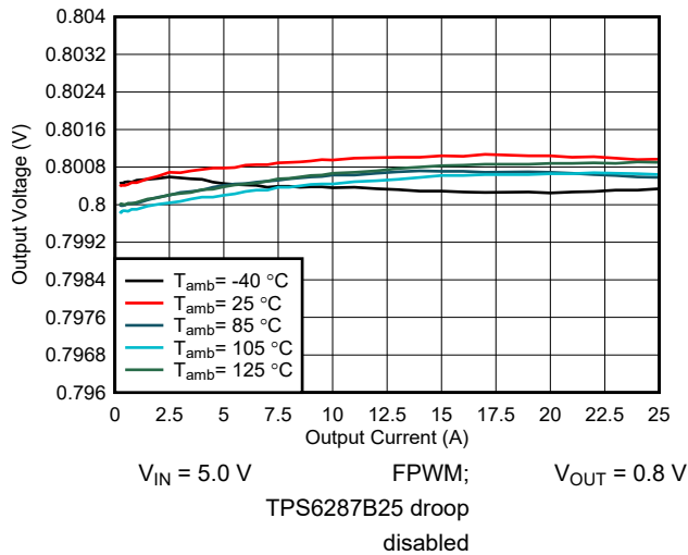
9-10. Output Voltage Versus Output Current
