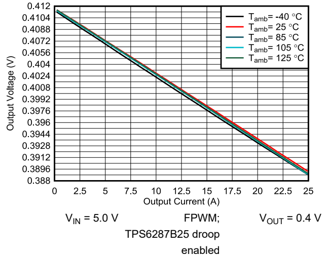
9-9. Output Voltage Versus Output Current
