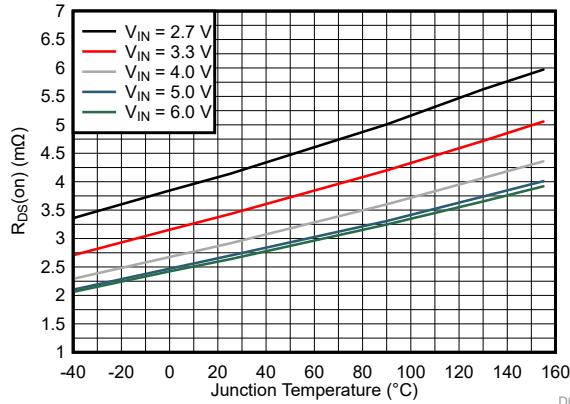
図 6-1. R_{DS(ON)} of High Side Switch
