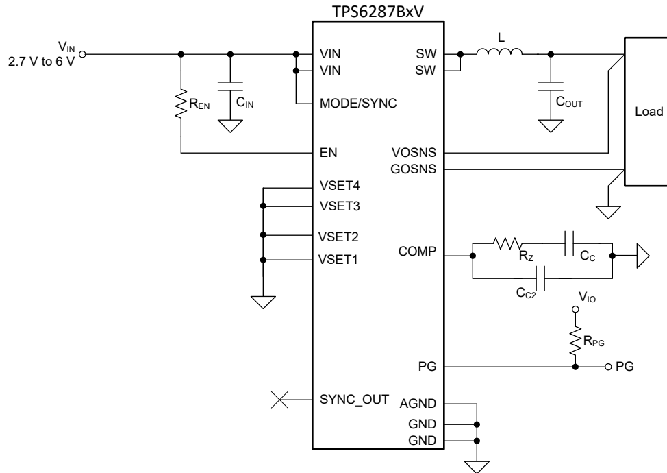
図 9-25. Typical Application Schematic for TPS6287BxV
