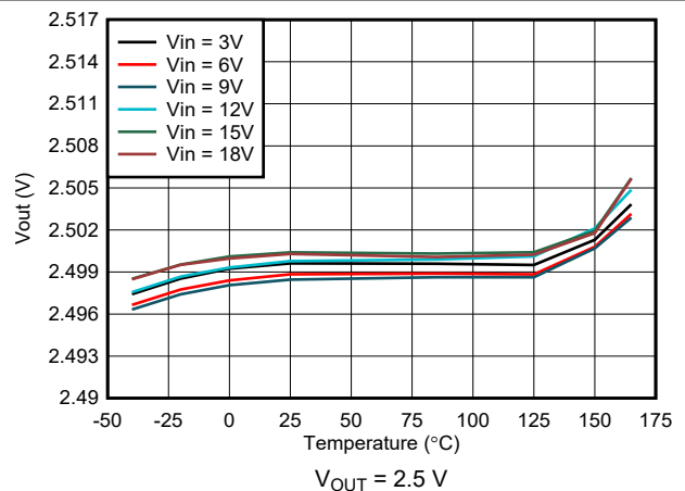
7-6. Output Voltage Accuracy - VSET Selected
