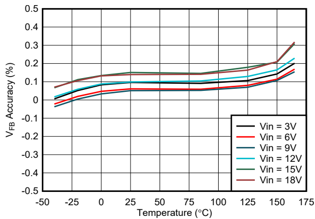
7-3. Feedback Voltage Accuracy - External Feedback Selected
