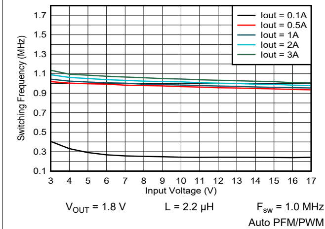
9-11. Switching Frequency vs Input Voltage
