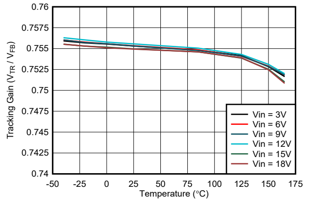
7-10. Tracking Voltage Gain vs Temperature
