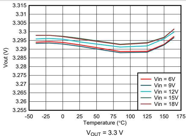
7-5. Output Voltage Accuracy - VSET Selected
