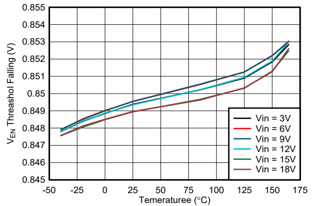
7-22. Precise EN Threshold vs Temperature
