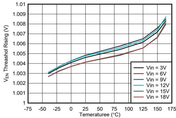
7-21. Precise EN Threshold vs Temperature
