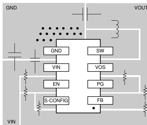
Figure 11-1. TPS629203-Q1 Layout
