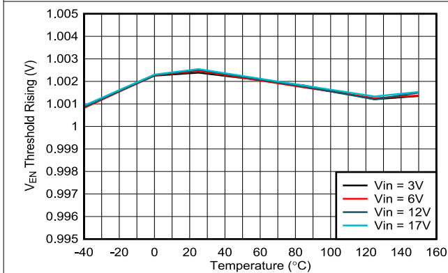
7-17. Precision Enable Threshold vs Temperature
