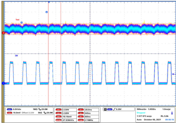
9-74. Output Voltage Ripple
