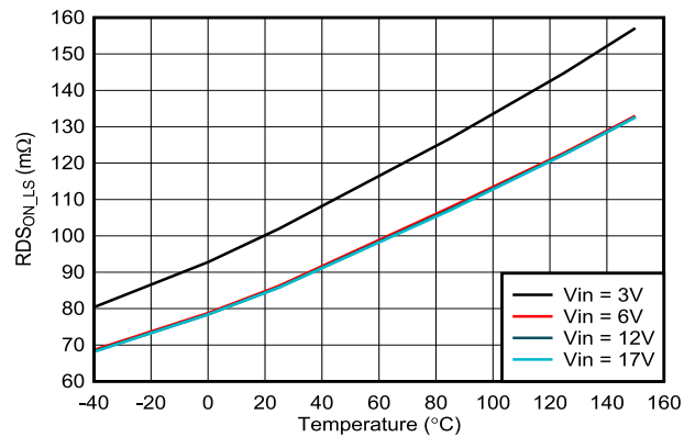
7-12. Low-Side R_{DS(ON)} vs Temperature
