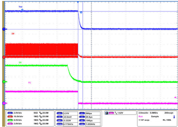
9-68. Shutdown Timing with Output Discharge Enabled
