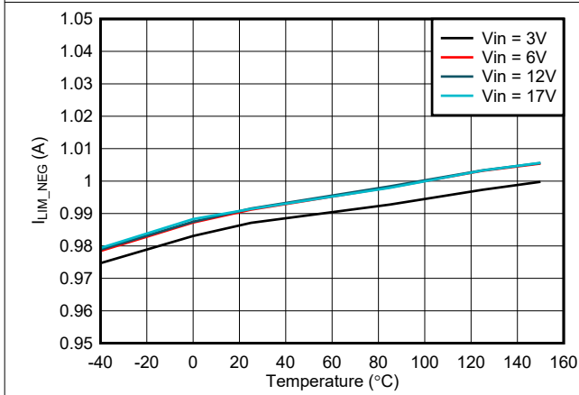
7-15. Low-Side I_{NEG} vs Temperature
