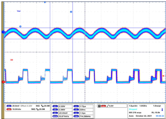
9-74. Output Voltage Ripple
