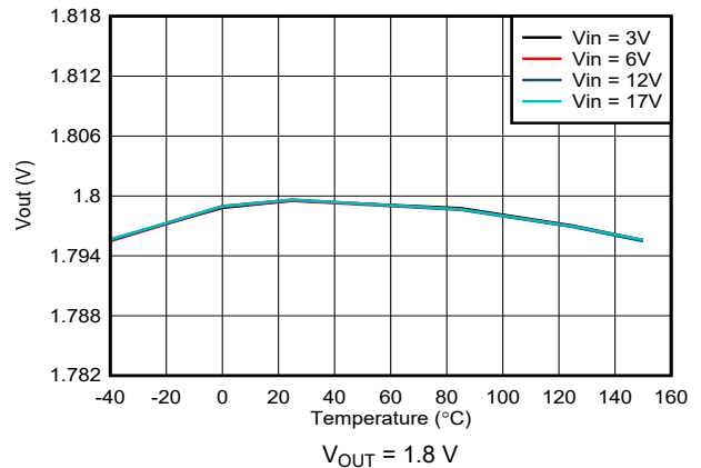
7-6. Output Voltage Accuracy – VSET Selected
