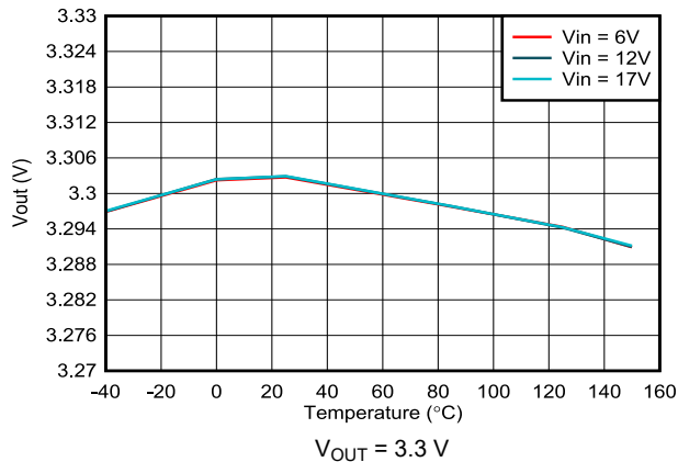
7-5. Output Voltage Accuracy – VSET Selected
