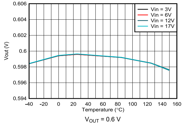
7-8. Output Voltage Accuracy – VSET Selected
