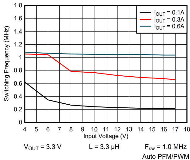
9-22. Switching Frequency vs Input Voltage
