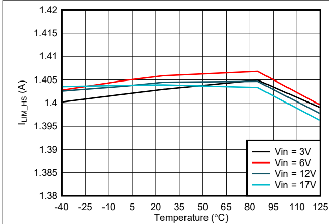
7-13. High-Side I_{LIM} vs Temperature
