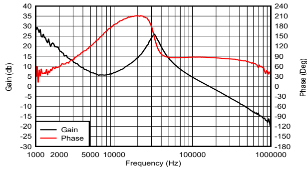
9-80. Bode Plot
