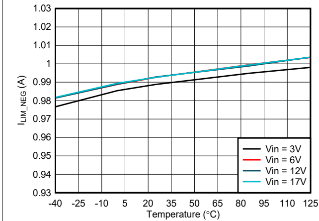
7-15. Low-Side I_{NEG} vs Temperature
