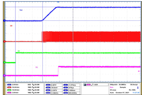
9-63. Start-Up Timing
