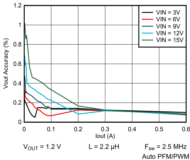
9-42. Output Voltage vs Output Current
