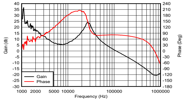
9-81. Bode Plot
