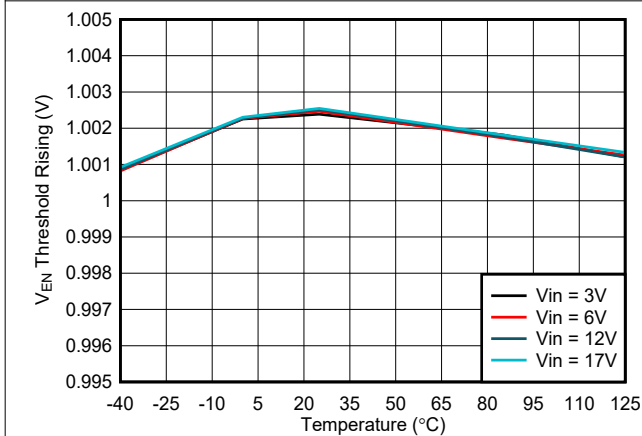
7-17. Precision Enable Threshold vs Temperature
