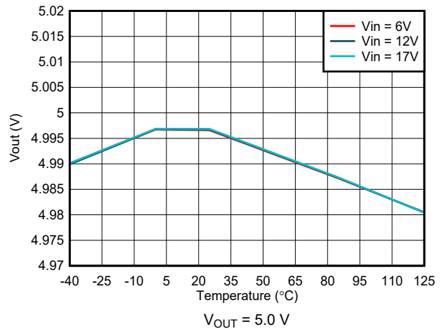
7-4. Output Voltage Accuracy – VSET Selected
