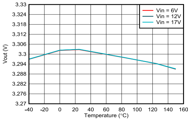
7-3. Output Voltage Accuracy – External Feedback
