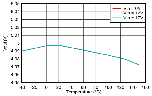
7-4. Output Voltage Accuracy – VSET Selected
