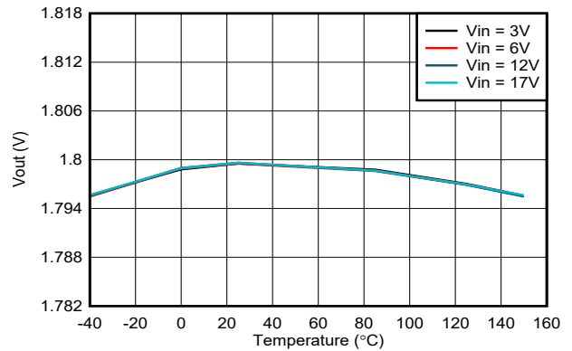
7-4. Output Voltage Accuracy – VSET Selected
