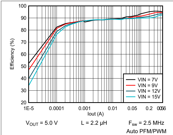
图 9-2. Efficiency vs Output Current
