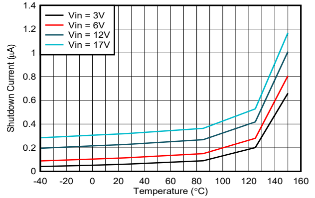
7-2. Typical Shutdown Current vs Temperature
