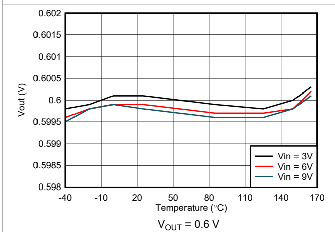
7-9. Output Voltage Accuracy - VSET Selected
