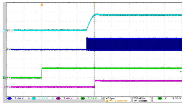
Figure 9-65. Start-Up Timing
