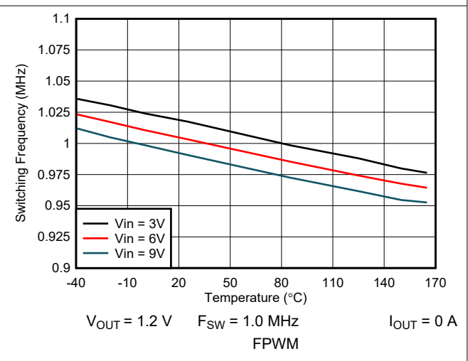
7-12. Switching Frequency vs Temperature
