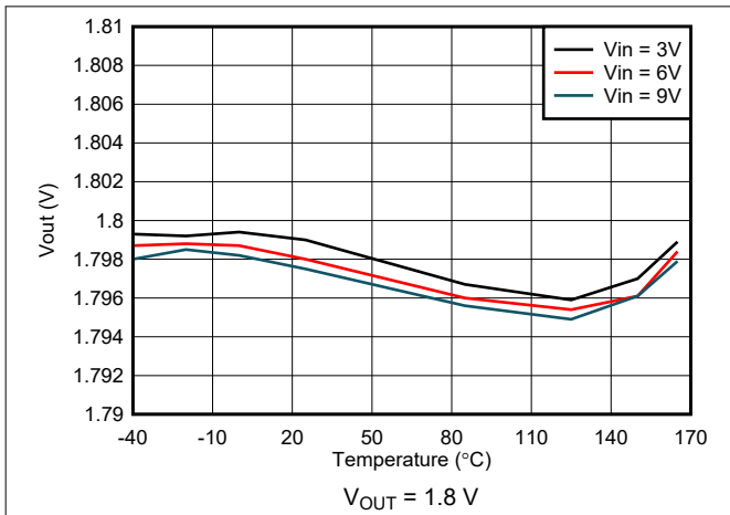
7-7. Output Voltage Accuracy - VSET Selected
