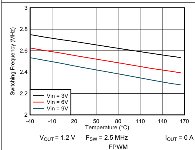
7-11. Switching Frequency vs Temperature
