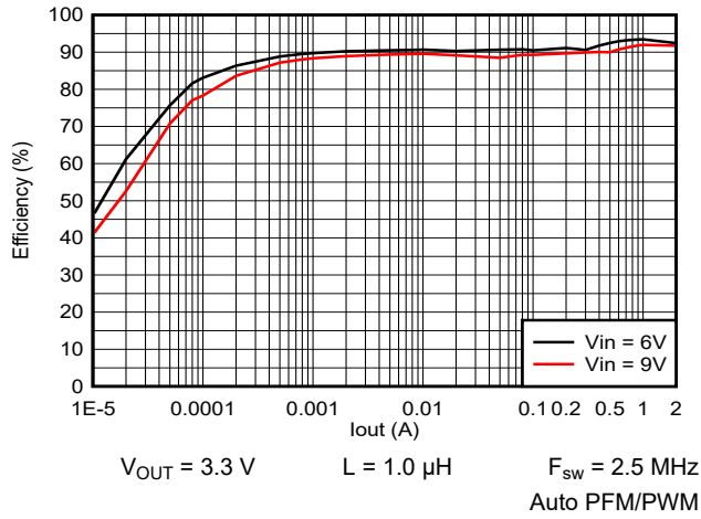
9-52. Efficiency vs Output Current
