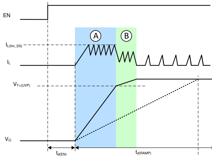
☒ 7-1. Typical Soft-Start Behavior
