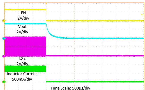
8-13. Shutdown by EN
