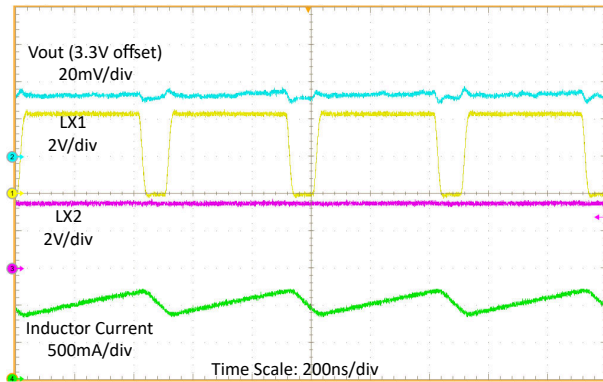
8-8. Switching Waveforms with 1A Load
