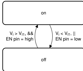
☒ 7-3. Device Functional Modes
