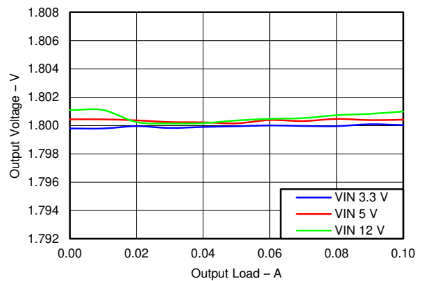
6-10. LDO2, Load Regulation
