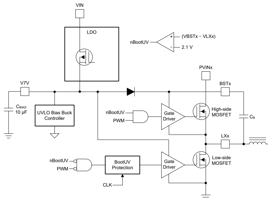
7-5. V7V Linear Dropout Regulator and Bootstrap Voltage Diagram
