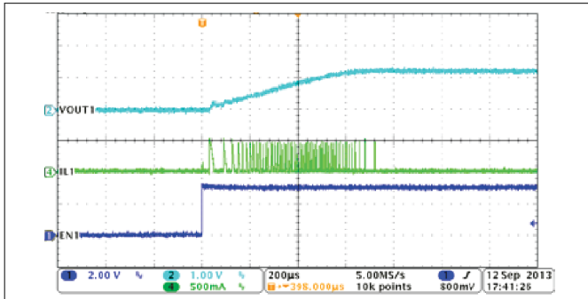
8-3. Buck1, Soft-Start With No Load
