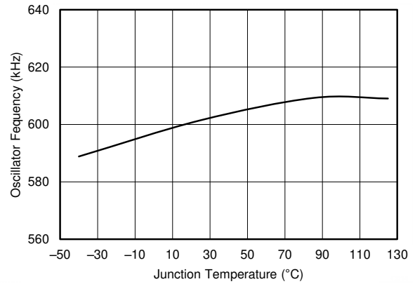
6-14. Oscillator Frequency vs Temperature
