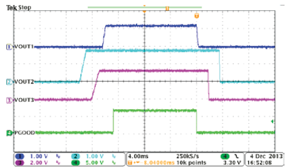
8-30. Automatic Power Sequencing, MODE = EN1 = HIGH, EN2 = LOW
