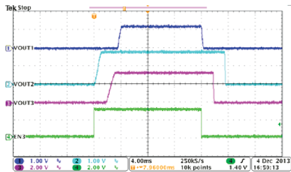
8-29. Automatic Power Sequencing, MODE = EN1 = HIGH, EN2 = LOW
