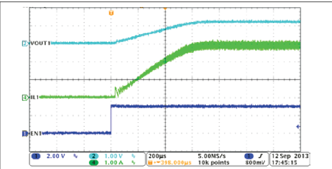
8-4. Buck1, Soft-Start With Full Load
