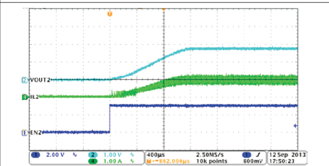
8-6. Buck2, Soft-Start With Full Load
