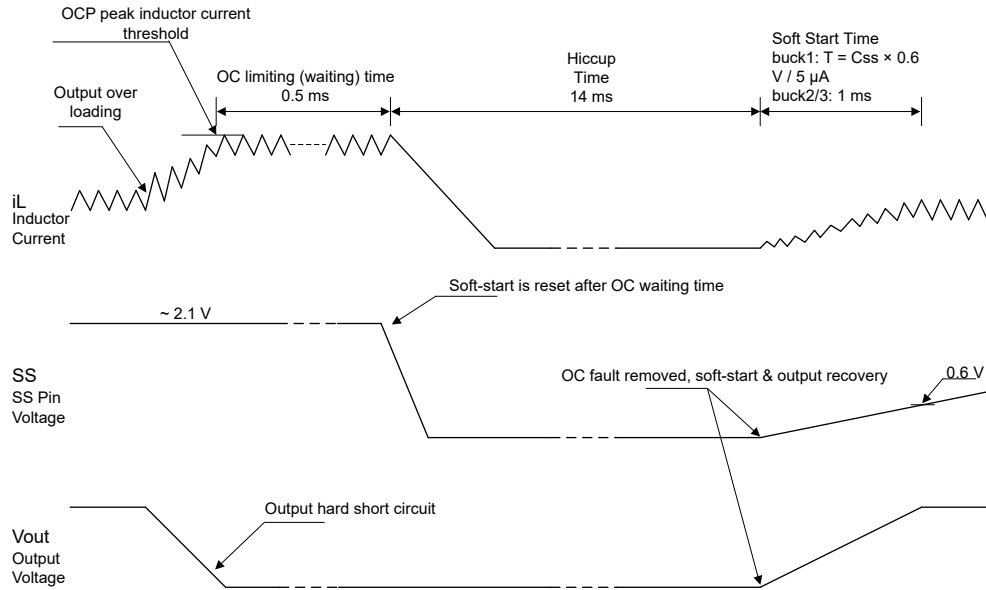
7-7. Overcurrent Protection
