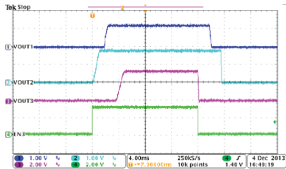
8-31. Automatic Power Sequencing, MODE = EN2 = HIGH, EN1 = LOW
