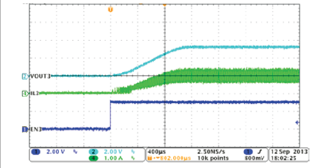
8-8. Buck3, Soft-Start With Full Load
