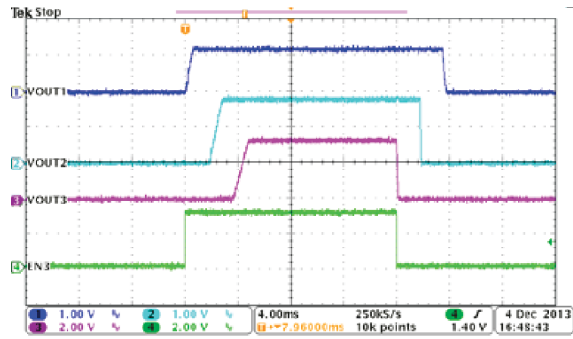
8-27. Automatic Power Sequencing, MODE = EN1 = EN2 = HIGH
