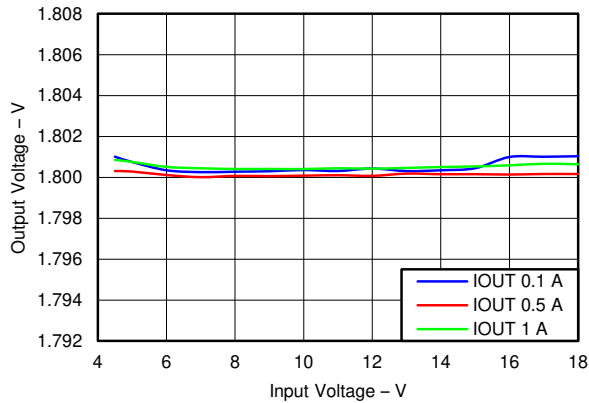
6-7. Buck2, Line Regulation
