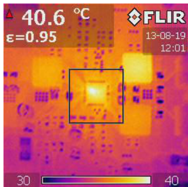
8-33. Thermal Signature of TPS65262EVM EVM Condition 4 Layers, 64 mm × 69 mm, T A = 30.5°C
