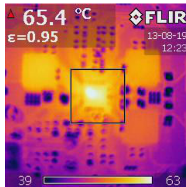
8-34. Thermal Signature of TPS65262EVM EVM Condition 4 Layers, 64 mm × 69 mm, T A = 30.5°C
