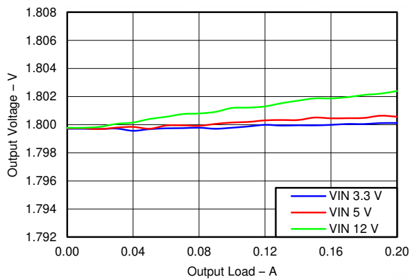
6-9. LDO1, Load Regulation
