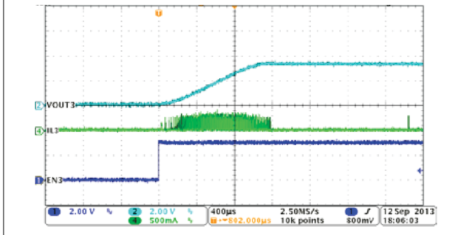
8-7. Buck3, Soft-Start With No Load
