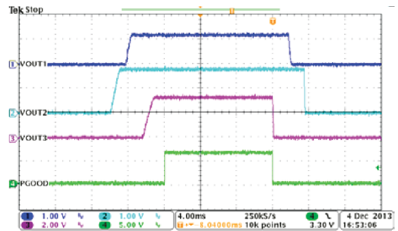
8-32. Automatic Power Sequencing, MODE = EN2 = HIGH, EN1 = LOW
