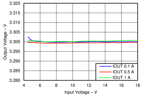
6-8. Buck3, Line Regulation
