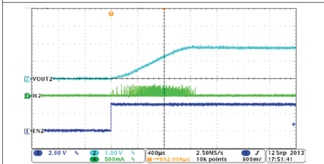
8-5. Buck2, Soft-Start With No Load
