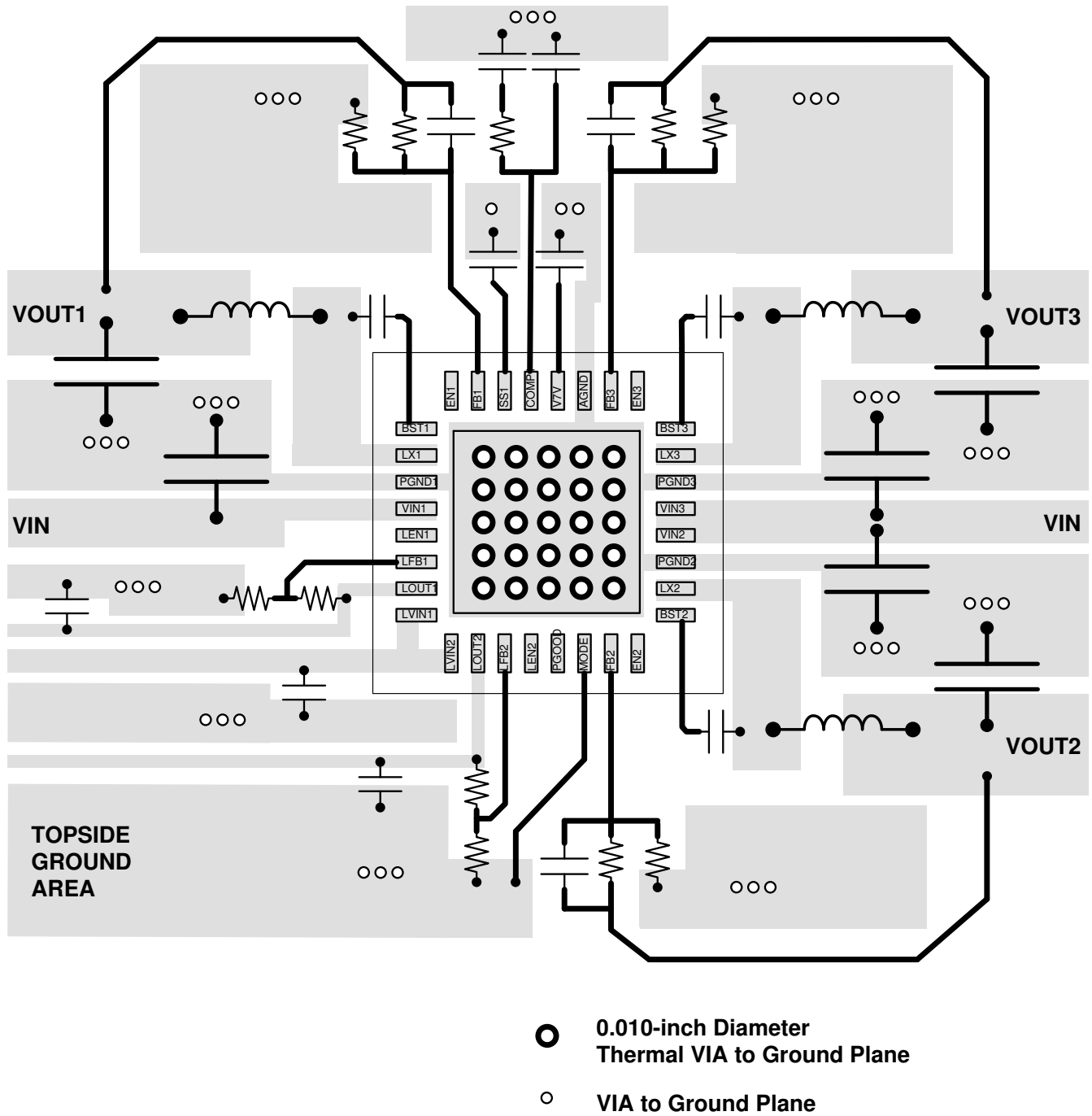
8-35. PCB Layout
