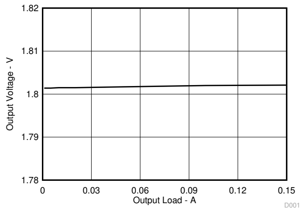
6-10. LDO2, Load Regulation, V_{IN} = 3.3\text{ V}
