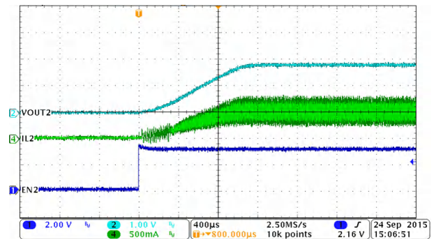
8-30. PWM Mode, Buck2, Soft-Start with Full Load
