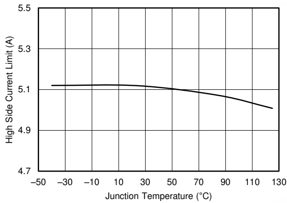
6-21. Buck1 High-Side Current Limit vs Temperature
