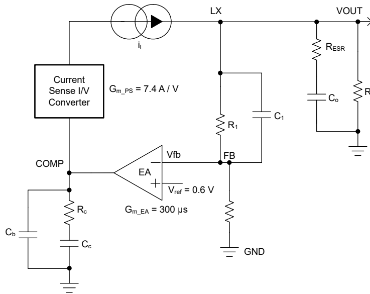
8-2. DC/DC Loop Compensation
