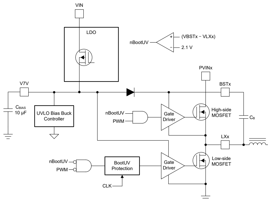
7-4. V7V Linear Dropout Regulator and Bootstrap Voltage Diagram
