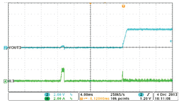
8-26. Buck3, Hiccup and Recovery
