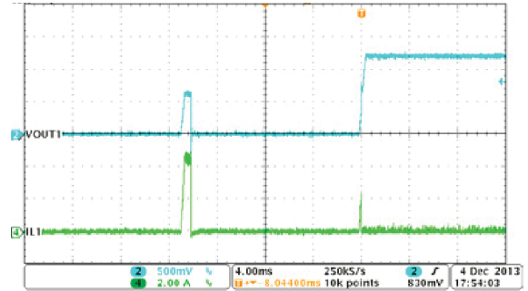
8-22. Buck1, Hiccup and Recovery
