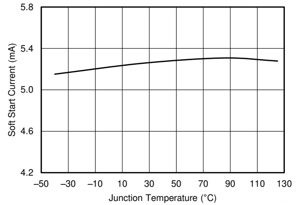
6-20. SS Pin Charge Current vs Temperature
