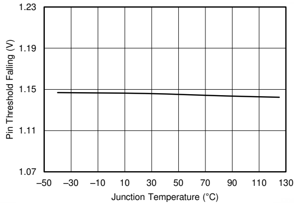
6-19. EN Pin Threshold Falling vs Temperature
