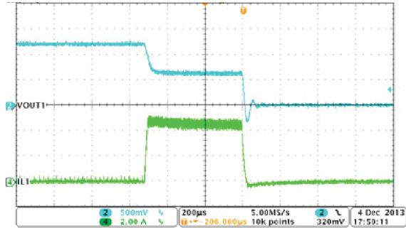
8-21. Buck1, Overcurrent Protection
