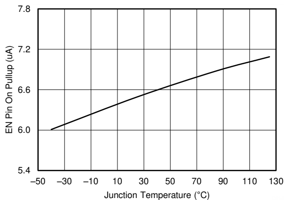
6-17. EN Pin Pullup Current vs Temperature, EN = 1.5 V
