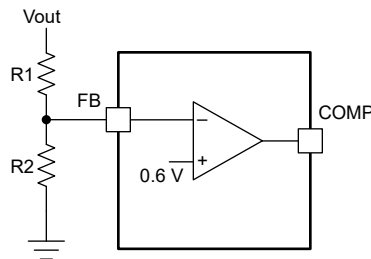
7-1. Voltage Divider Circuit
