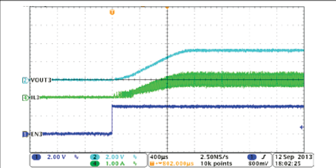
8-8. PSM Mode Buck3, Soft-Start with Full Load
