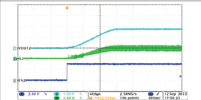
8-6. PSM Mode Buck2, Soft-Start with Full Load
