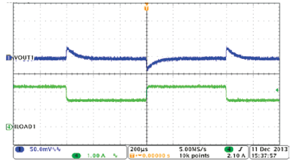
8-16. Buck1, Load Transient, 1.5 to 2.25 A SR = 0.25 A/µs
