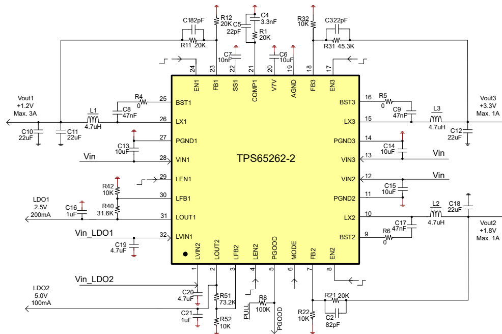
図 8-1. Typical Application Schematic
