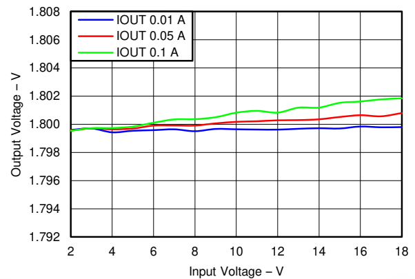
6-12. LDO2, Line Regulation
