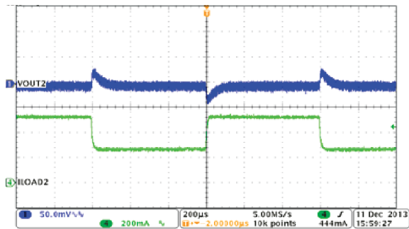
8-17. Buck2, Load Transient, 0.25 to 0.5 A SR = 0.25 A/µs
