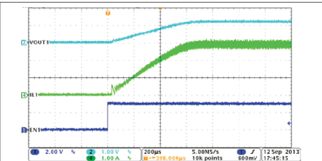
8-4. PSM Mode Buck1, Soft-Start With Full Load
