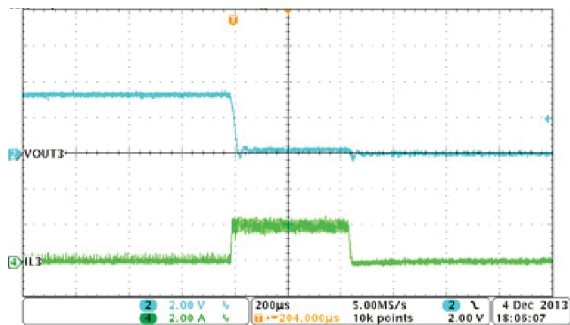
8-25. Buck3, Overcurrent Protection
