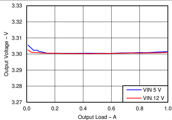
6-5. Buck3, PSM Mode Load Regulation
