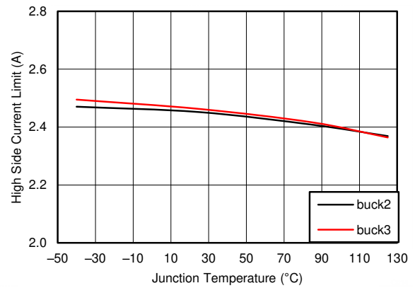
6-22. Buck2, 3 High-Side Current Limit vs Temperature
