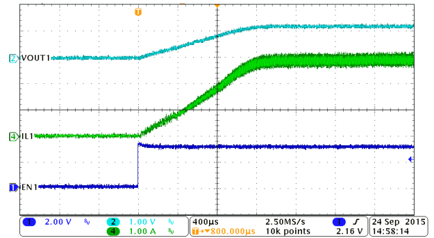
8-28. PWM Mode, Buck1, Soft-Start with Full Load
