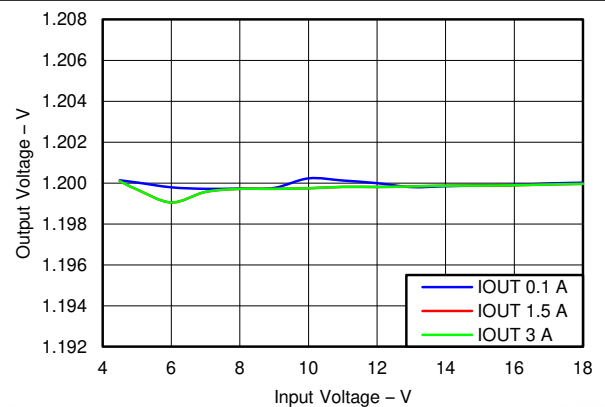
6-6. Buck1, PSM Mode Line Regulation
