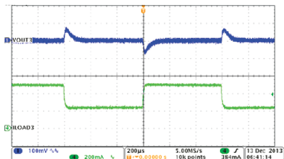
8-19. Buck3, Load Transient, 0.25 to 0.5 A SR = 0.25 A/µs
