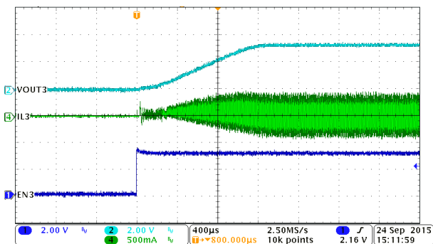
8-31. PWM Mode, Buck3, Soft-Start with No Load
