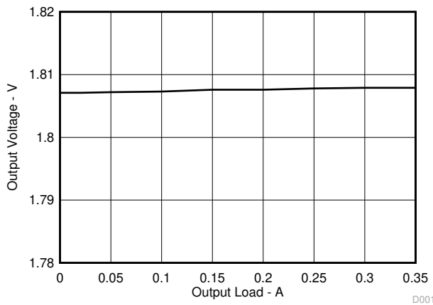
6-9. LDO1, Load Regulation, V_{IN} = 3.3\text{ V}
