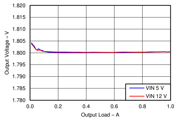
6-4. Buck2, PSM Mode Load Regulation
