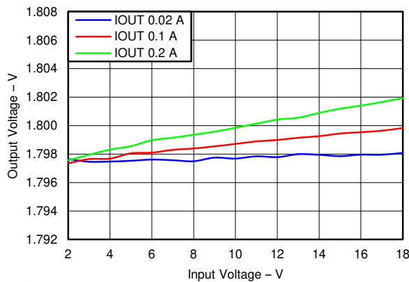
6-11. LDO1, Line Regulation
