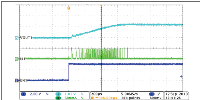
8-3. PSM Mode Buck1, Soft-Start with No Load
