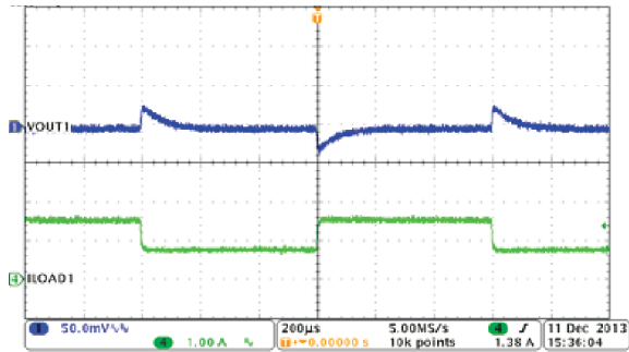
8-15. Buck1, Load Transient, 0.75 to 1.5 A SR = 0.25 A/µs
