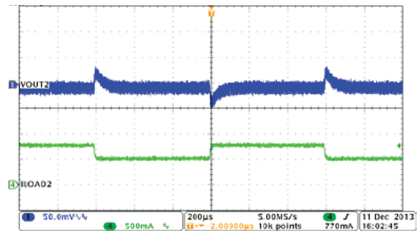
8-18. Buck2, Load Transient, 0.5 to 0.75 A SR = 0.25A/µs
