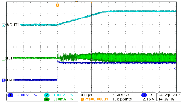
8-27. PWM Mode, Buck1, Soft-Start with No Load
