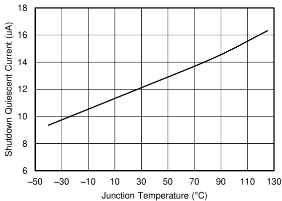
6-15. Shutdown Quiescent Current vs Temperature
