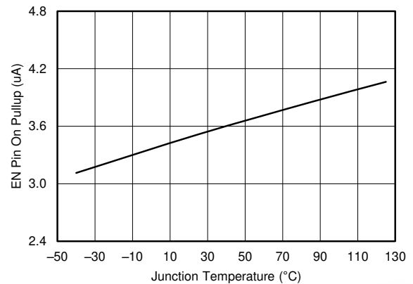
6-16. EN Pin Pullup Current vs Temperature, EN = 1 V
