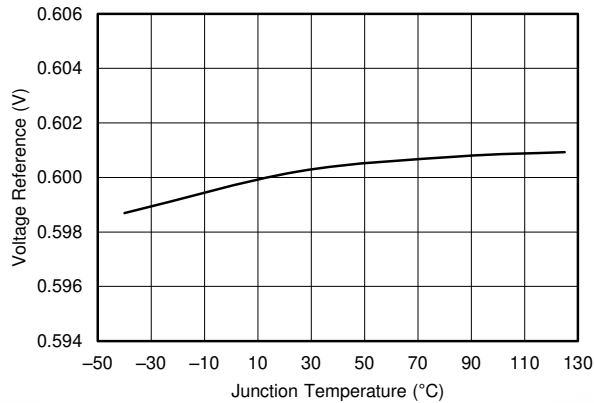
6-13. Voltage Reference vs Temperature
