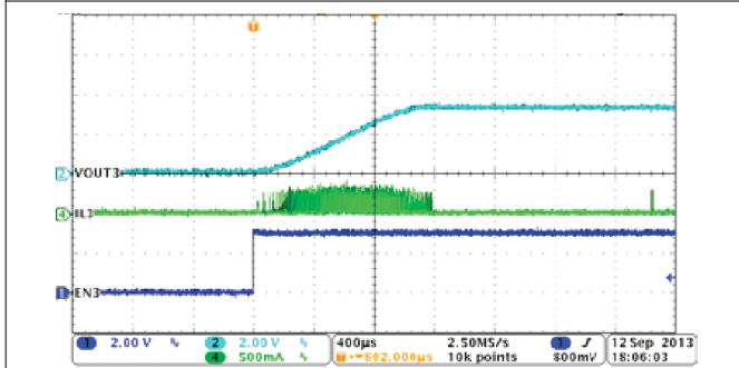
8-7. PSM Mode Buck3, Soft-Start With No Load
