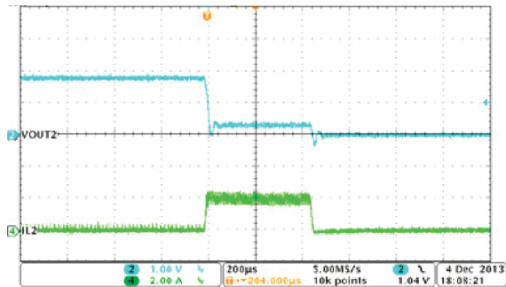
8-23. Buck2, Overcurrent Protection
