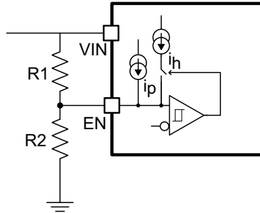
☒ 7-2. Adjustable VIN Undervoltage Lockout
