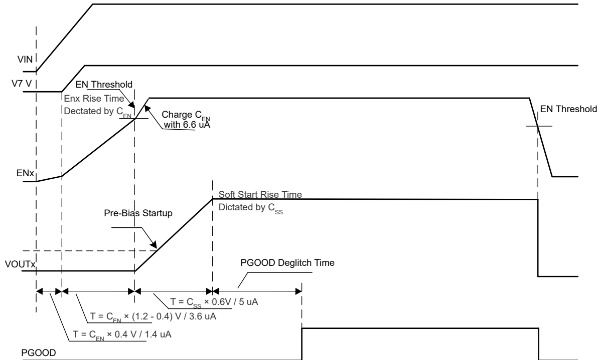
7-3. Startup Power Sequence
