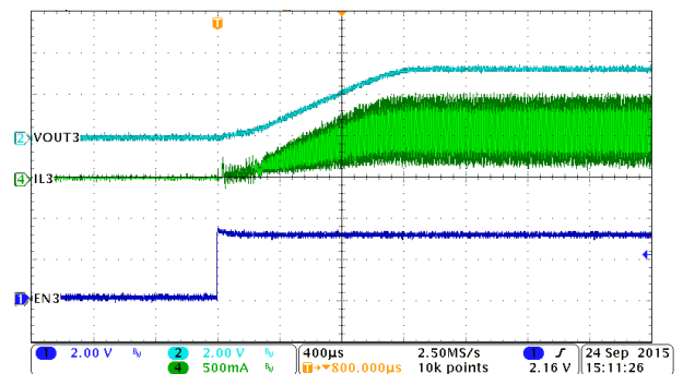
8-32. PWM Mode, Buck3, Soft-Start with Full Load
