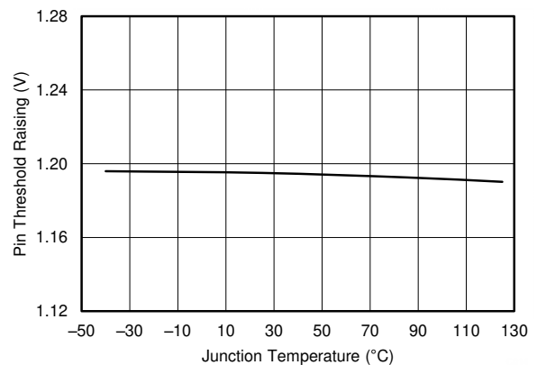
6-18. EN Pin Threshold Rising vs Temperature
