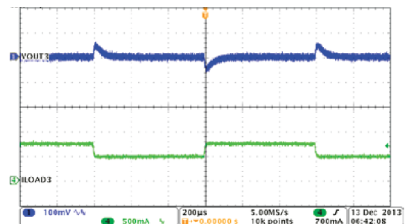
8-20. Buck3, Load Transient, 0.5 to 0.75 A SR = 0.25A/µs
