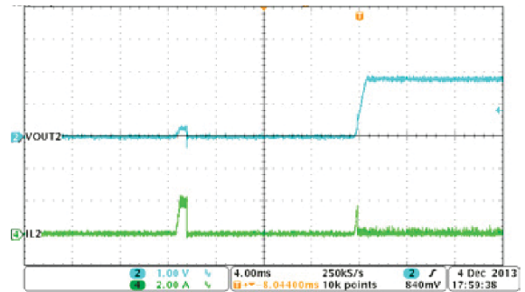
8-24. Buck2, Hiccup and Recovery
