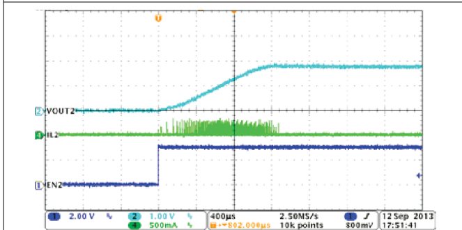
8-5. PSM Mode Buck2, Soft-Start with No Load
