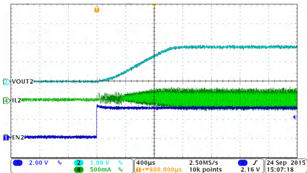
8-29. PWM Mode, Buck2, Soft-Start with No Load
