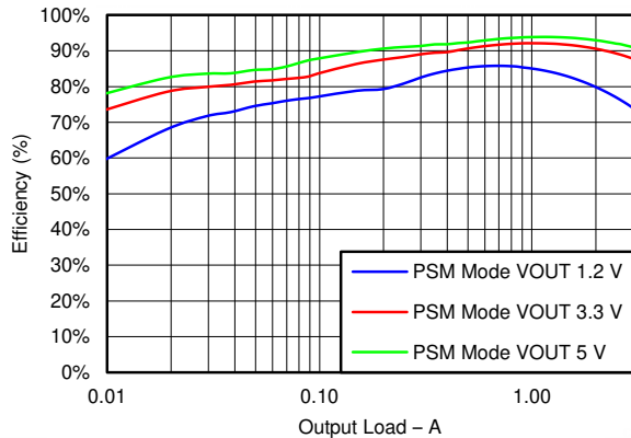
6-1. Buck1 Efficiency
