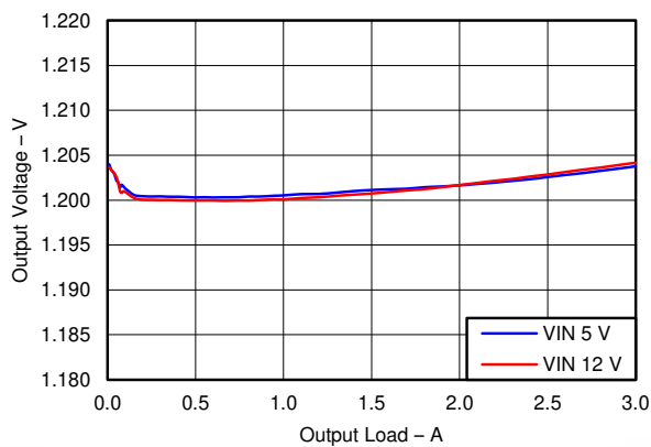
6-3. Buck1, PSM Mode Load Regulation
