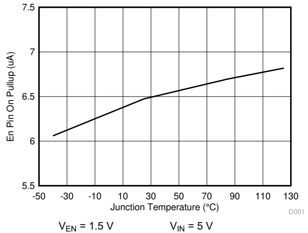
6-14. EN Pin Pullup Current vs Temperature
