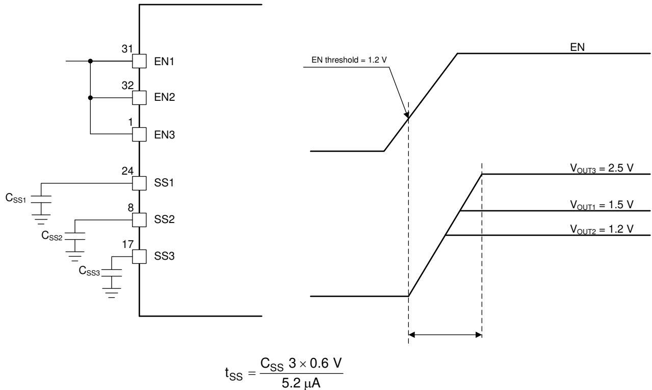
7-6. Simultaneous Startup Sequence Using SSx Pins
