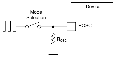
図 7-11. Works With Resistor Mode and Synchronization Mode
