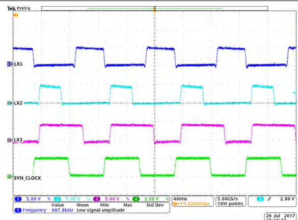
8-20. Synchronization With External Clock
