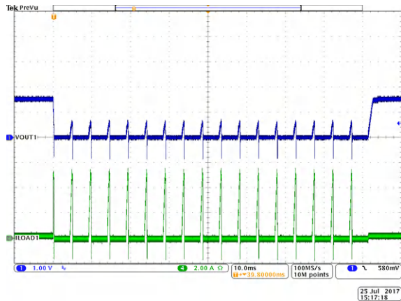
8-15. BUCK1 Hiccup and Recovery
