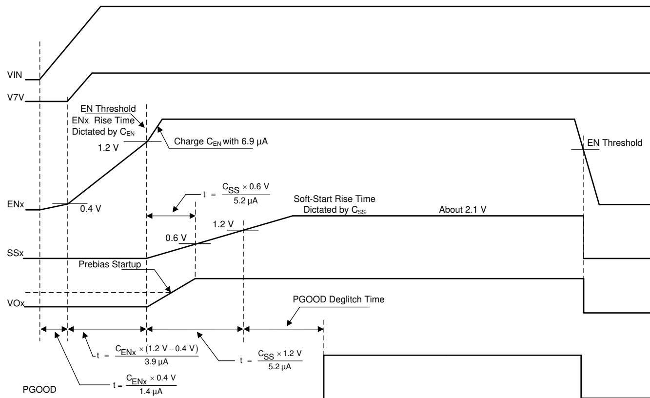
7-7. Startup Power Sequence
