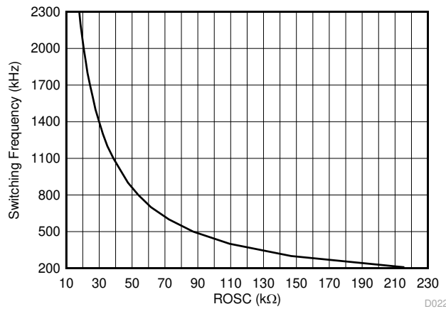
図 7-10. ROSC vs Switching Frequency
