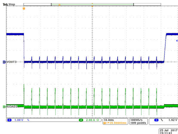
8-17. BUCK3 Hiccup and Recovery
