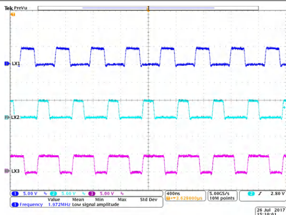
8-19. 180° Out-of-Phase
