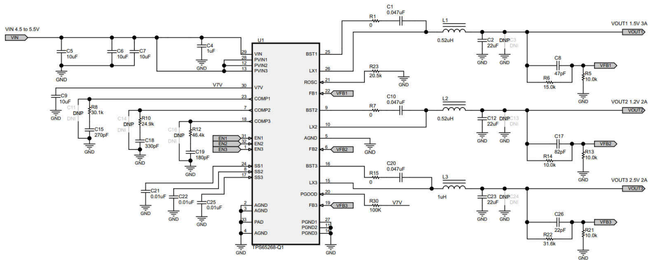
図 8-1. Typical Application Schematic
