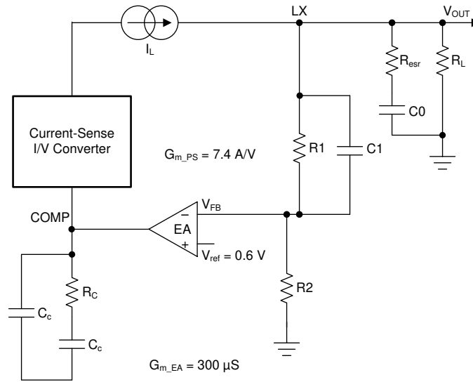
8-2. DC-DC Loop Compensation
