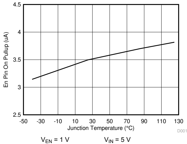
6-13. EN Pin Pullup Current vs Temperature
