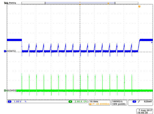
8-16. BUCK2 Hiccup and Recovery
