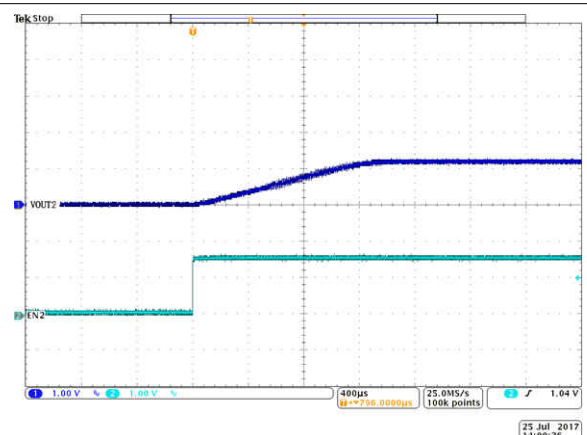
8-4. BUCK2 Soft-Start
