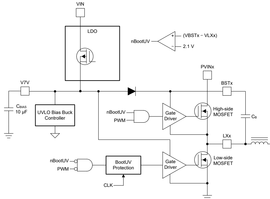
7-8. V7V Linear Dropout Regulator and Bootstrap Voltage Diagram
