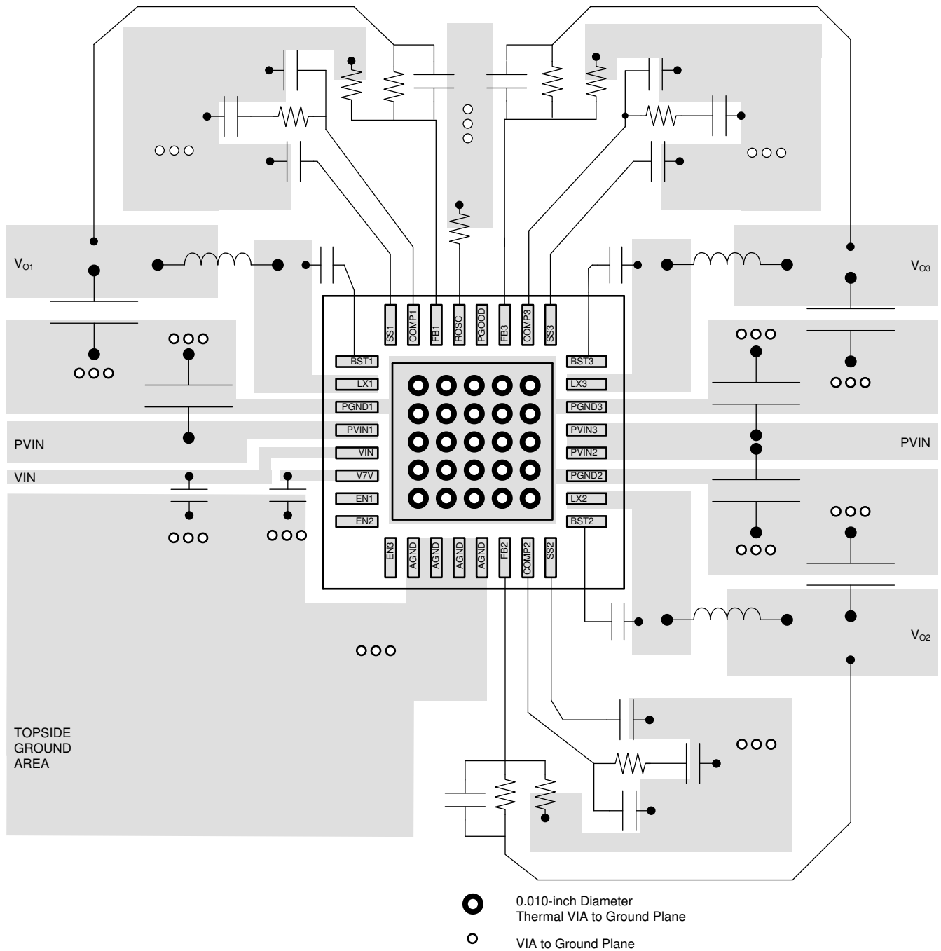
8-22. PCB Layout
