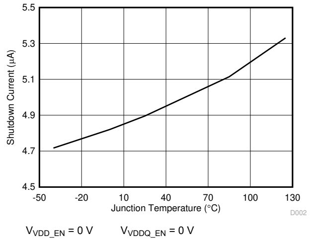
Fig 6-2. VCC_5V Shutdown Current vs Temperature
