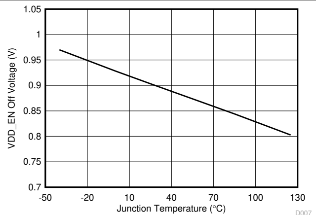
Fig 6-6. Enable Off Voltage (VDD_EN) vs Junction Temperature
