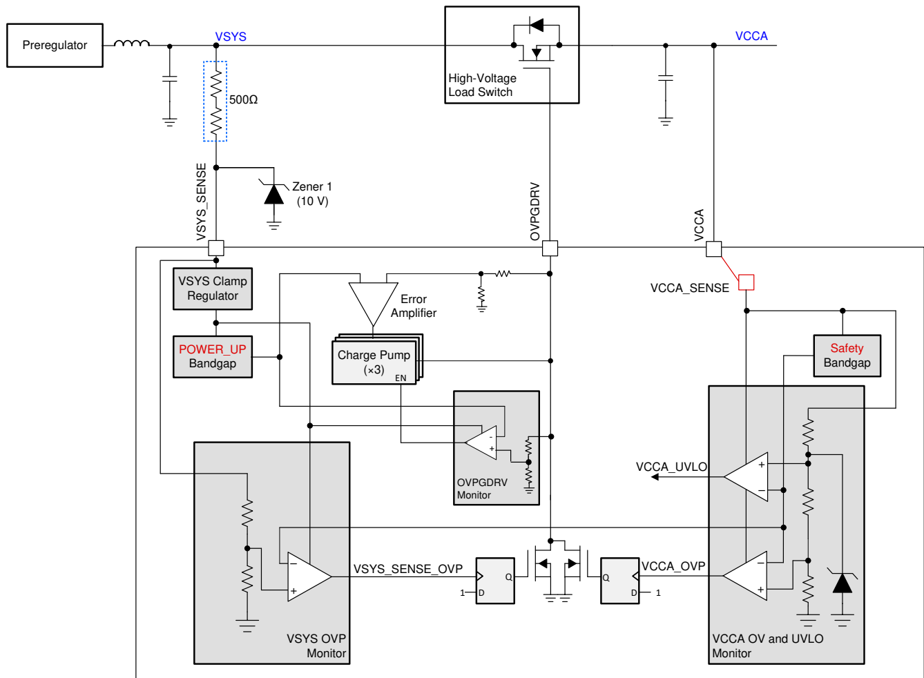
Figure 8-1. VSYS Monitor and OVP/UVLO Output Generation
