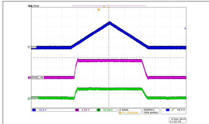
8-5. TPS71533-Q1 Power-Up and Power-Down Waveform for Legacy Chip
