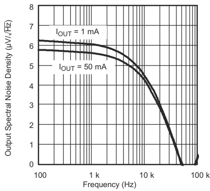
6-7. Output Spectral Noise Density vs Frequency for Legacy Chip
