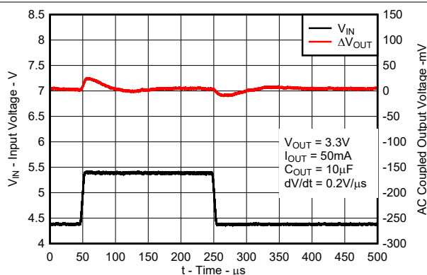
5-27. Fast Power-Up (New Chip)
