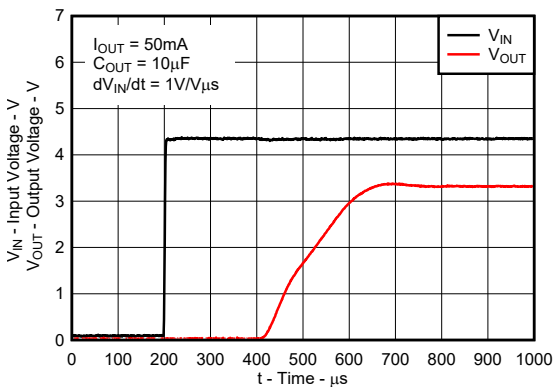
5-25. Power-Up, Power-Down (New Chip)
