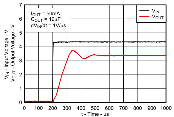
5-26. Fast Power-Up (Legacy Chip)
