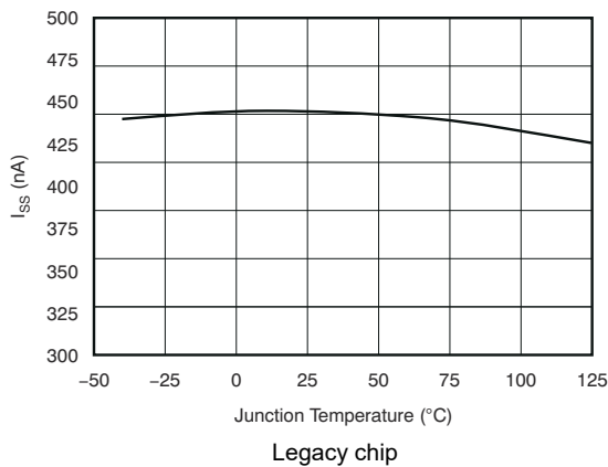
5-23. Soft-Start Charging Current ( I_{SS} ) vs Temperature ( T_J )
