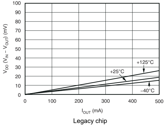
5-9. Dropout Voltage vs I_{OUT} and Temperature ( T_J )
