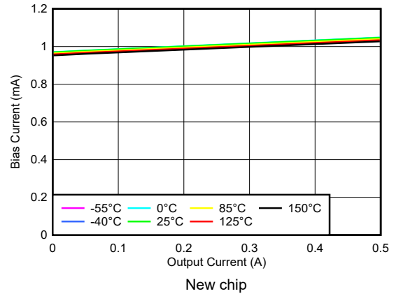
5-20. BIAS Pin Current vs Output Current and Temperature ( T_J )
