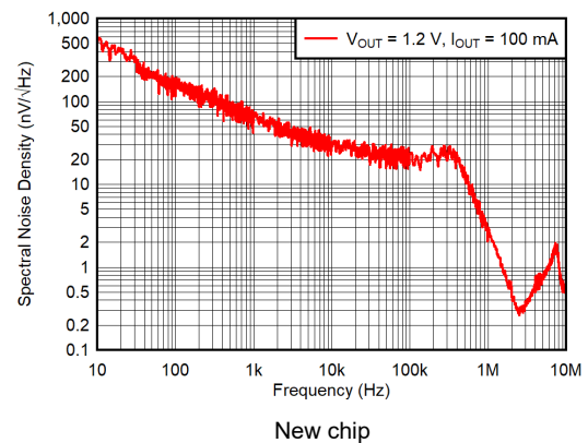
5-18. Noise Spectral Density
