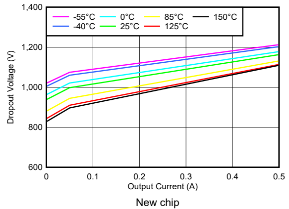
5-12. V_{BIAS} Dropout Voltage vs I_{OUT} and Temperature ( T_J )
