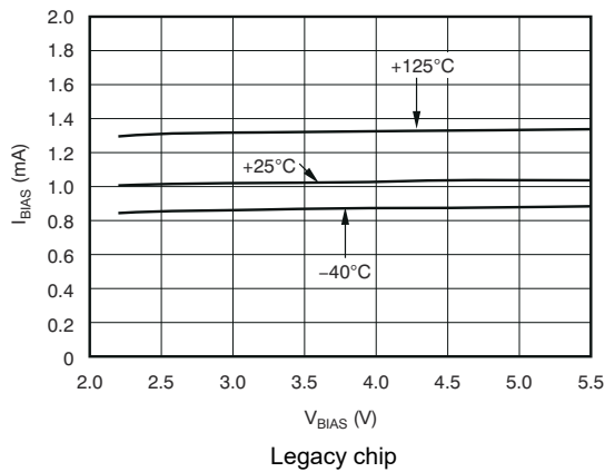
5-21. BIAS Pin Current vs V_{BIAS} and Temperature ( T_J )
