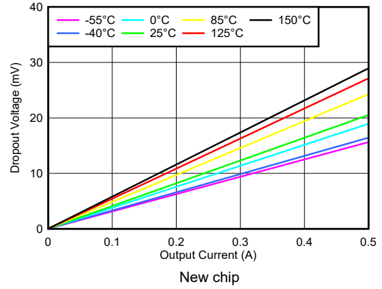
5-10. V_{IN} Dropout Voltage vs I_{OUT} and Temperature ( T_J )
