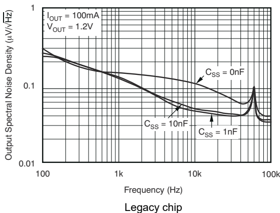
5-17. Noise Spectral Density
