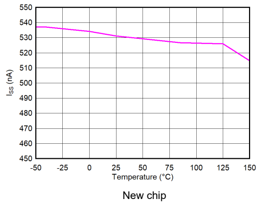
5-24. Soft-Start Charging Current ( I_{SS} ) vs Temperature ( T_J )
