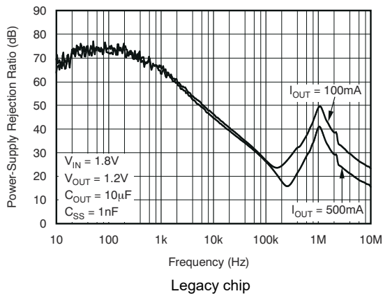
5-15. V_{IN} PSRR vs Frequency
