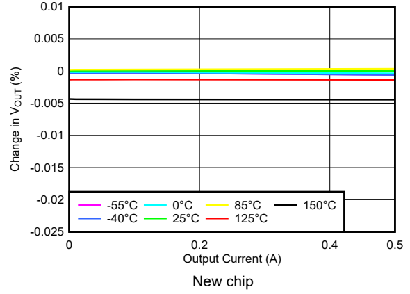
5-8. Load Regulation
