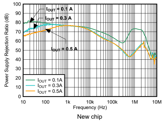
5-16. V_{IN} PSRR vs Frequency
