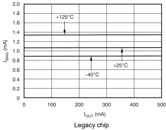
5-19. BIAS Pin Current vs I_{OUT} and Temperature ( T_J )
