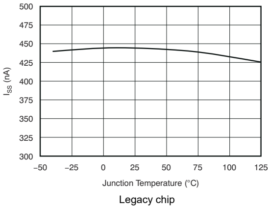
5-27. Soft-Start Charging Current ( I_{SS} ) vs Temperature ( T_J )
