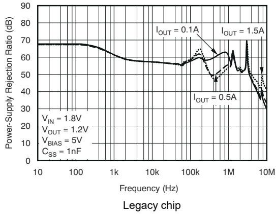
5-15. V_{BIAS} PSRR vs Frequency
