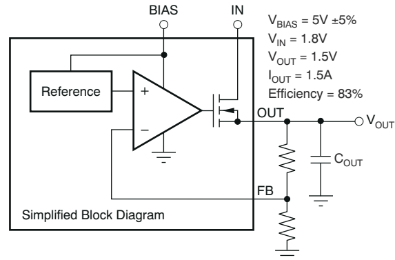
☒ 7-2. Typical Application of the TPS748 Using an Auxiliary Bias Rail
