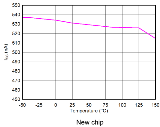
5-28. Soft-Start Charging Current ( I_{SS} ) vs Temperature ( T_J )
