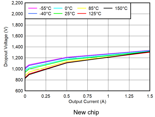
5-14. V_{BIAS} Dropout Voltage vs I_{OUT} and Temperature ( T_J )
