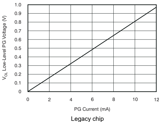
5-29. Low-Level PG Voltage vs Current
