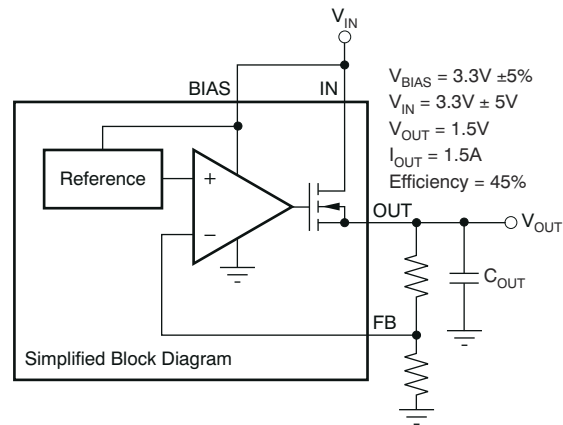
☒ 7-8. Typical Application of the TPS748 Without an Auxiliary Bias Rail
