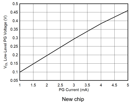
5-30. Low-Level PG Voltage vs Current
