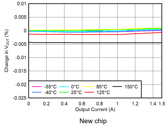
5-8. Load Regulation
