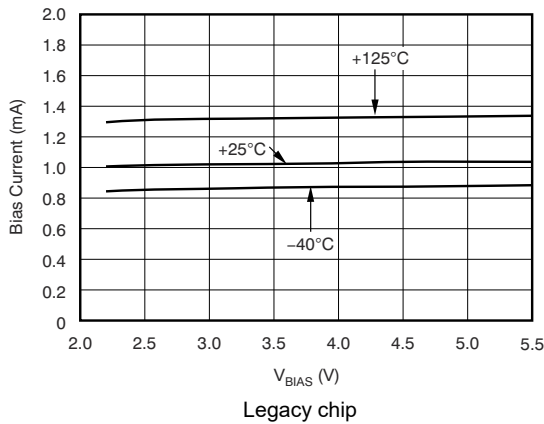
5-25. BIAS Pin Current vs V_{BIAS} and Temperature ( T_J )
