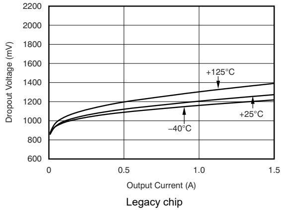
5-13. V_{BIAS} Dropout Voltage vs I_{OUT} and Temperature ( T_J )
