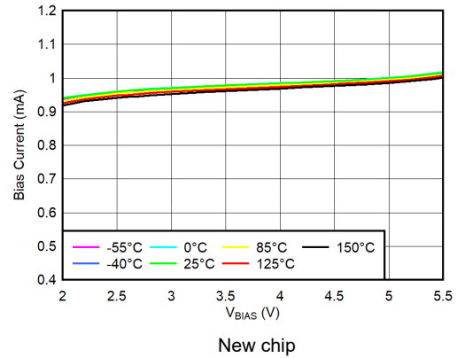
5-26. BIAS Pin Current vs V_{BIAS} and Temperature ( T_J )
