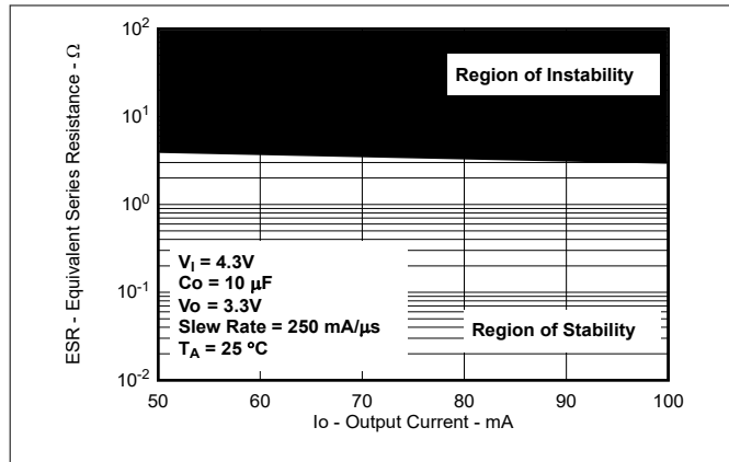
5-58. Typical Region of Stability ESR vs Output Current (New Chip)
