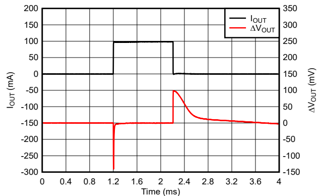
7-13. TPS76933-Q1 Load Transient Response (Legacy Chip)
