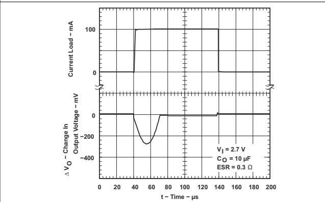
7-9. TPS76915-Q1 Load Transient Response (Legacy Chip)
