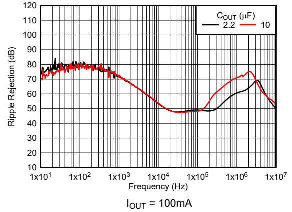
5-32. TPS76933-Q1 Ripple Rejection vs Output Capacitor (New Chip)
