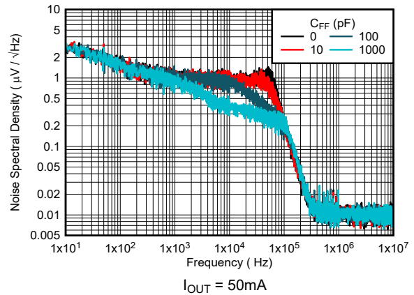
5-24. TPS76901-Q1 Output Spectral Noise Density vs Feed-Forward Capacitor (New Chip)
