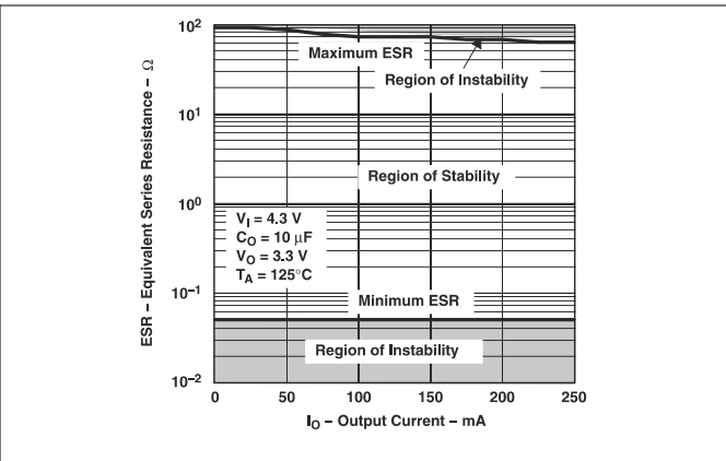
5-59. Typical Region of Stability ESR vs Output Current (Legacy Chip)
