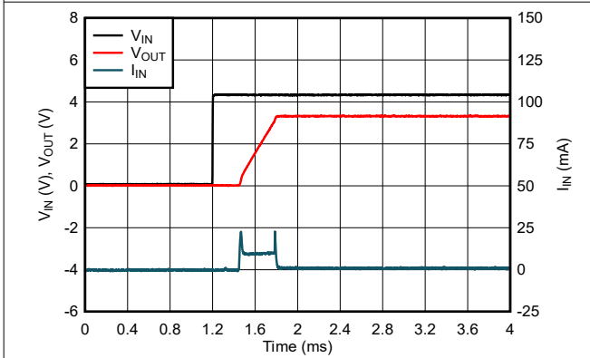
7-4. Power-Up Waveform (Legacy Chip)
