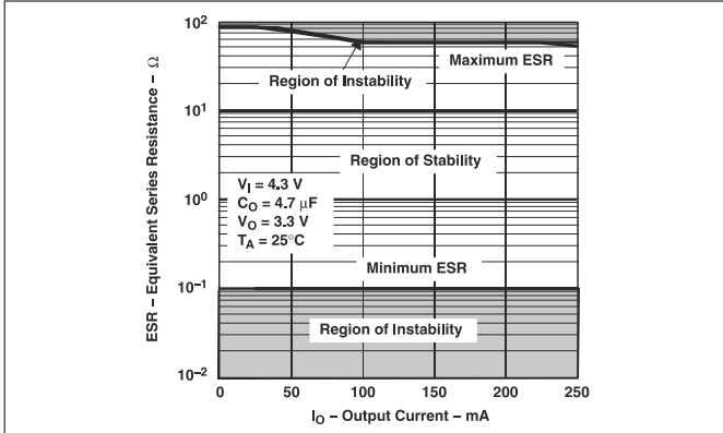
5-52. Typical Region of Stability ESR vs Output Current (Legacy Chip)
