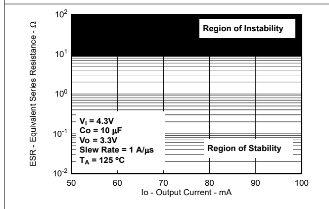
5-60. Typical Region of Stability ESR vs Output Current (New Chip)
