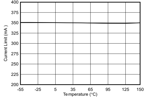
5-20. TPS76933-Q1 Current Limit vs Free-Air Temperature (New Chip)
