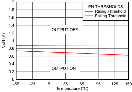
5-19. TPS76933-Q1 EN Threshold vs Free-Air Temperature (New Chip)
