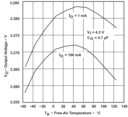
5-8. TPS76933-Q1 Output Voltage vs Free-Air Temperature (Legacy Chip)
