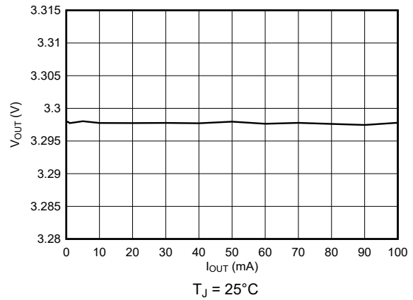
☒ 5-4. TPS76933-Q1 Output Voltage vs Output Current (New Chip)
