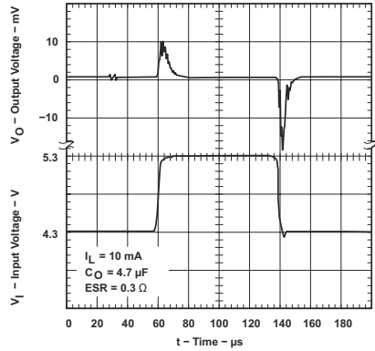
7-10. TPS76933-Q1 Line Transient Response (Legacy Chip)
