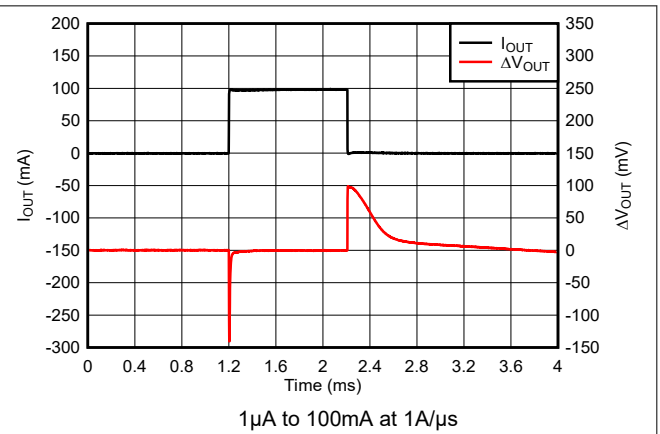
图 5-44. TPS76933-Q1 Load Transient Response (New Chip)
