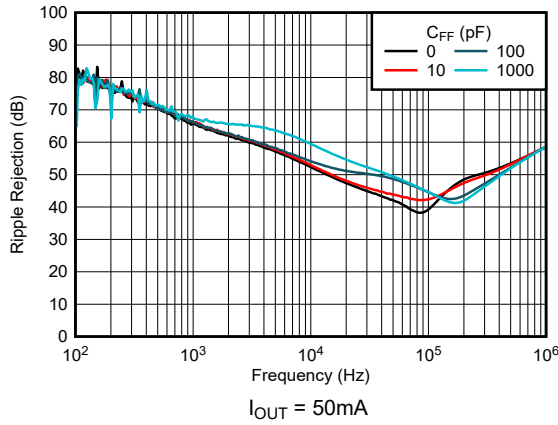
5-33. TPS76901-Q1 Ripple Rejection vs Feed-Forward Capacitor (New Chip)
