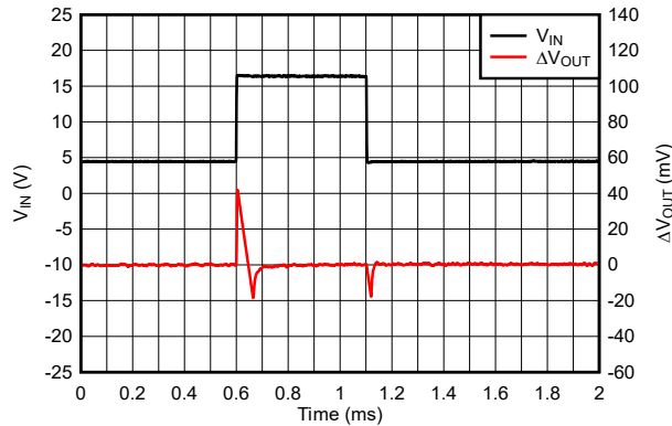
7-10. TPS76933-Q1 Line Transient Response (Legacy Chip)
