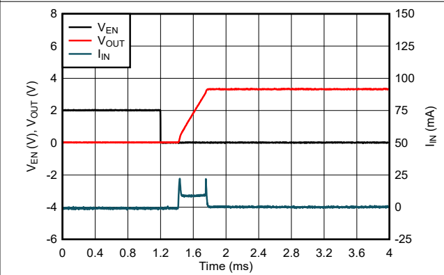
7-5. Power-Down Waveform (Legacy Chip)
