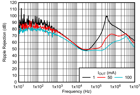
5-31. TPS76933-Q1 Ripple Rejection vs Output Current (New Chip)
