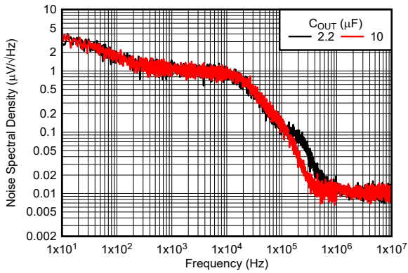
5-21. TPS76933-Q1 Output Spectral Noise Density vs Frequency (Legacy Chip)
