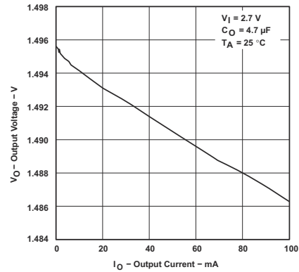
☒ 5-2. TPS76915-Q1 Output Voltage vs Output Current (Legacy Chip)
