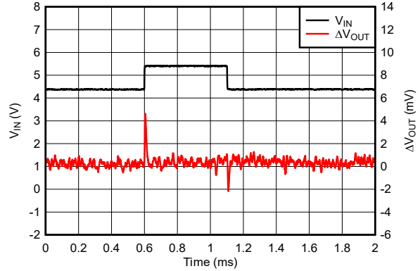
7-11. TPS76933-Q1 Line Transient Response (New Chip)
