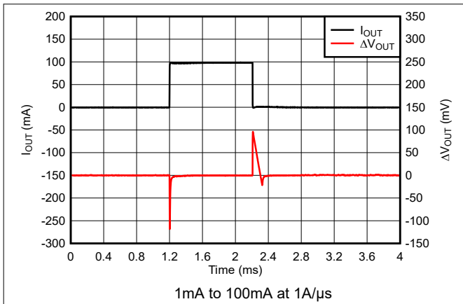
图 5-43. TPS76933-Q1 Load Transient Response (New Chip)
