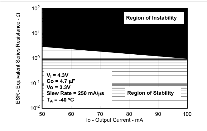
5-63. Typical Region of Stability ESR vs Output Current (Legacy Chip)
