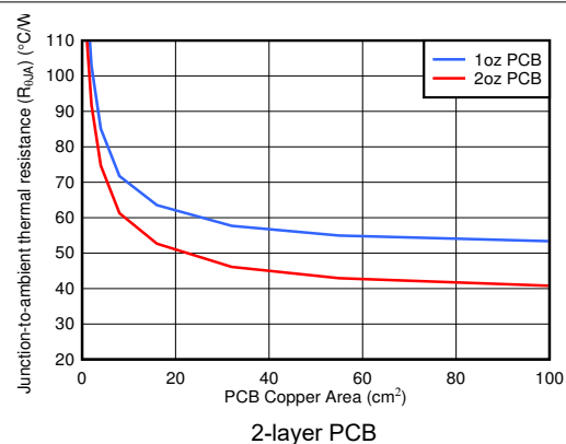
10-2. Junction-to-Ambient Thermal Resistance ( R_{\theta JA} ) vs PCB Copper Area (DRB Package)
