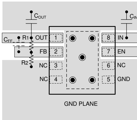
10-7. Layout Example for the DRB Package Adjustable Version
