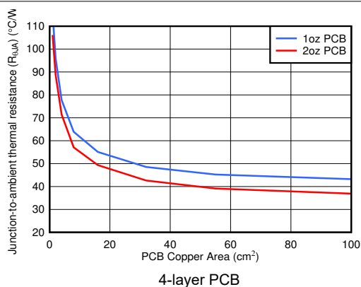
10-1. Junction-to-Ambient Thermal Resistance ( R_{\theta JA} ) vs PCB Copper Area (DRB Package)
