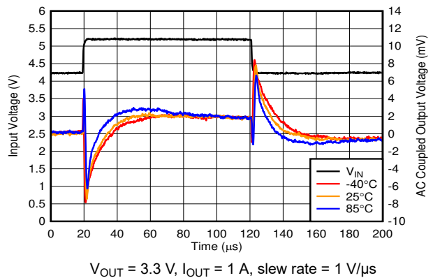
6-18. Line Transient vs Temperature
