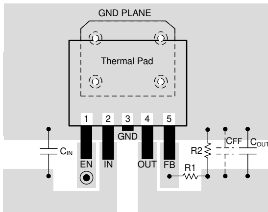
10-7. Layout Example for the DRB Package Adjustable Version
