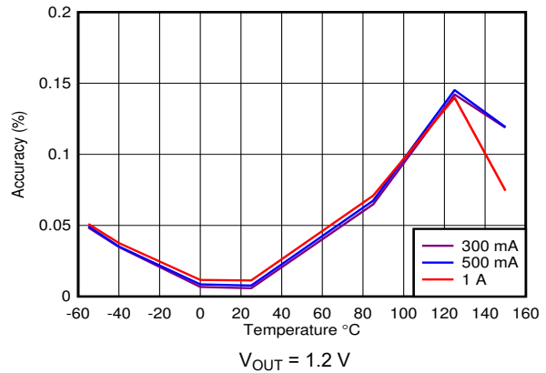
6-4. Output Accuracy vs Temperature
