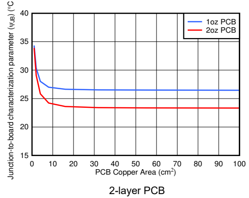
10-4. Junction-to-Board Characterization Parameter ( \psi_{JB} ) vs PCB Copper Area (DRB Package)
