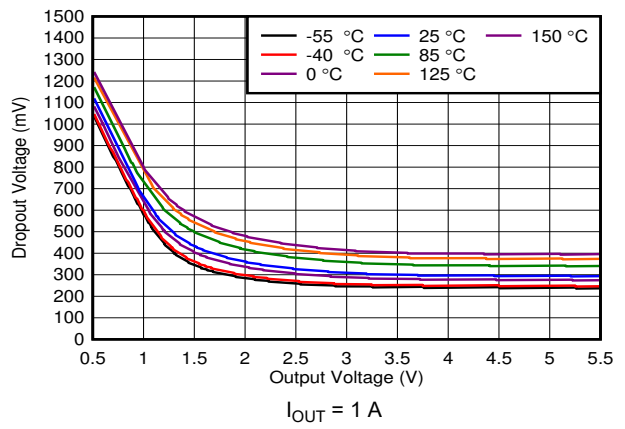
6-6. Dropout vs Output Voltage
