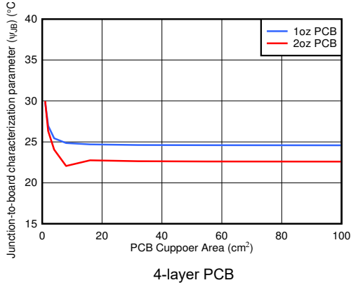
10-3. Junction-to-Board Characterization Parameter ( \psi_{JB} ) vs PCB Copper Area (DRB Package)
