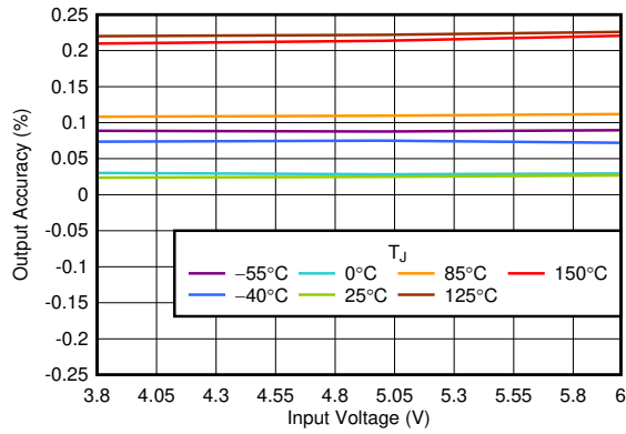
6-1. Output Accuracy vs V_{IN}
