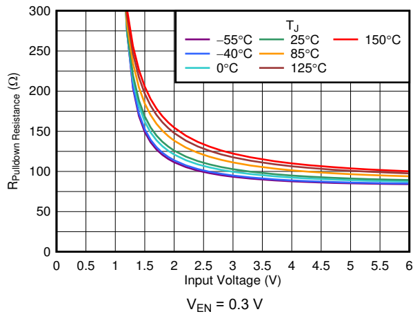
6-13. Pulldown Resistor ( R_{\text{Pulldown}} ) vs V_{\text{IN}}
