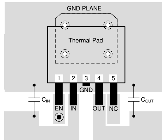
10-8. Layout Example for the DRB Package Fixed Version
