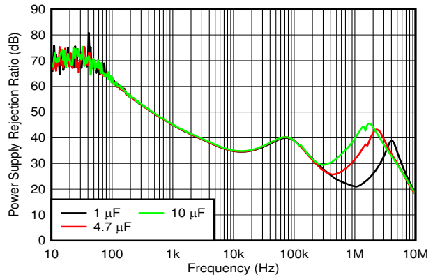
FIG 6-26. PSRR vs C_{OUT}
