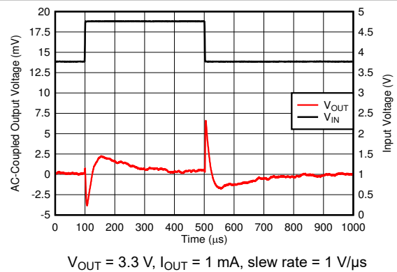
6-16. Line Transient
