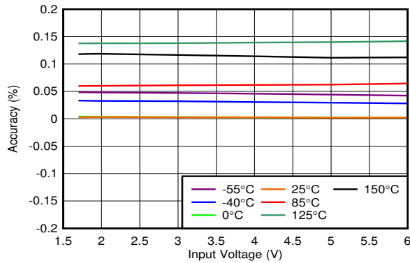
6-1. Output Accuracy vs V_{IN}
