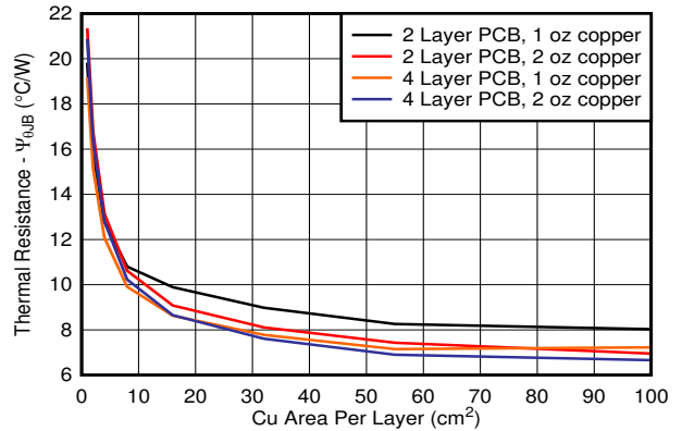
10-6. Junction-to-Board Characterization Parameter ( \psi_{JB} ) vs PCB Copper Area (KVU Package)
