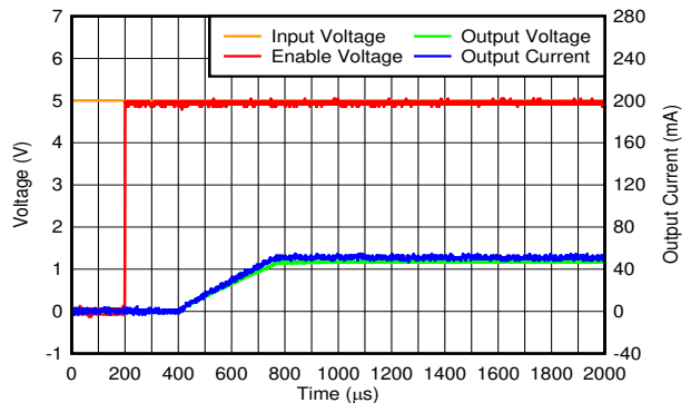
FIG 6-28. Start-Up Inrush Current With C_{OUT} = 1\text{ }\mu\text{F}
