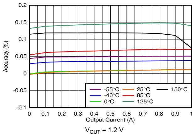
6-5. Output Accuracy vs Output Current
