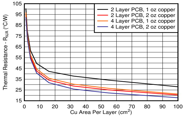
10-5. Junction-to-Ambient Thermal Resistance ( R_{\theta JA} ) vs PCB Copper Area (KVU Package)
