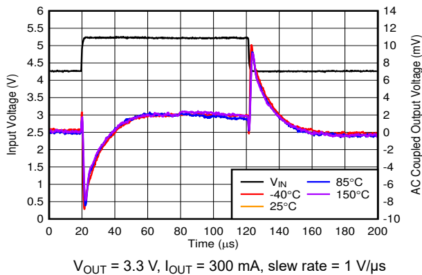
6-17. Line Transient vs Temperature
