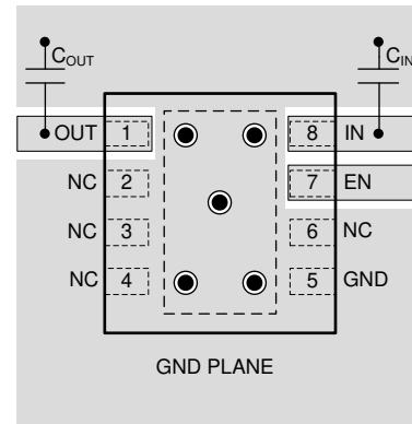
10-8. Layout Example for the DRB Package Fixed Version
