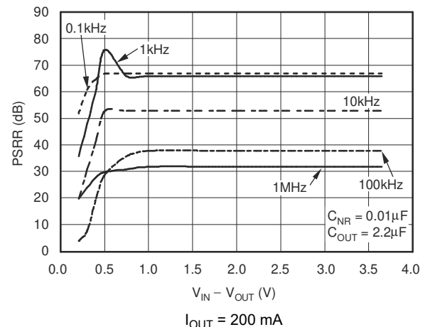
6-18. Power-Supply Ripple Rejection vs V_{IN} - V_{OUT}
