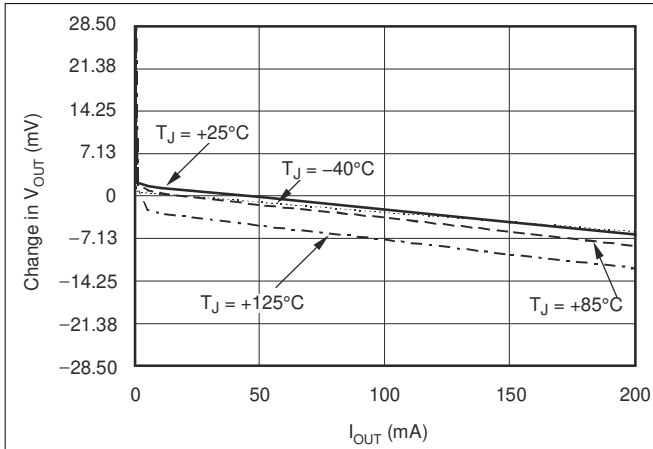
6-1. Load Regulation
