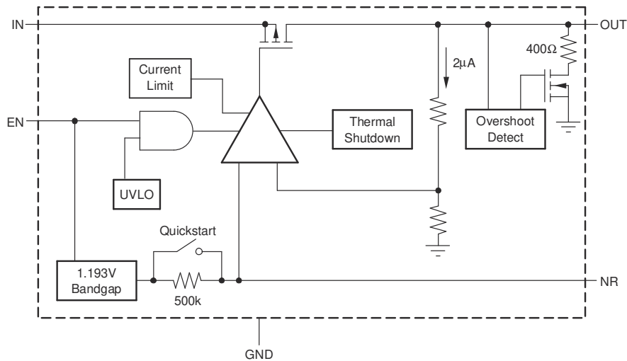
7-1. Fixed-Voltage Versions
