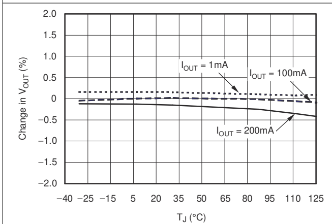
6-1. Load Regulation
