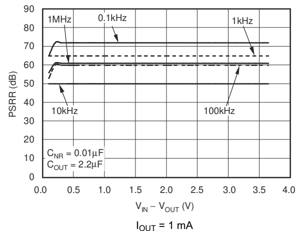
6-16. Power-Supply Ripple Rejection vs V_{IN} - V_{OUT}
