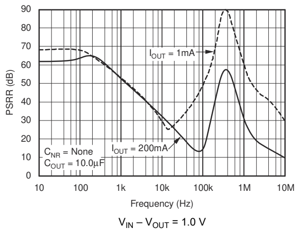
6-15. TPS799285 Power-Supply Ripple Rejection vs Frequency
