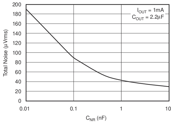
6-19. TPS799285 Total Noise vs C_{NR}
