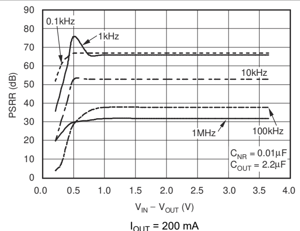
6-18. Power-Supply Ripple Rejection vs V_{IN} - V_{OUT}
