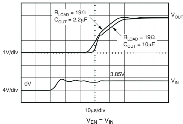
6-23. TPS799285 Turn-On Response
