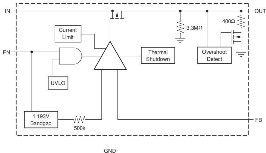
7-2. Adjustable-Voltage Versions
