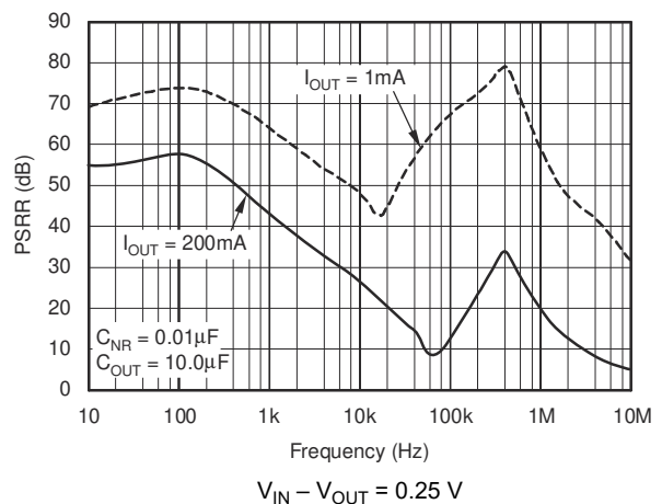
6-14. TPS799285 Power-Supply Ripple Rejection vs Frequency
