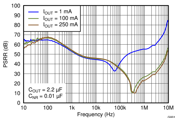
8-3. Power-Supply Rejection Ratio vs Frequency
