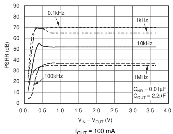
6-17. Power-Supply Ripple Rejection vs V_{IN} - V_{OUT}
