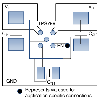
☒ 10-1. Layout Example
