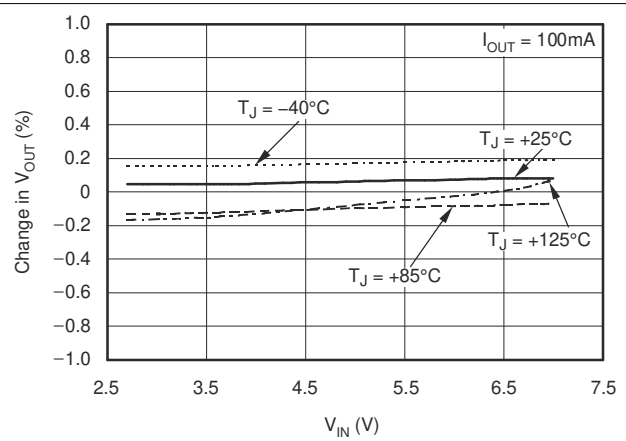
6-2. Line Regulation
