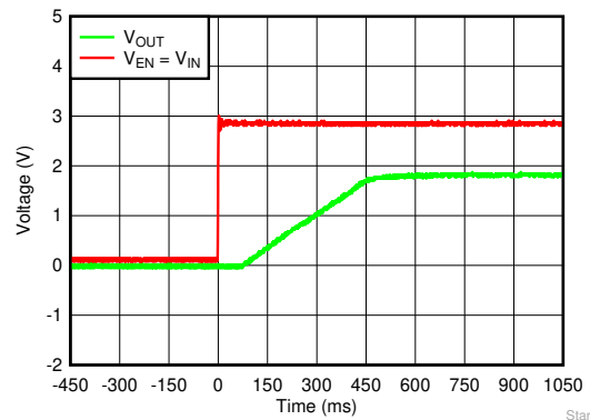
6-50. Startup With V_{EN} = V_{IN}
