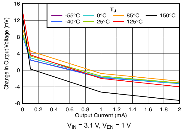
5-4. Load Regulation vs I_{OUT}
