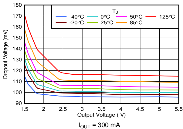
5-17. Dropout Voltage vs V_{OUT}
