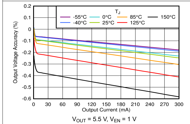
5-9. Output Voltage Accuracy vs I_{OUT}
