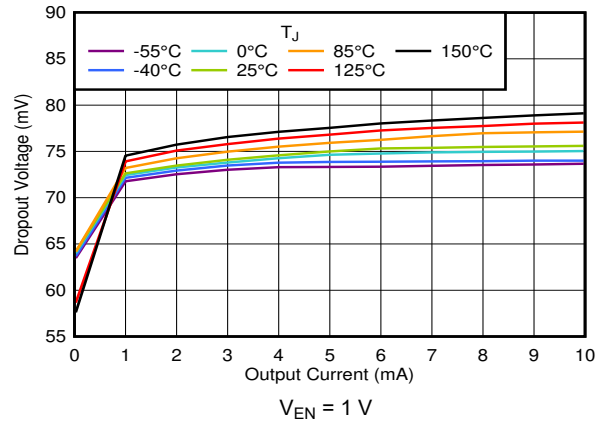
5-14. Dropout Voltage vs I_{OUT}
