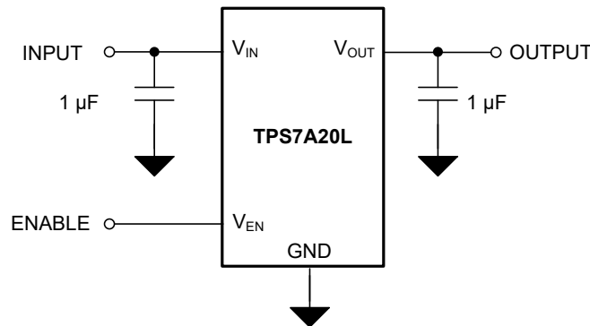
☒ 7-4. TPS7A20L Typical Application
