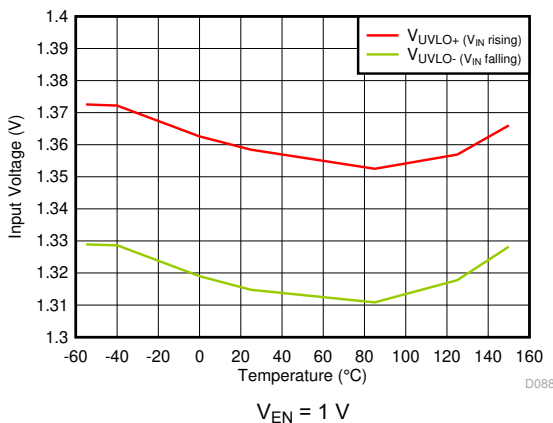
5-29. UVLO Threshold vs Temperature
