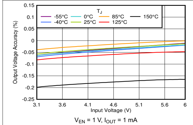
5-11. Output Voltage Accuracy vs V_{IN}
