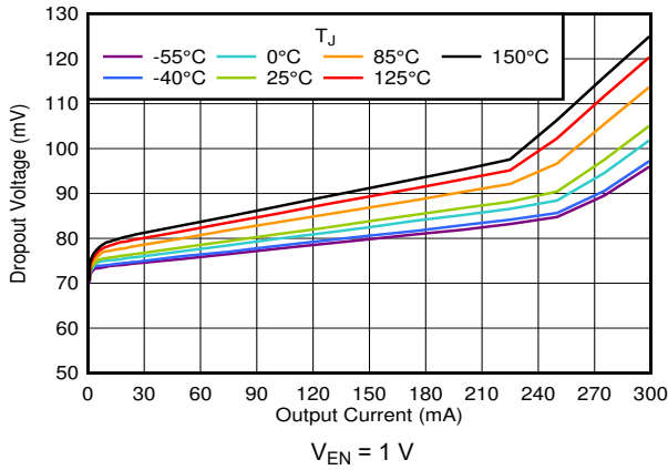
5-13. Dropout Voltage vs I_{OUT}
