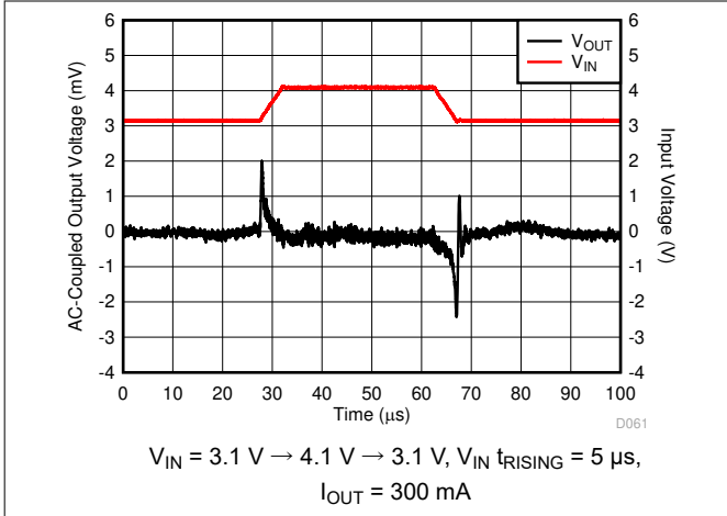
5-43. Line Transient
