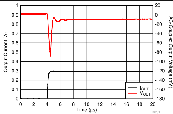
5-36. Load Transient
