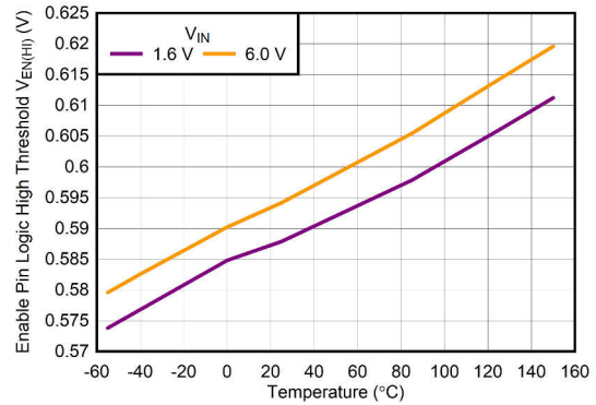
5-30. Enable Logic High Threshold vs Temperature
