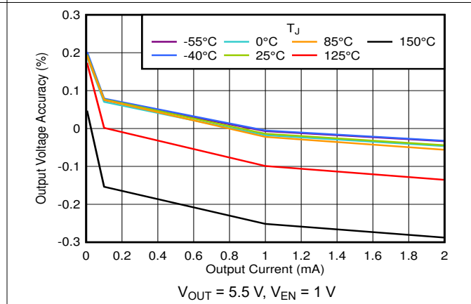
5-10. Output Voltage Accuracy vs I_{OUT}
