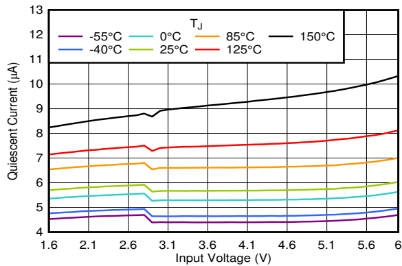
5-19. I_{GND} vs V_{IN}
