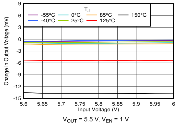
5-2. Line Regulation vs V_{IN}
