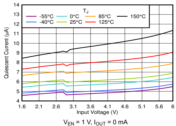
5-18. I_{GND} vs V_{IN}
