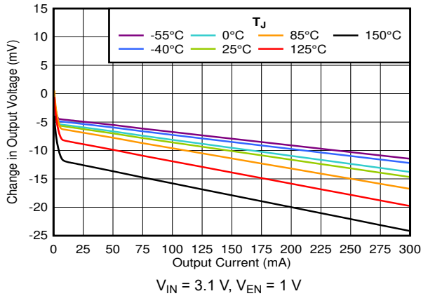
5-3. Load Regulation vs I_{OUT}
