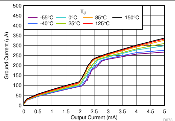
5-22. I_{GND} vs I_{OUT}
