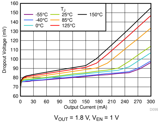
5-15. Dropout Voltage vs I_{OUT}
