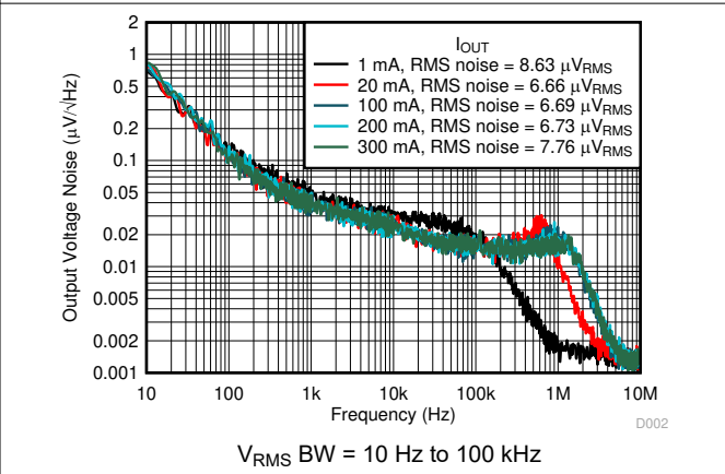
5-48. Noise vs Frequency and I_{OUT}
