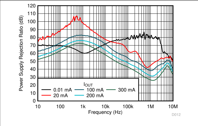
5-46. PSRR vs Frequency and I_{OUT}
