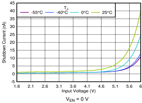
5-25. Shutdown Current vs V_{IN}
