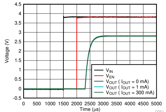
Figure 5-58. Start-Up
