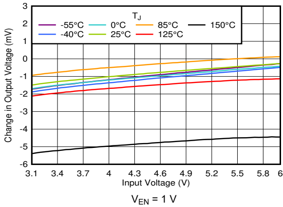
5-1. Line Regulation vs V_{IN}
