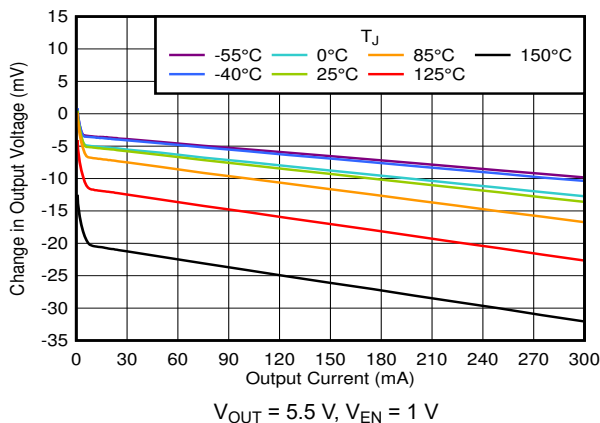
5-5. Load Regulation vs I_{OUT}
