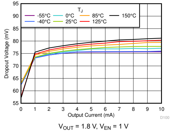
5-16. Dropout Voltage vs I_{OUT}
