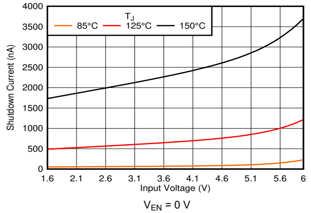
5-26. Shutdown Current vs V_{IN}
