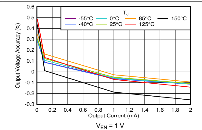
5-8. Output Voltage Accuracy vs I_{OUT}
