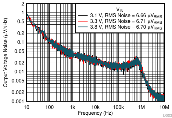
5-49. Noise vs Frequency and V_{IN}
