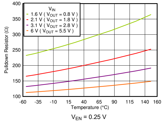
5-32. Output Pulldown Resistor vs Temperature
