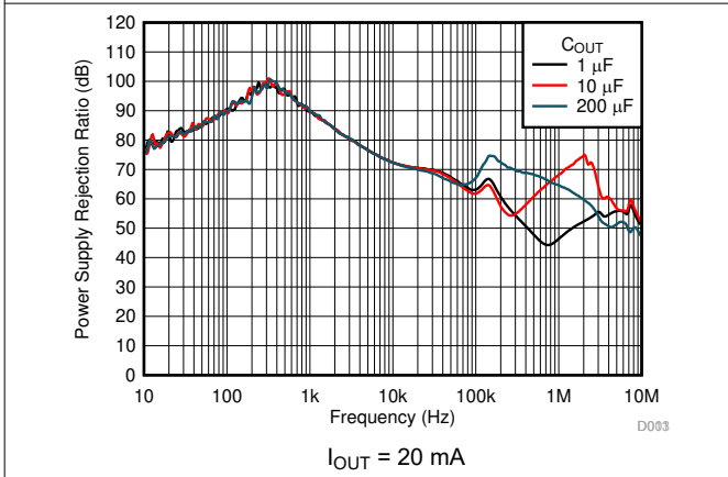
5-47. PSRR vs Frequency and C_{OUT}
