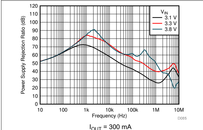
5-45. PSRR vs Frequency and V_{IN}
