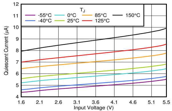
5-20. I_{GND} vs V_{IN} in the Dropout Region
