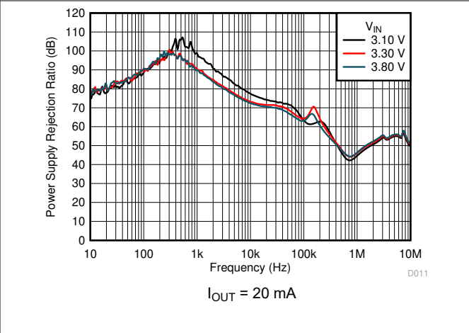
5-44. PSRR vs V_{IN} vs Frequency and V_{IN}
