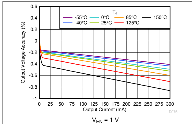
5-7. Output Voltage Accuracy vs I_{OUT}
