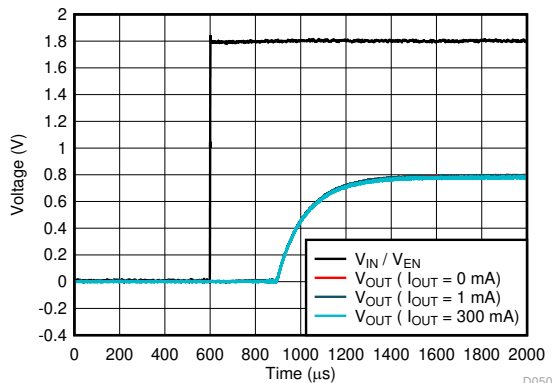
Figure 5-57. Start-Up
