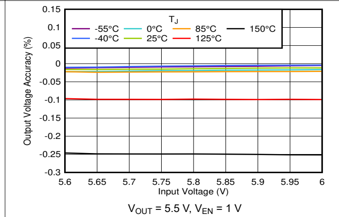
5-12. Output Voltage Accuracy vs V_{IN}
