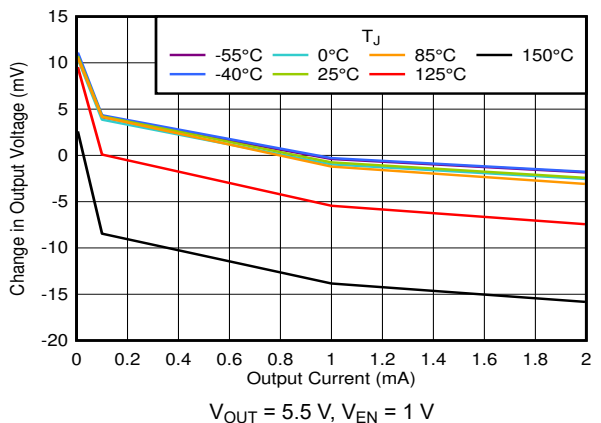
5-6. Load Regulation vs I_{OUT}
