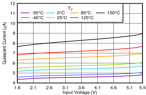
5-19. I_{GND} vs V_{IN}
