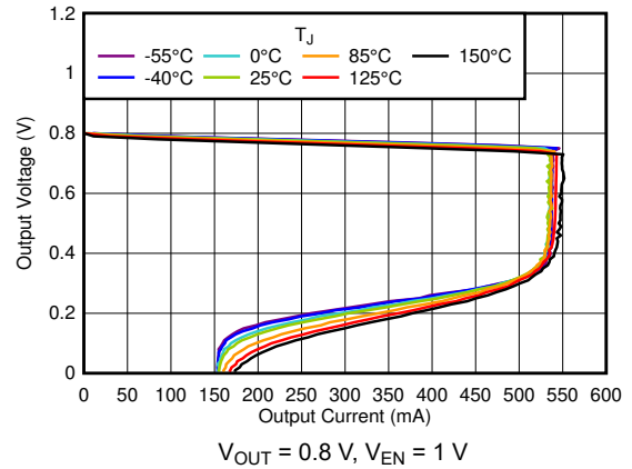
5-28. Current Limit
