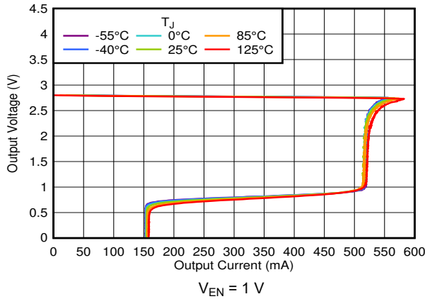
5-27. Current Limit
