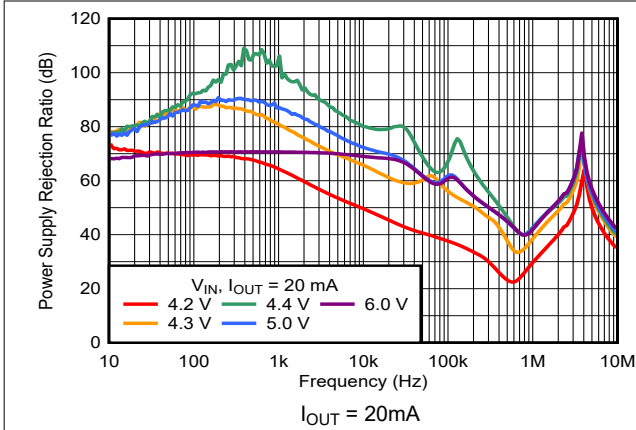
5-25. PSRR vs Frequency and V_{IN}
