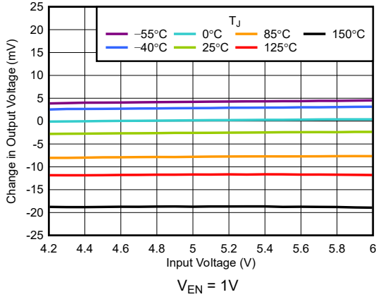
图 5-1. Line Regulation vs V_{IN}
