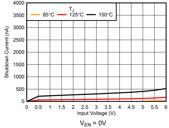
5-14. Shutdown Current vs V_{IN}
