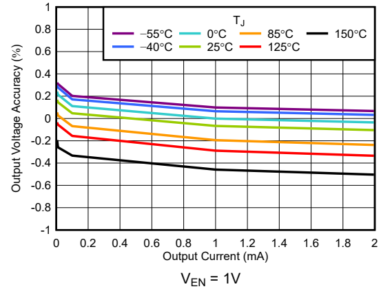
图 5-4. Output Voltage Accuracy vs I_{OUT}
