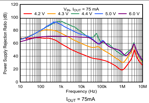
5-26. PSRR vs Frequency and V_{IN}
