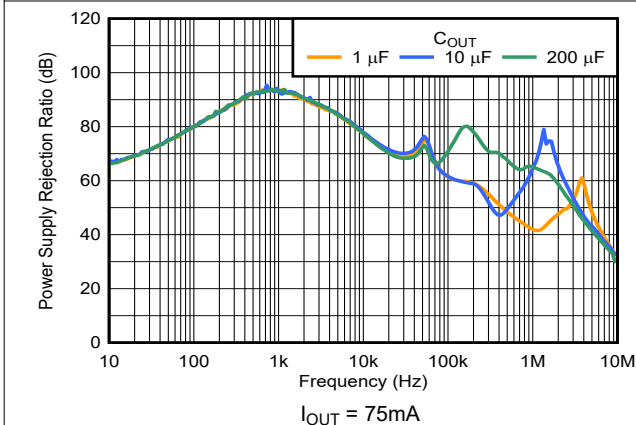
5-29. PSRR vs Frequency and C_{OUT}
