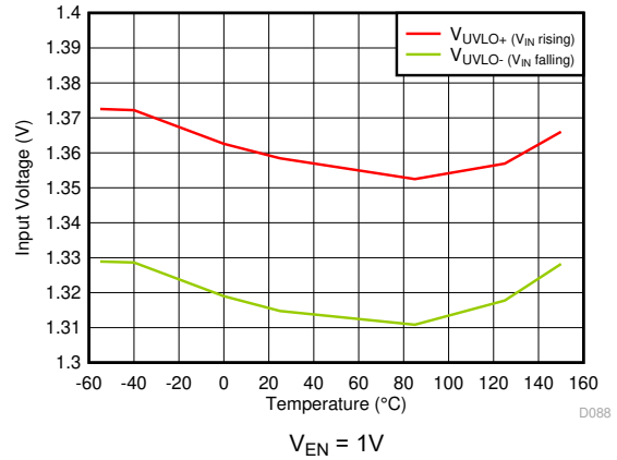
5-16. UVLO Threshold vs Temperature
