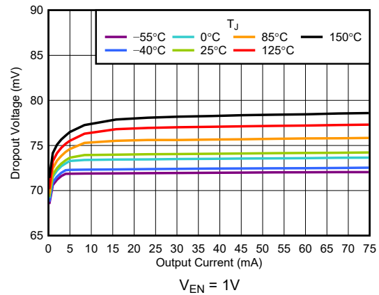
5-8. Dropout Voltage vs I_{OUT}
