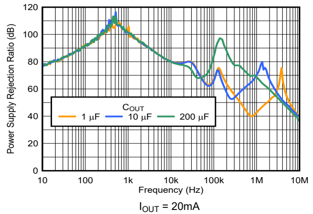
5-28. PSRR vs Frequency and C_{OUT}
