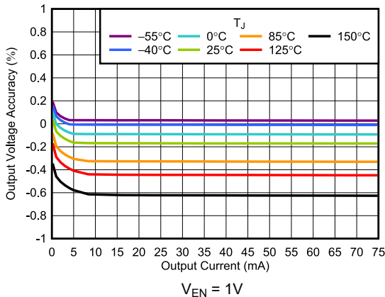
图 5-5. Output Voltage Accuracy vs I_{OUT}
