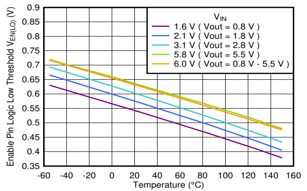
5-18. Enable Logic Low Threshold vs Temperature
