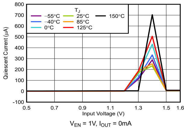
5-9. I_{GND} vs V_{IN}
