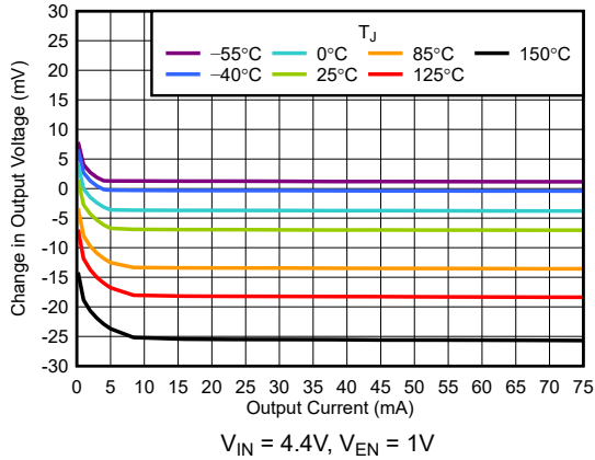
图 5-3. Load Regulation vs I_{OUT}
