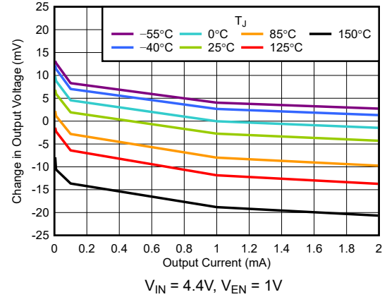
图 5-2. Load Regulation vs I_{OUT}
