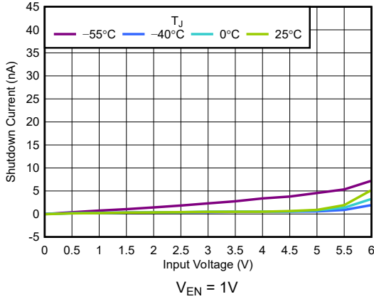
5-13. Shutdown Current vs V_{IN}
