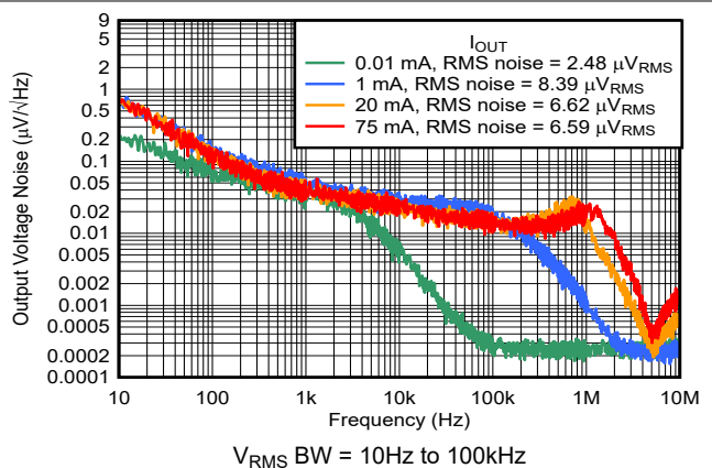
5-30. Noise vs Frequency and I_{OUT}
