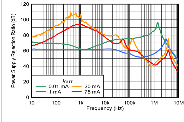
5-27. PSRR vs Frequency and I_{OUT}
