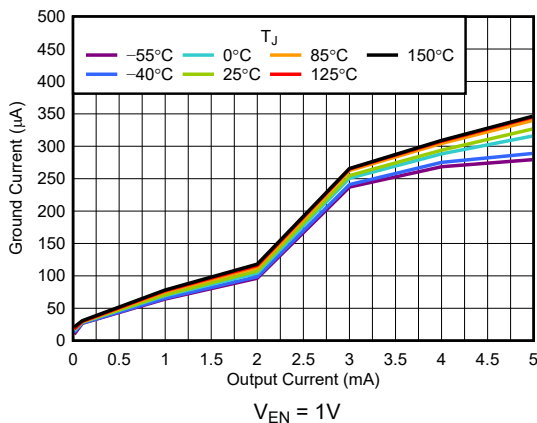
5-11. I_{GND} vs I_{OUT}
