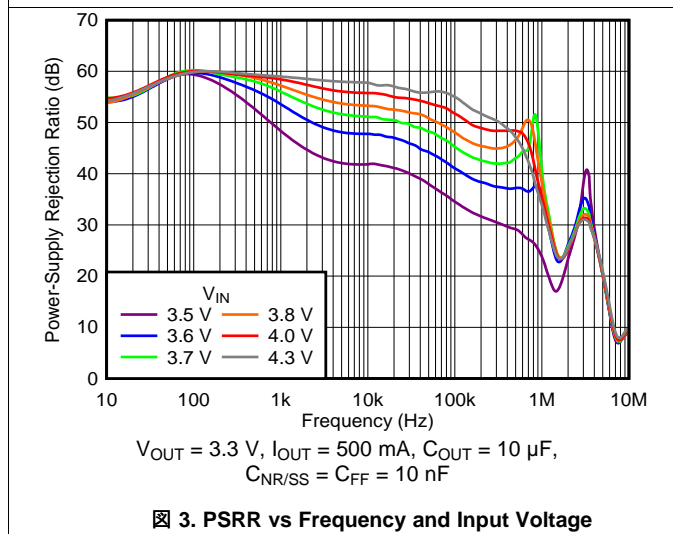
Fig. 1. PSRR vs Frequency and Input Voltage
