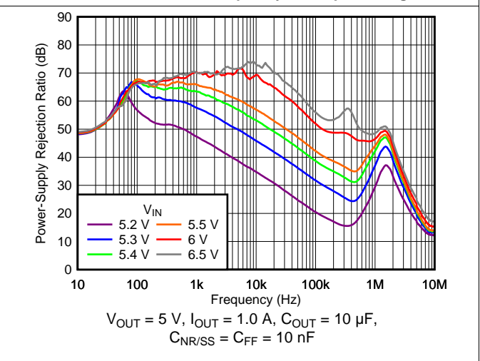
Fig. 4. PSRR vs Frequency and Input Voltage
