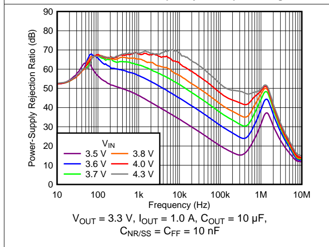
Fig. 3. PSRR vs Frequency and Input Voltage
