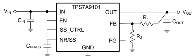
Figure 38. Adjustable Operation
