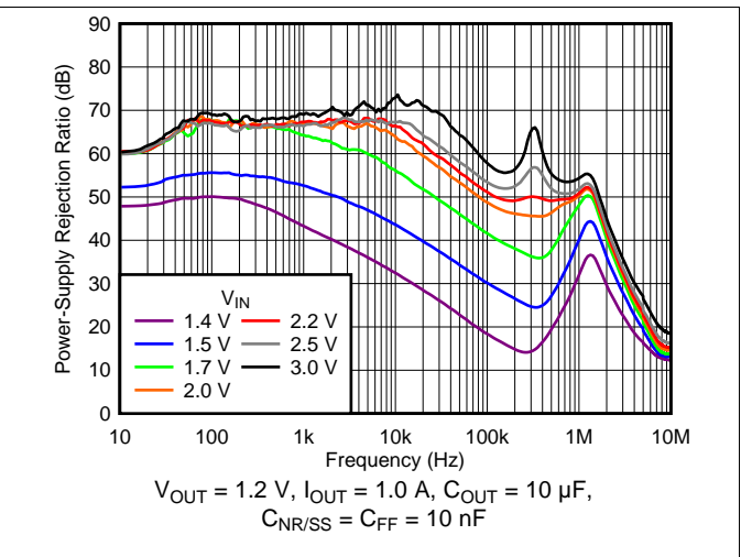
Fig. 2. PSRR vs Frequency and Input Voltage
