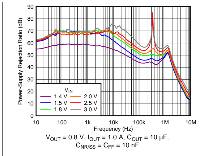
Fig. 1. PSRR vs Frequency and Input Voltage
