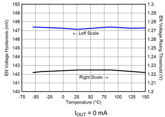
6-64. V_{EN} Hysteresis and Threshold vs Temperature
