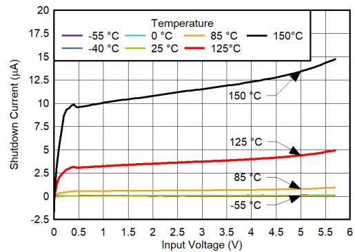
6-72. Shutdown Current vs V_{IN} and Temperature
