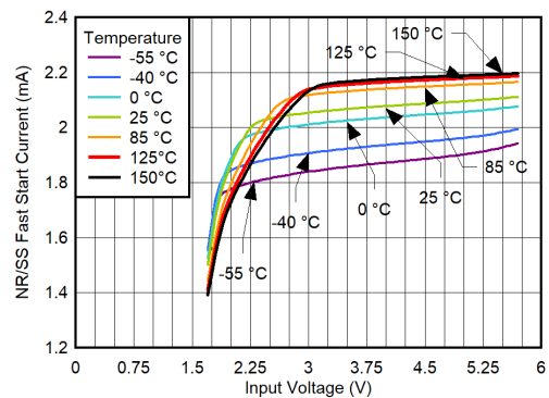
8-12. I_{FAST\_SS} Reference vs Input Voltage and Temperature for V_{OUT} = 3.3 V
