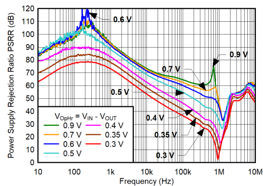
6-6. PSRR vs Frequency for Operating Headroom ( V_{OpHr} )
