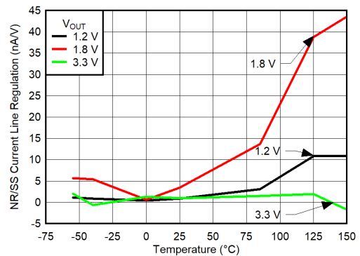
6-36. I_{NR/SS} Line Regulation
