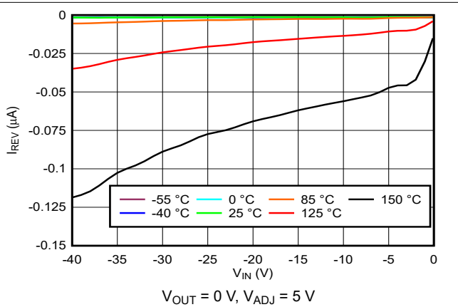
6-16. Reverse Current vs. Input Voltage
