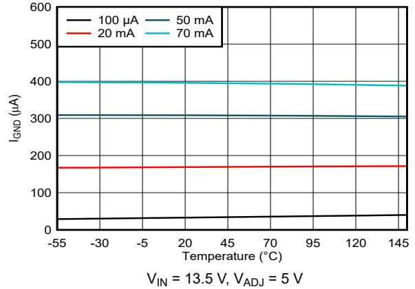
6-10. Ground Current vs Ambient Temperature
