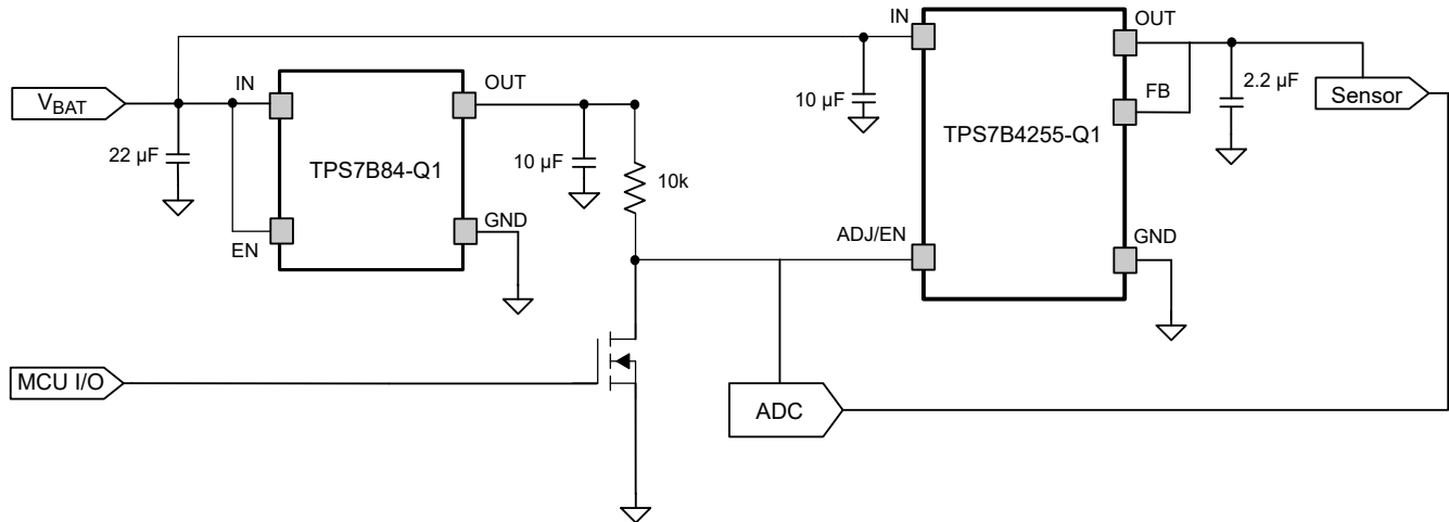
Figure 7-7. Tracking an LDO With an Enable Circuit
