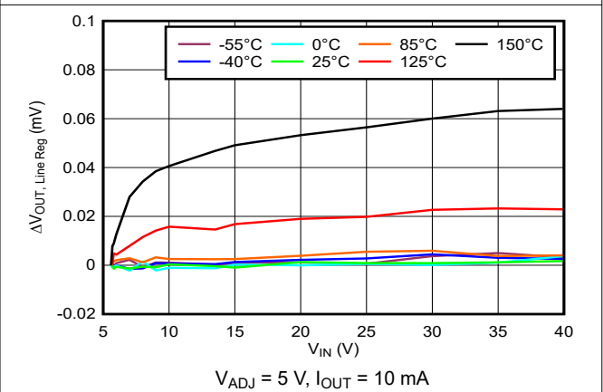
6-4. Line Regulation
