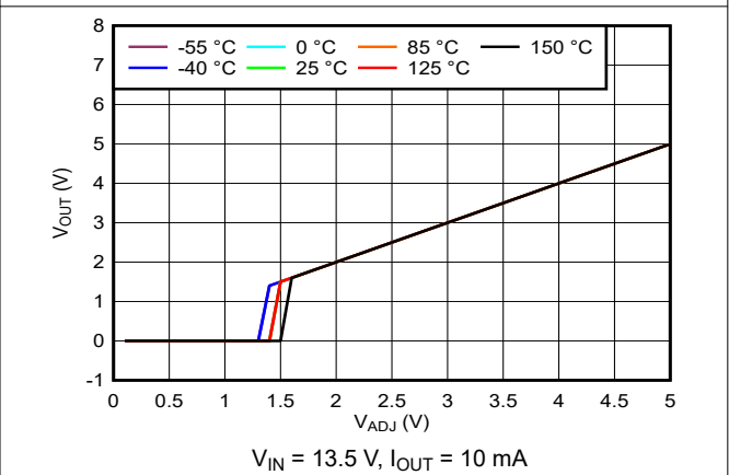
6-6. Output Voltage vs Adjustable Reference Voltage
