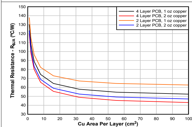
Figure 8-8. R_{\theta JA} vs Copper Area (DYB Package)
