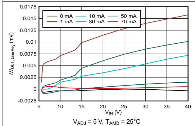
6-3. Line Regulation
