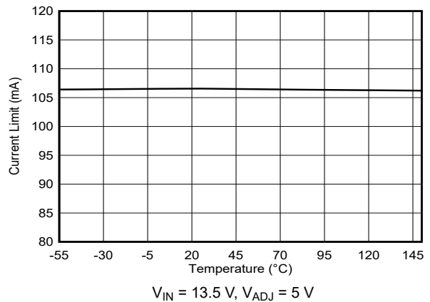
6-12. Current Limit vs Ambient Temperature
