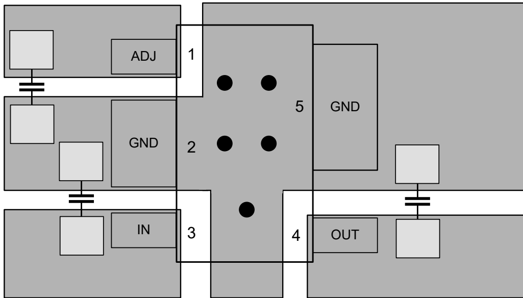
☒ 8-10. DYB Package Layout Example
