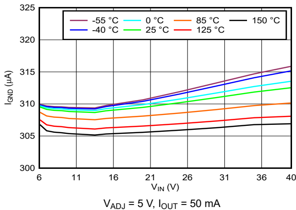
6-11. Ground Current vs Input Voltage
