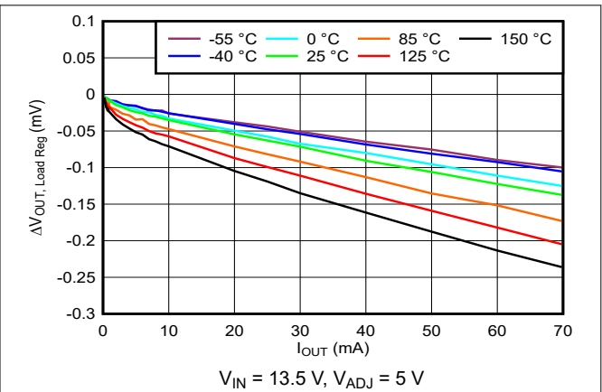
6-2. Load Regulation
