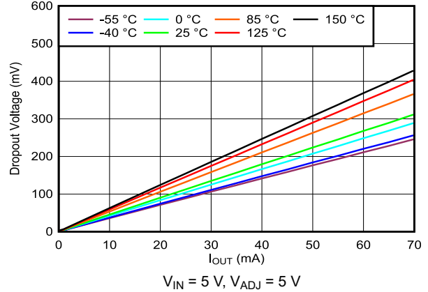
6-8. Dropout Voltage vs Output Current
