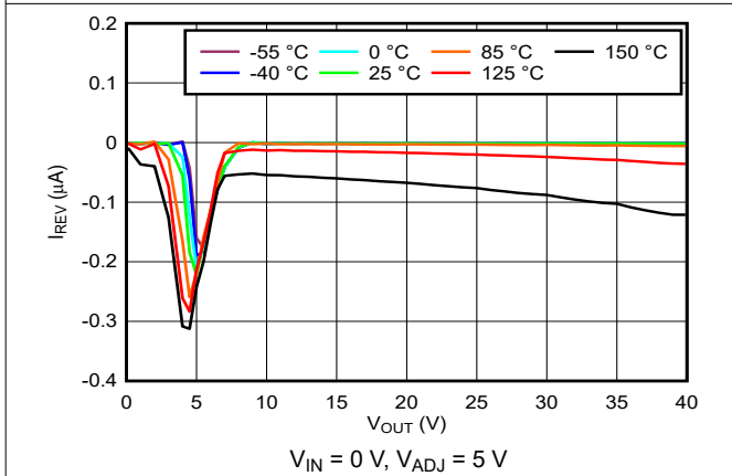
6-15. Reverse Current vs. Output Voltage
