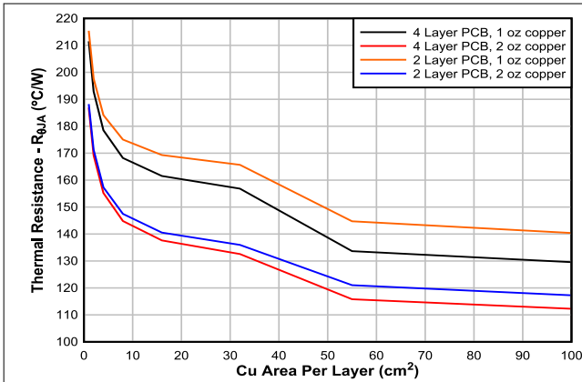
Figure 8-6. R_{\theta JA} vs Copper Area (DBV Package)
