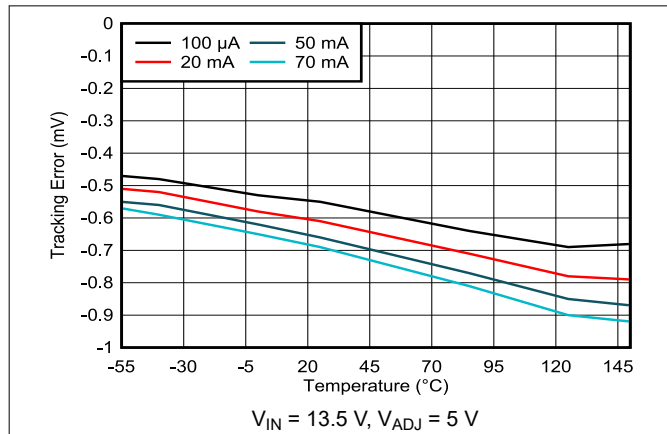
6-1. Tracking Error vs Ambient Temperature
