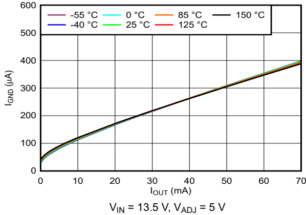
6-9. Ground Current vs Output Current
