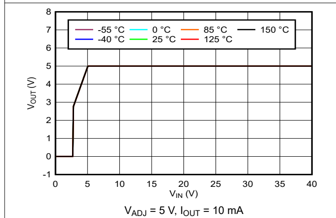
6-5. Output Voltage vs Input Voltage
