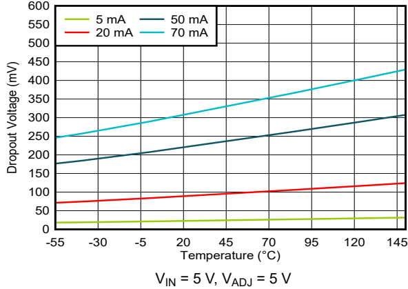
6-7. Dropout Voltage vs Ambient Temperature
