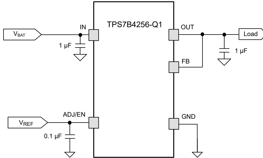
図 6-2. Tracker Output Voltage equal to Reference Voltage
