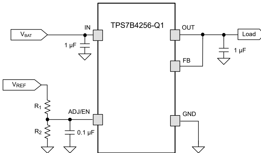
図 6-3. Tracker Output Voltage Lower Than the Reference Voltage
