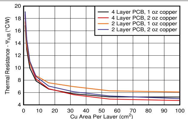
8-5. \psi_{JB} vs Copper Area (KVU Package)
