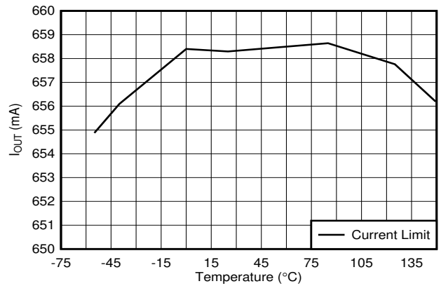
6-26. Output Current Limit vs Temperature
