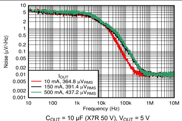
6-12. Noise vs Frequency
