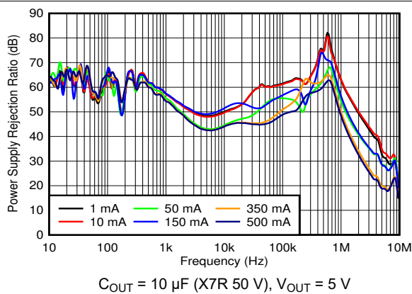
6-11. PSRR vs Frequency and I_{OUT}
