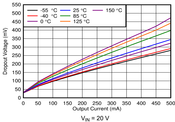
6-9. Dropout Voltage ( V_{DO} ) vs I_{OUT}
