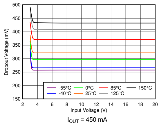
6-10. Dropout Voltage ( V_{DO} ) vs V_{IN}
