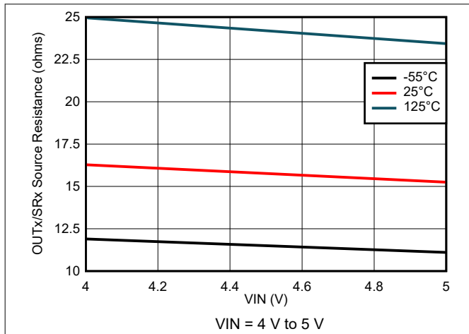
8-61. Output Source Resistance Variation
