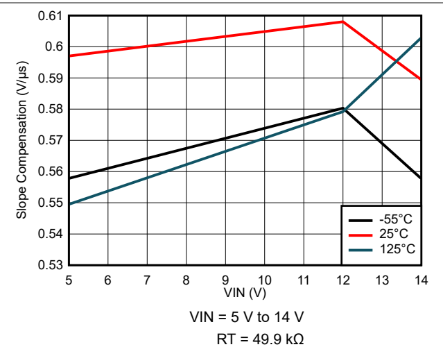
8-72. Slope Compensation Variation
