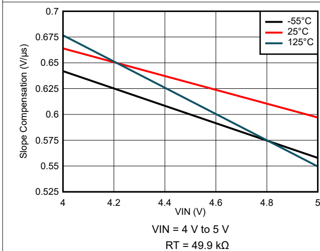
8-71. Slope Compensation Variation
