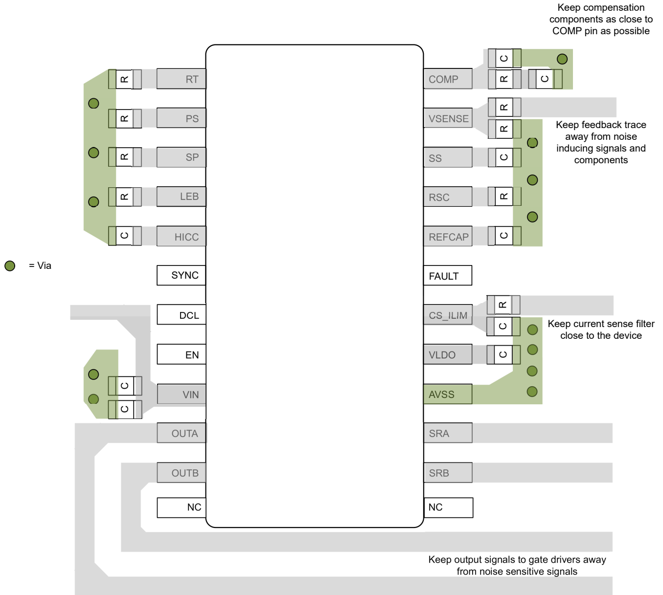
10-5. PCB Layout Example for TSSOP Package
