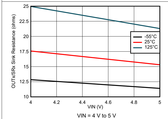
8-63. Output Sink Resistance Variation
