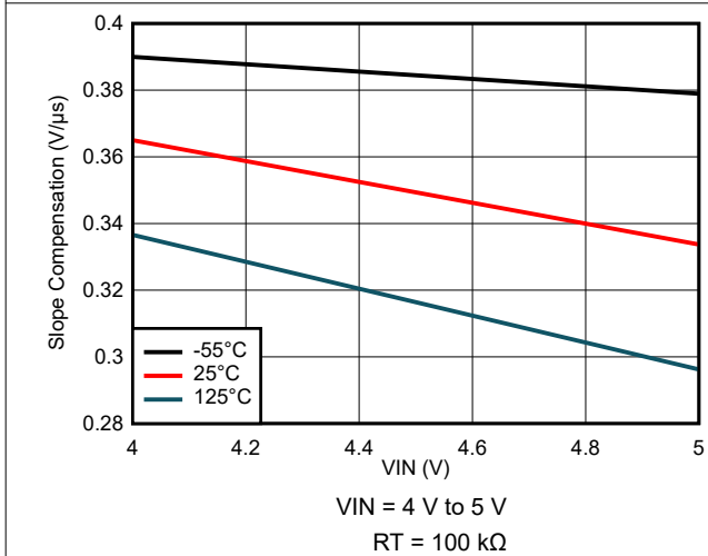
8-69. Slope Compensation Variation
