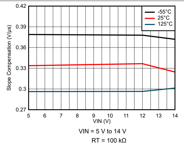
8-70. Slope Compensation Variation
