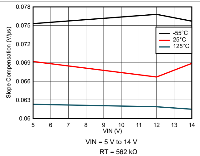
8-68. Slope Compensation Variation
