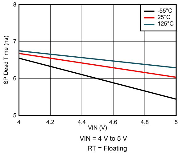
8-49. SP Dead Time Variation
