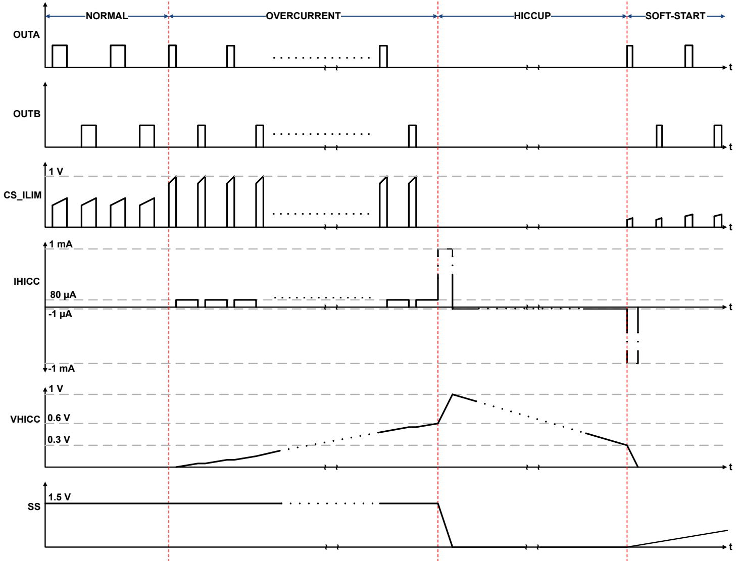
9-15. Cycle-by-Cycle Current Limit Delay Timer and Hiccup Restart Timer
