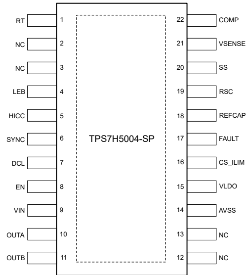
7-4. TPS7H5004-SP HFT Package 22-Pin CFP With Thermal Pad (Top View)
