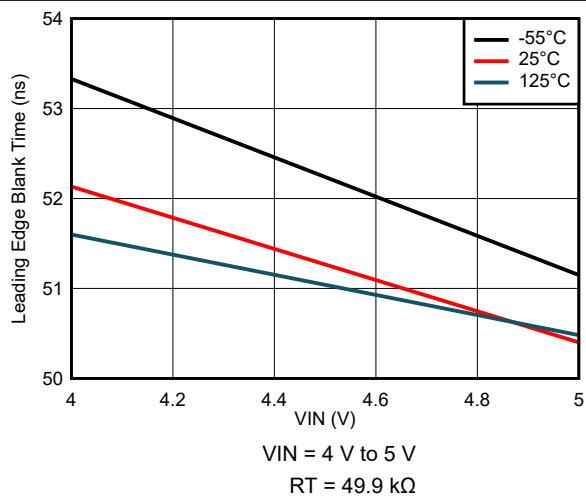
8-35. Leading Edge Blank Time Variation
