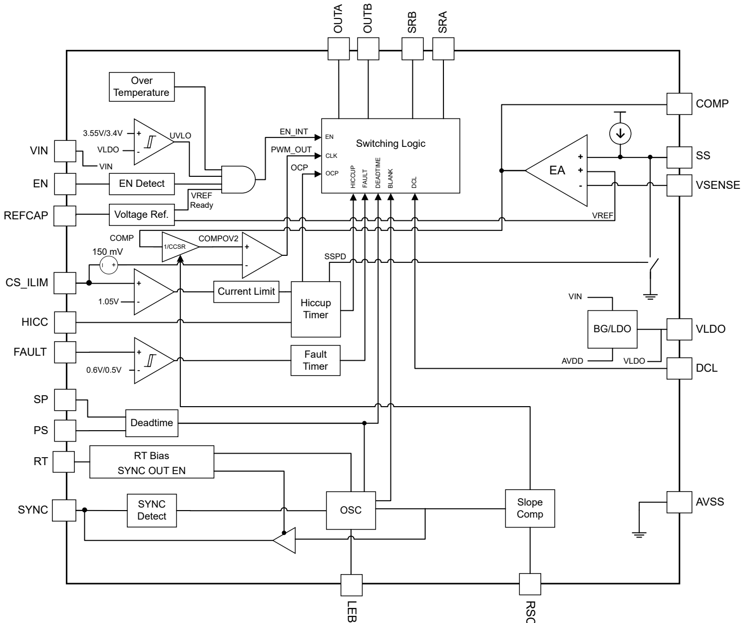
9-1. TPS7H5001-SP Functional Block Diagram
