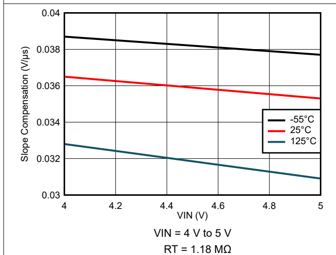
8-65. Slope Compensation Variation
