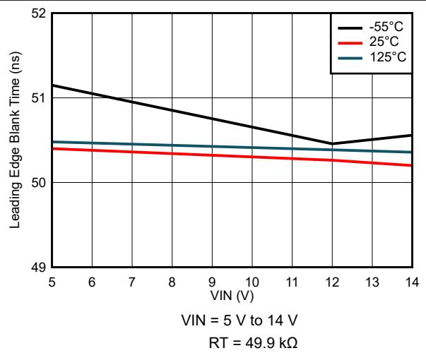
8-36. Leading Edge Blank Time Variation
