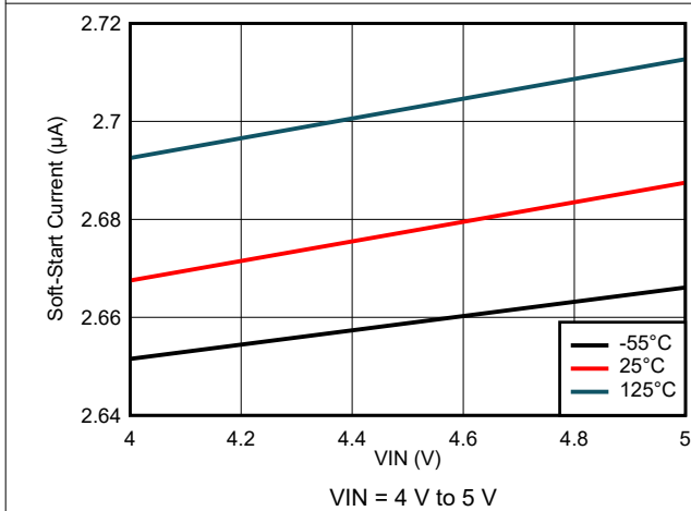
8-9. Soft-Start Current Variation
