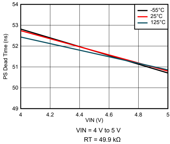
8-43. PS Dead Time Variation
