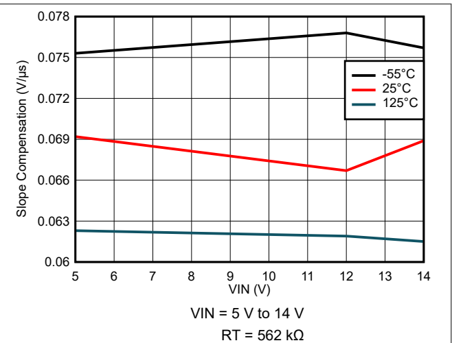
8-68. Slope Compensation Variation
