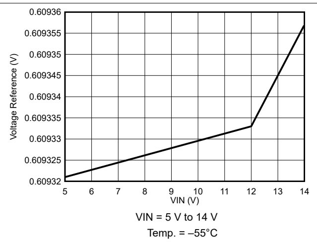
8-12. Voltage Reference Variation
