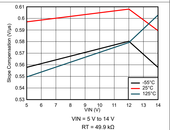
8-72. Slope Compensation Variation
