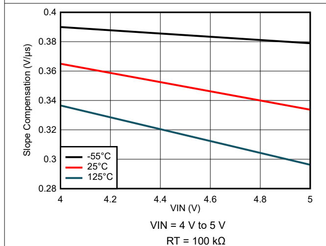
8-69. Slope Compensation Variation
