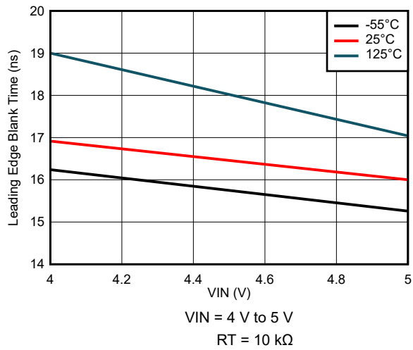
8-33. Leading Edge Blank Time Variation
