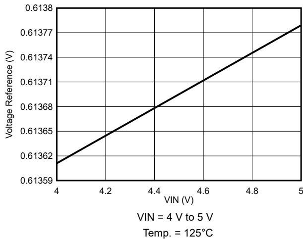
8-15. Voltage Reference Variation
