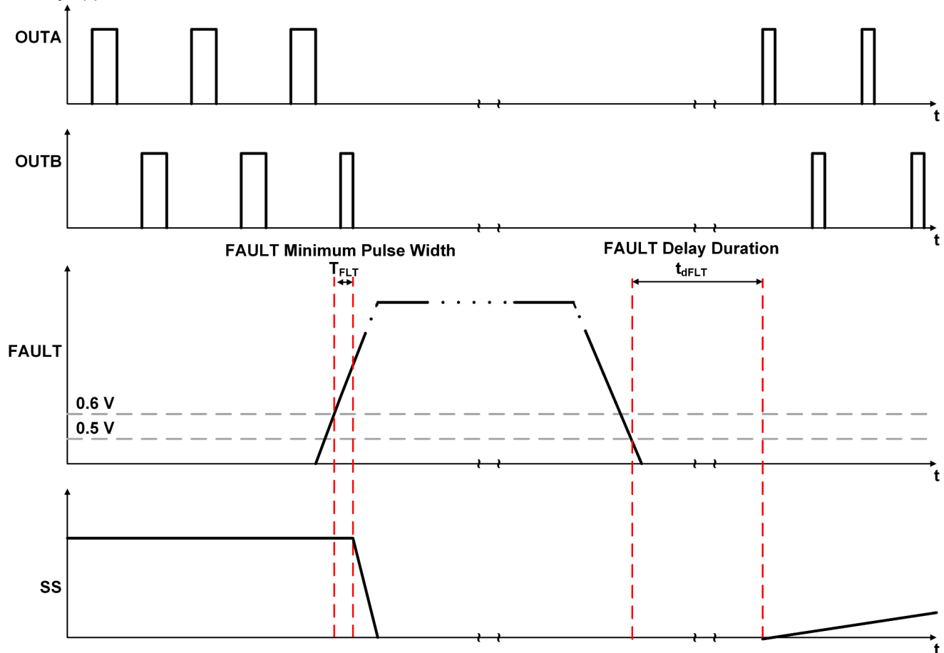
Figure 9-16. Switching Waveforms During Fault Mode
