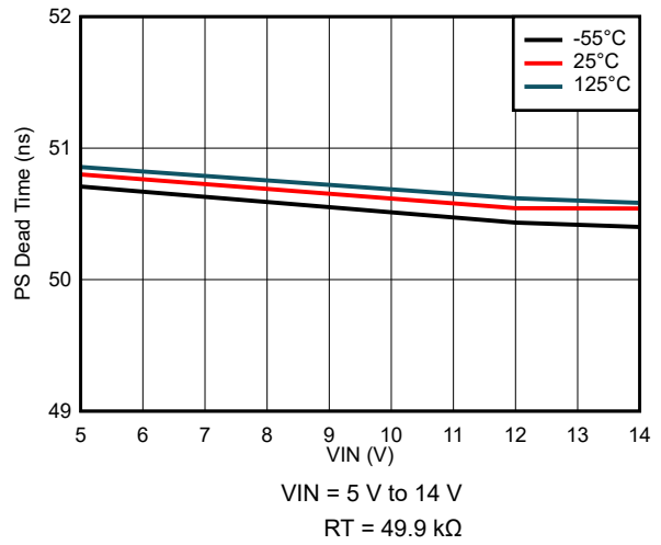
8-44. PS Dead Time Variation
