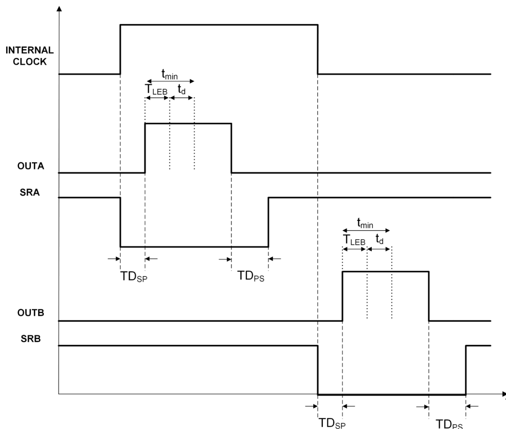
9-13. Outputs Timing Waveforms
