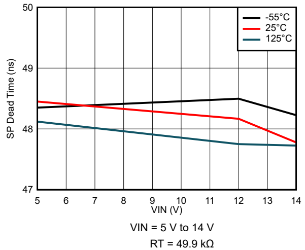
8-52. SP Dead Time Variation
