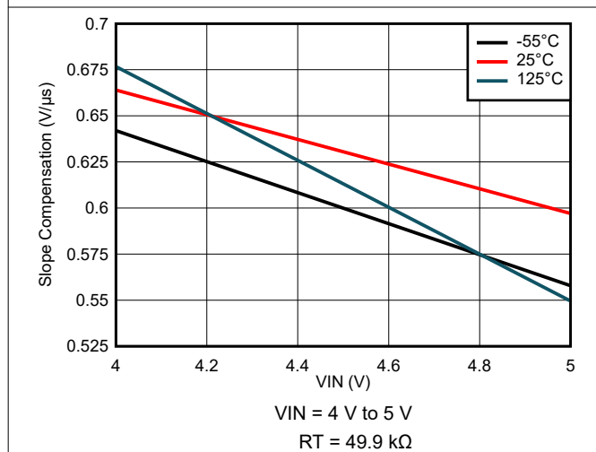
8-71. Slope Compensation Variation
