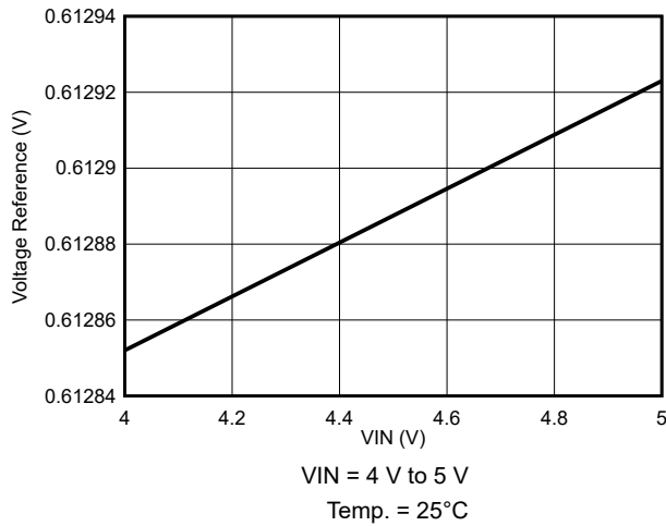
8-13. Voltage Reference Variation
