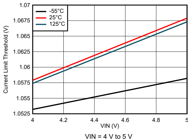
8-17. Current Limit Threshold Variation
