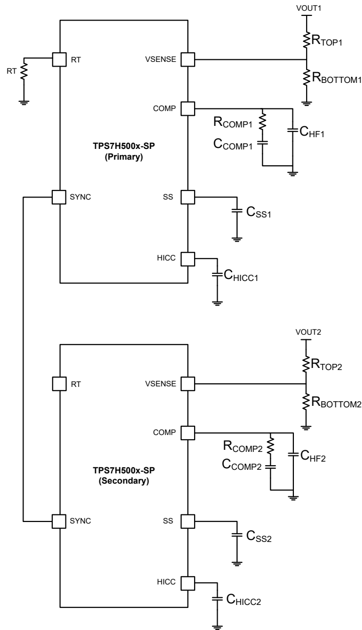
9-10. Primary-Secondary Mode Configuration for Two Independent Converters
