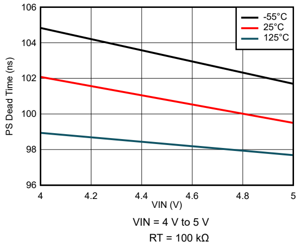
8-45. PS Dead Time Variation
