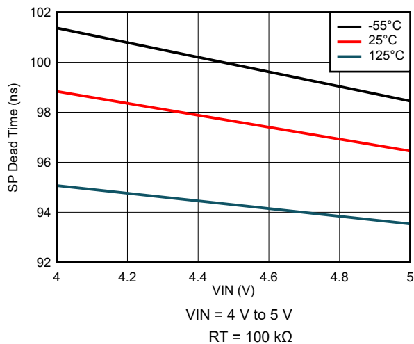
8-53. SP Dead Time Variation
