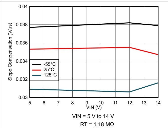
8-66. Slope Compensation Variation
