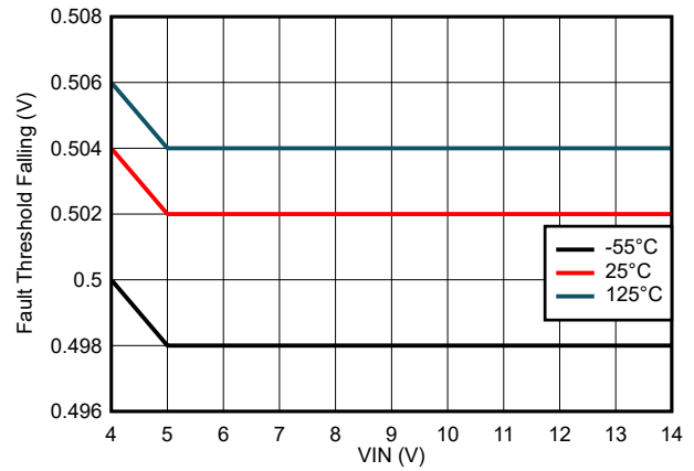
8-32. FAULT Threshold Falling Variation
