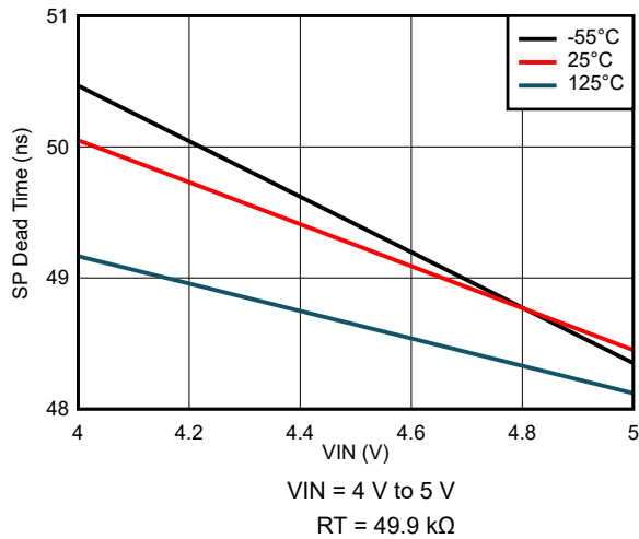
8-51. SP Dead Time Variation
