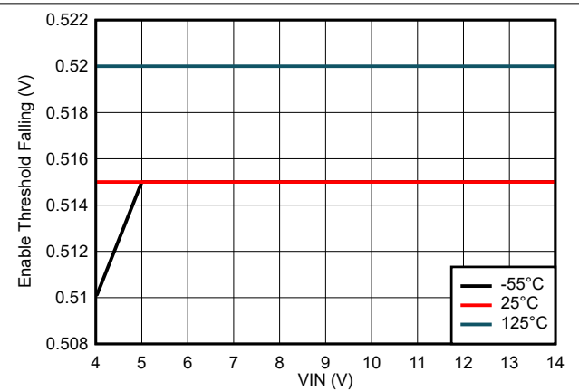
8-8. Enable Threshold Falling Variation
