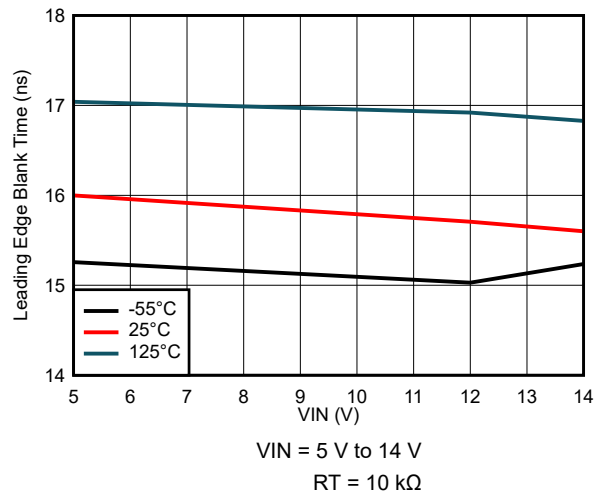
8-34. Leading Edge Blank Time Variation
