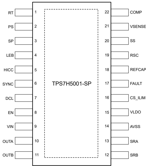
7-1. TPS7H5001-SP HFT Package 22-Pin CFP With Thermal Pad (Top View)
