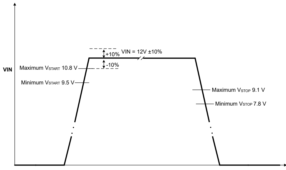
Figure 9-6. Start-Up and UVLO Values for Two-Resistor Configuration With V_{IN} = 12\text{ V}
