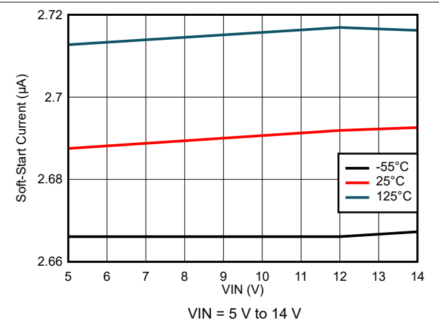
8-10. Soft-Start Current Variation
