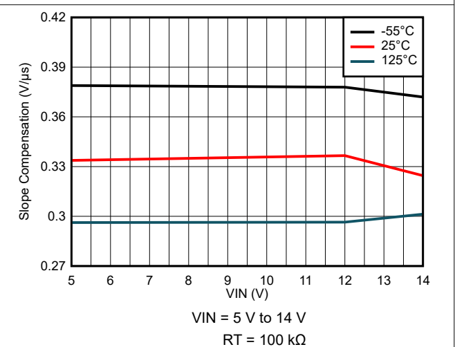
8-70. Slope Compensation Variation
