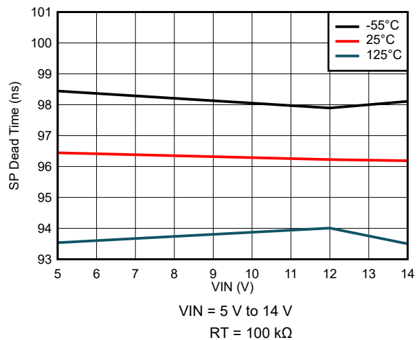
8-54. SP Dead Time Variation
