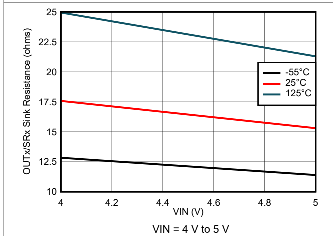
8-63. Output Sink Resistance Variation
