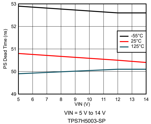
8-48. PS Dead Time Variation
