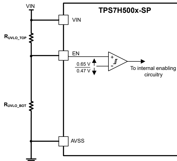
Figure 9-5. Enable Pin Configuration Using Two External Resistors
