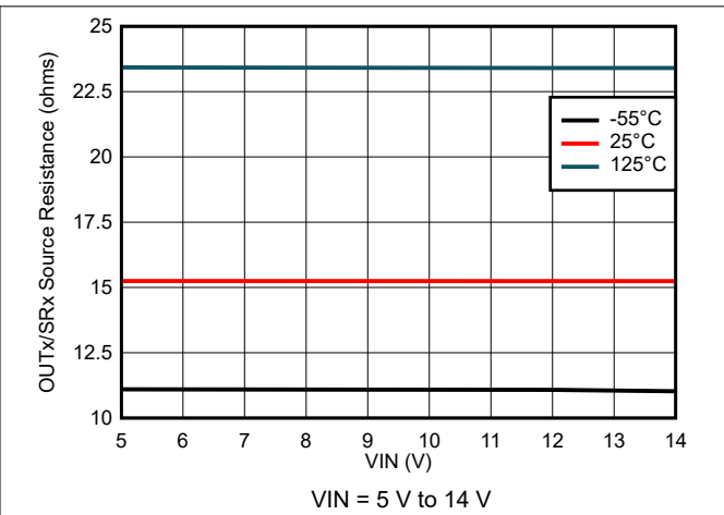
8-62. Output Source Resistance Variation
