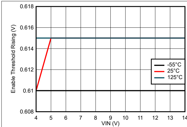
8-7. Enable Threshold Rising Variation
