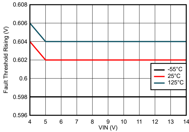
8-31. FAULT Threshold Rising Variation
