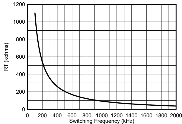
Figure 9-7. RT vs Switching Frequency
