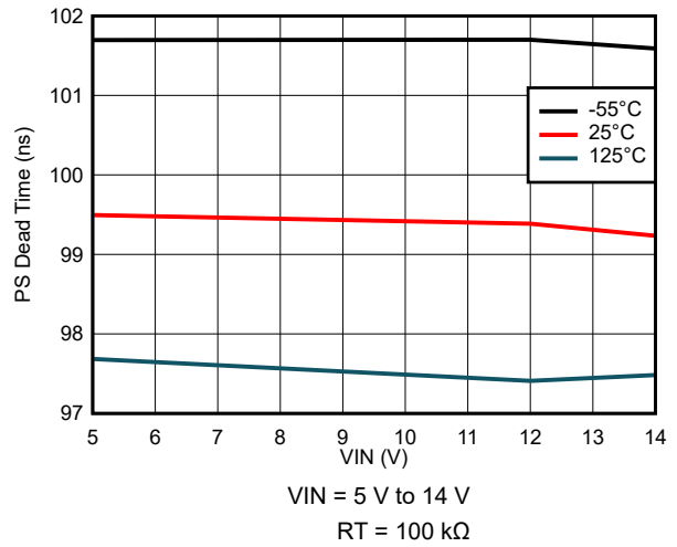
8-46. PS Dead Time Variation
