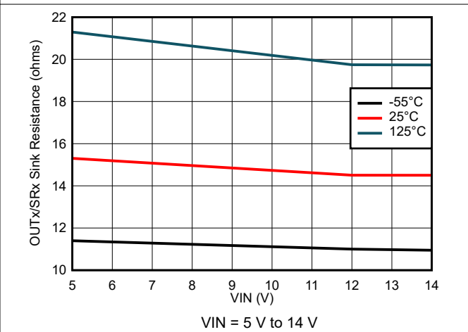
8-64. Output Sink Resistance Variation
