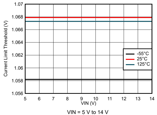
8-18. Current Limit Threshold Variation
