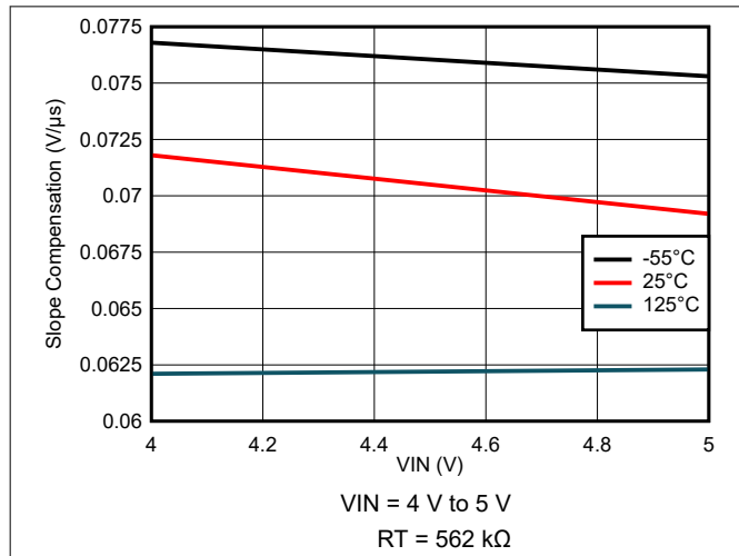
8-67. Slope Compensation Variation
