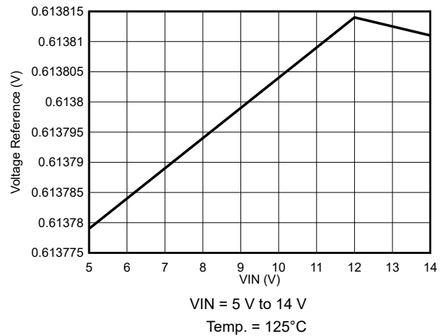
8-16. Voltage Reference Variation
