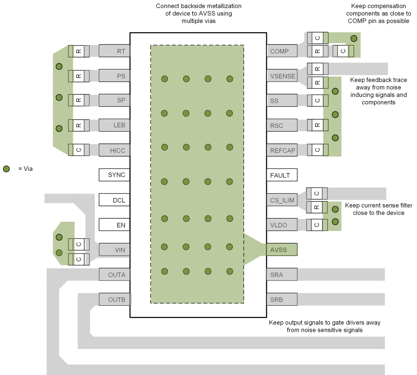
FIG 10-4. PCB Layout Example for CFP Package
