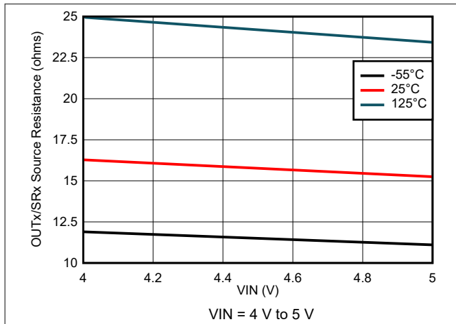
8-61. Output Source Resistance Variation
