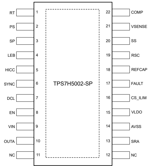
7-2. TPS7H5002-SP HFT Package 22-Pin CFP With Thermal Pad (Top View)
