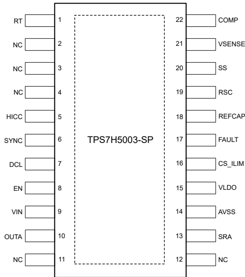
7-3. TPS7H5003-SP HFT Package 22-Pin CFP With Thermal Pad (Top View)
