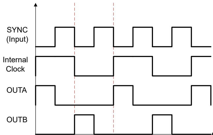
Figure 9-9. Switching Waveforms for External Synchronization Mode
